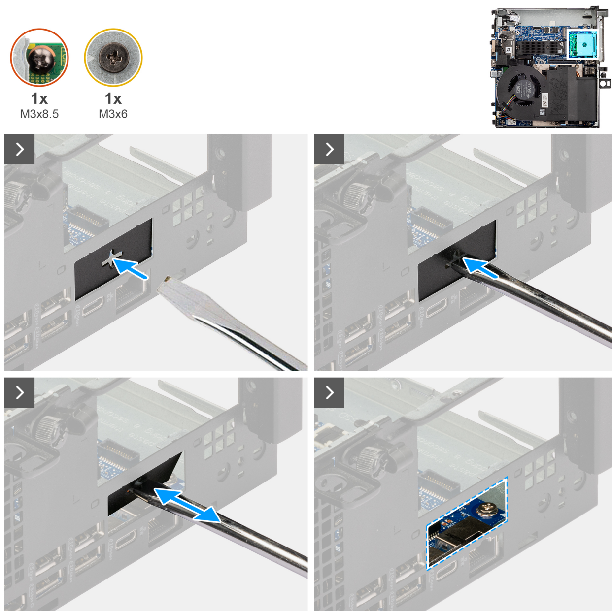
Figure 37. Installation du port DisplayPort
