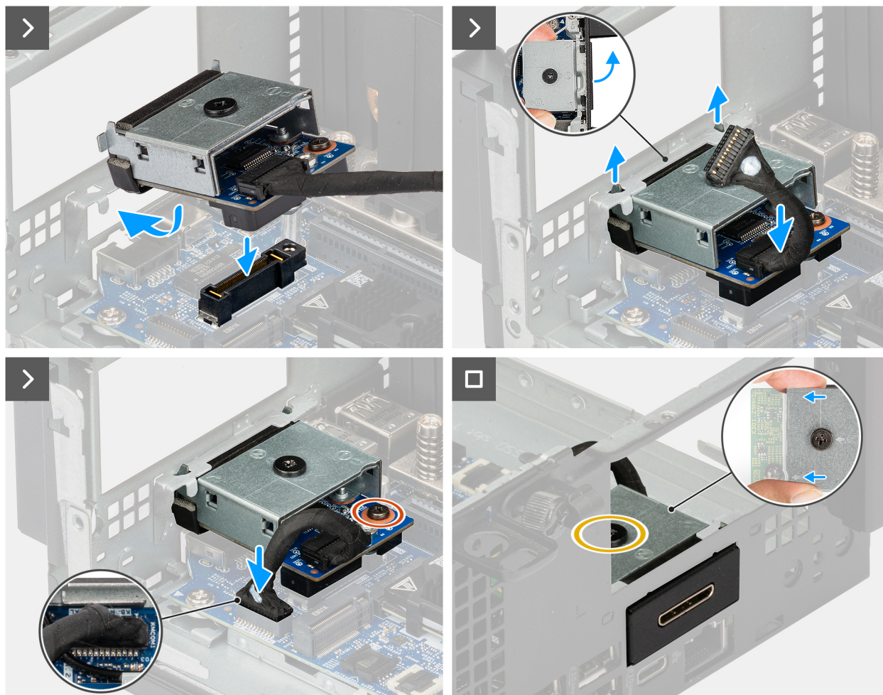
Figure 35. Installation du port PS2
