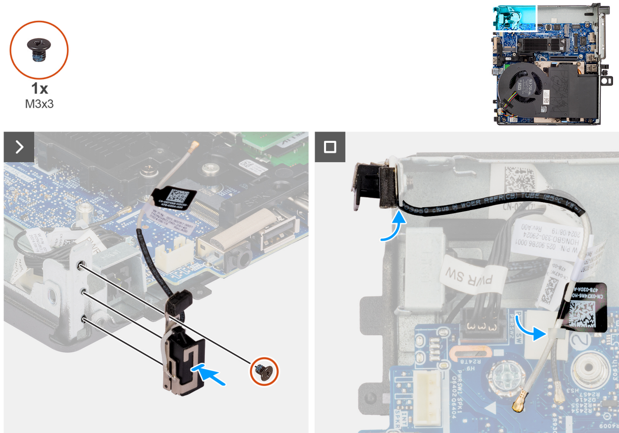
Figure 59. Installation de l'antenne interne (emplacement 1)
