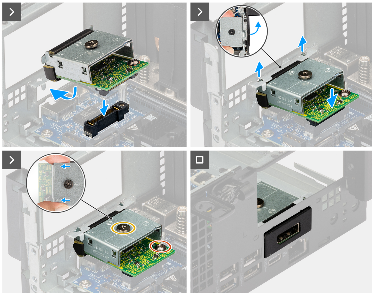
Figure 38. Installation du port DisplayPort
