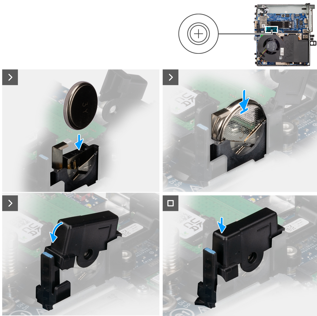
Figure 8. Installation de la pile bouton
