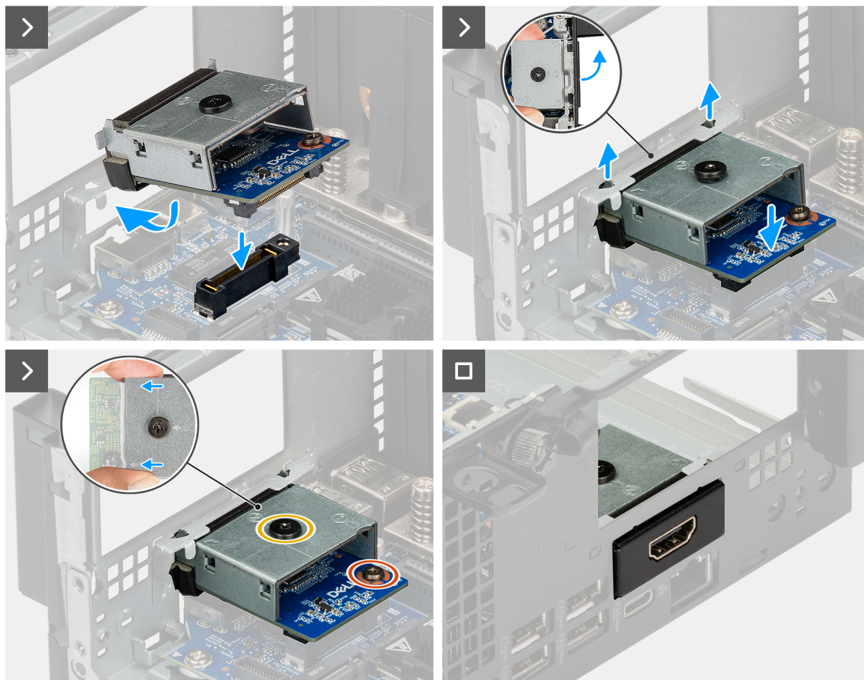
Figure 44. Installation du port HDMI
