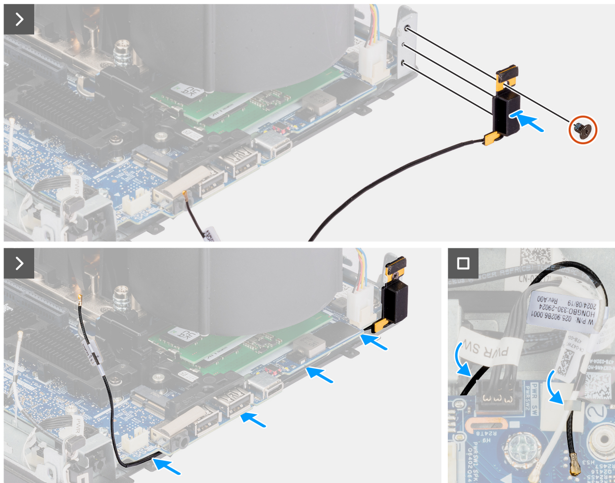
Figure 61. Installation de l'antenne interne (emplacement 2)
