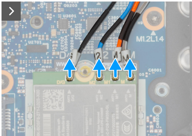
Figure 26. Removing the 5G WWAN card
