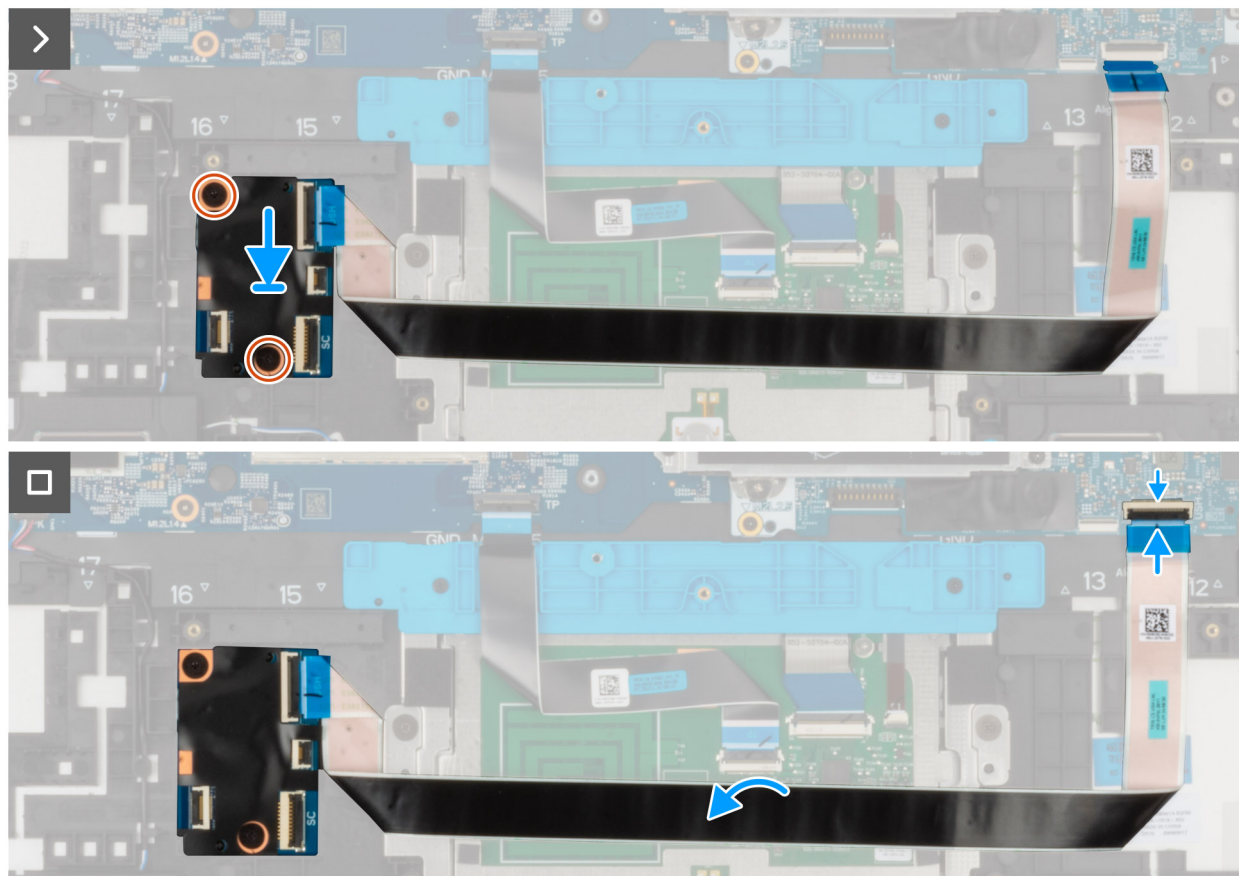
Figure 42. USH board
