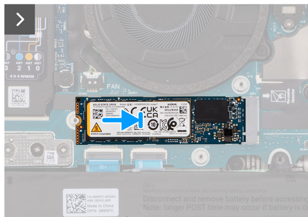
Figure 34. Installing the M.2 2280 SSD
