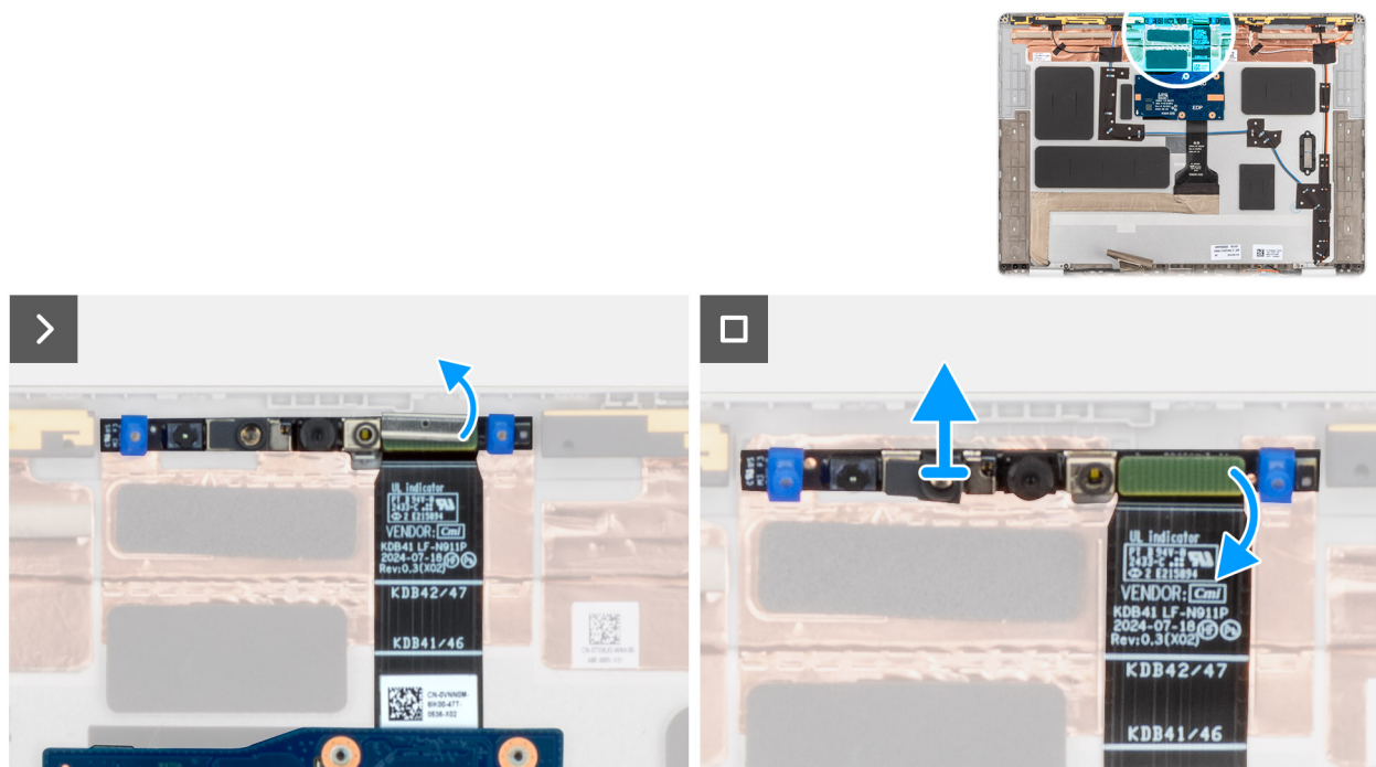
Figure 83. Removing the MIPI camera
