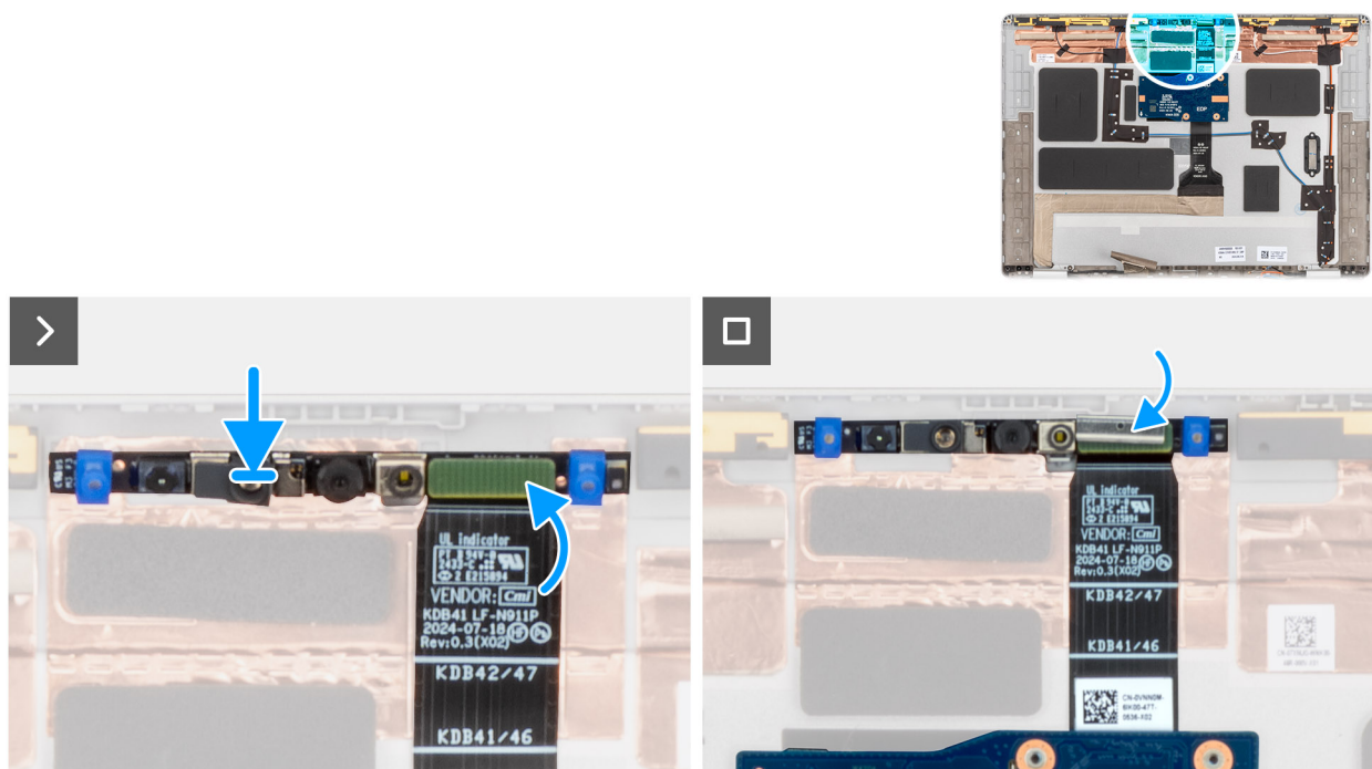
Figure 84. Installing the MIPI camera
