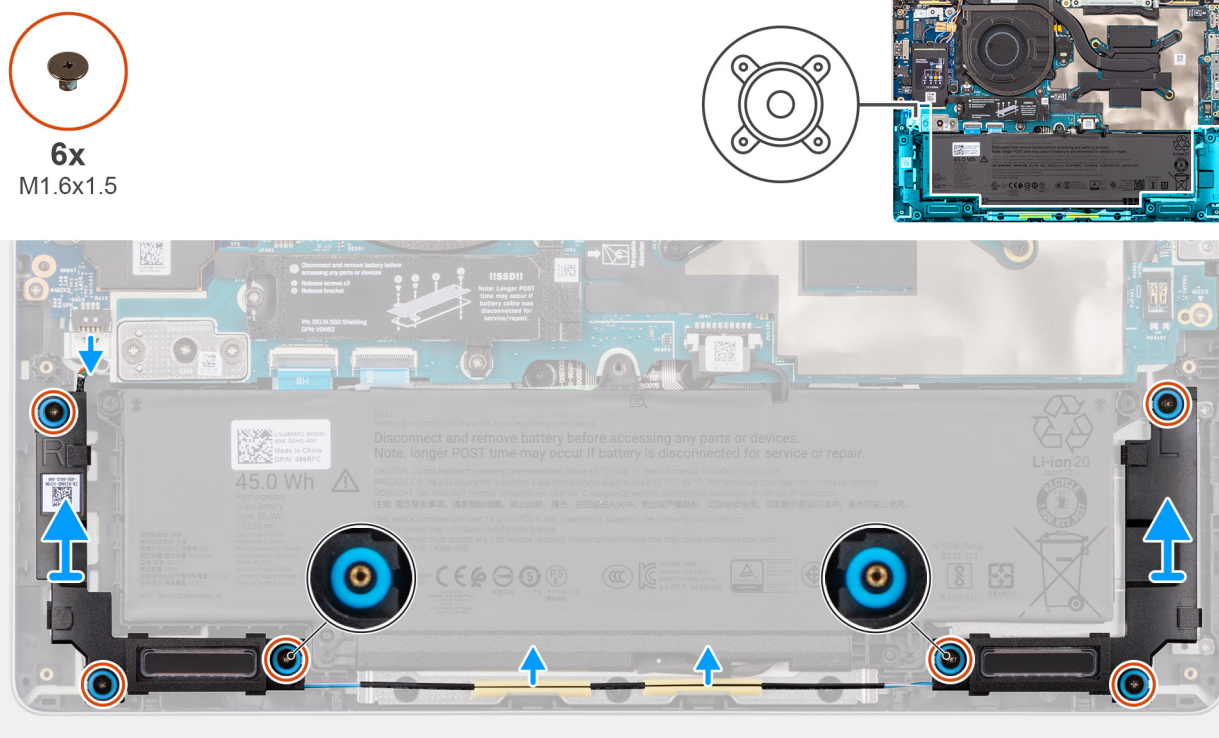
Figure 35. Removing the speakers
