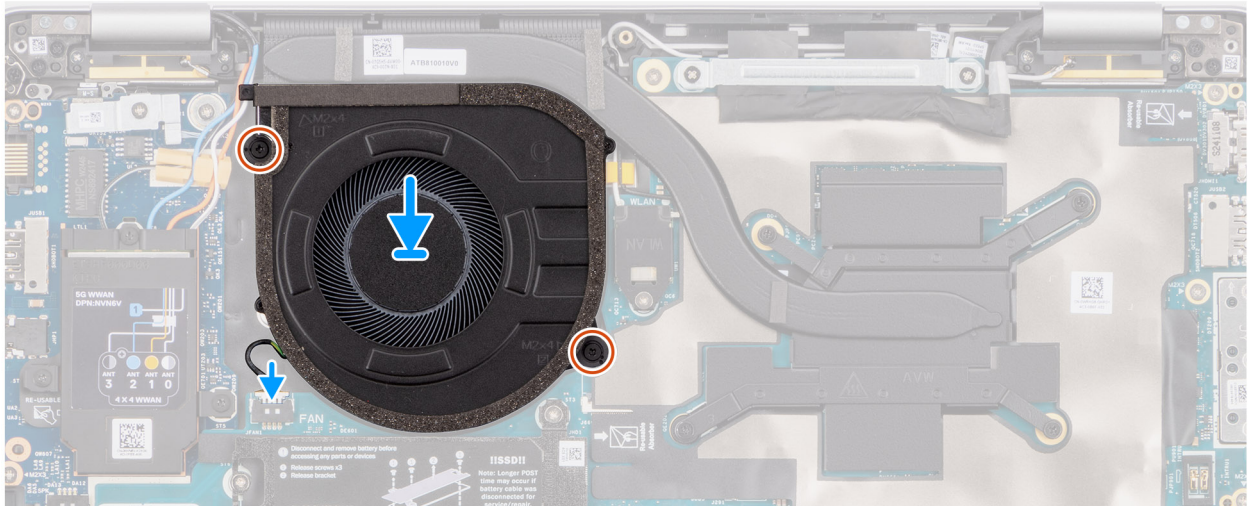
Figure 39. Installing the fan
