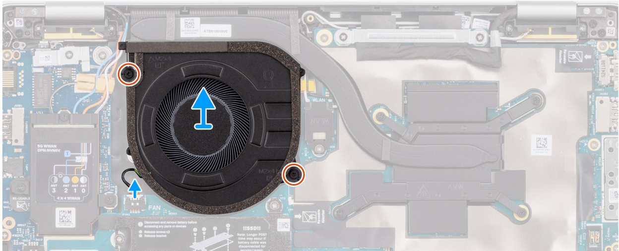
Figure 38. Removing the fan
