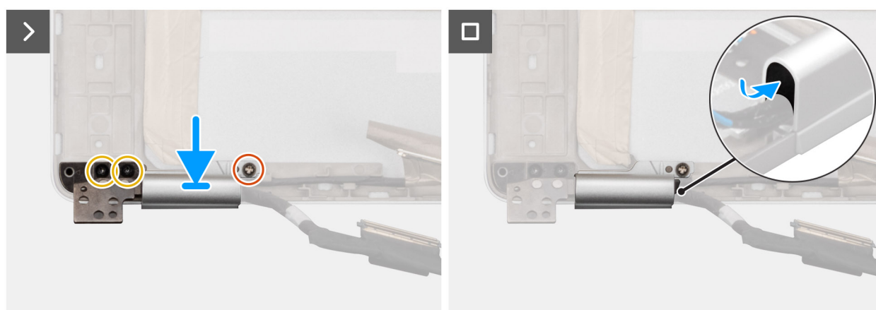
Figure 88. Installing the display cable for RGB/IR camera
