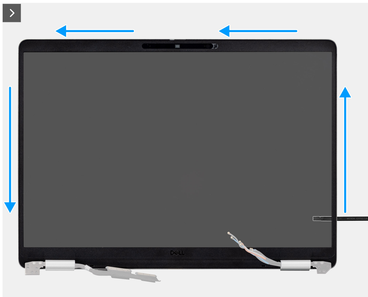
Figure 68. Prying the bezel along the sides
