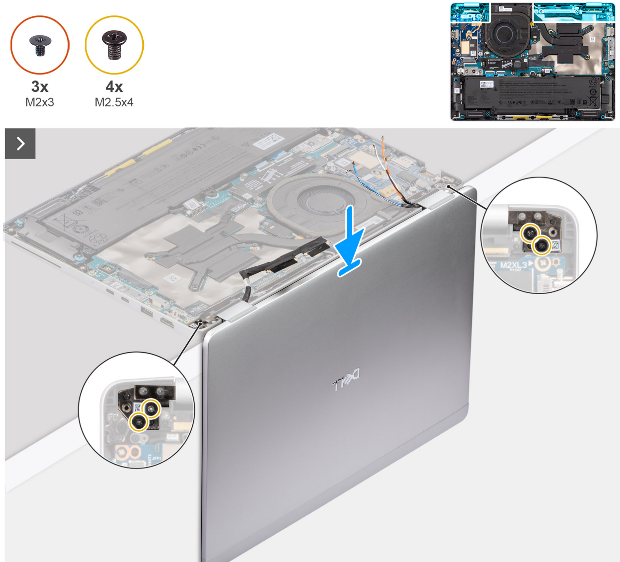
Figure 63. Aligning the display assembly with the palm-rest assembly
