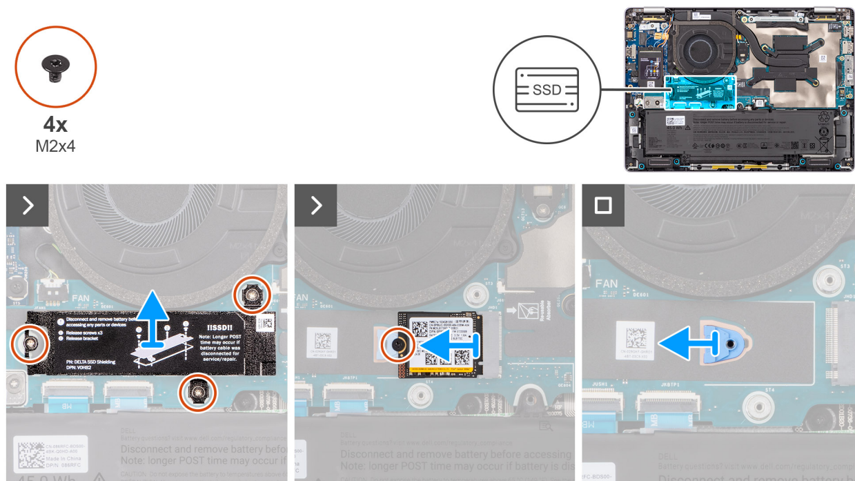
Figure 31. Removing the M.2 2230 SSD
