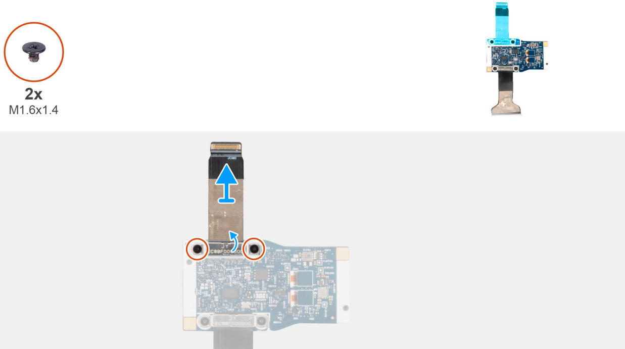
Figure 91. Removing the middle-board cable
