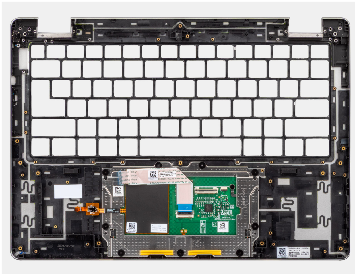
Figure 101. Palm-rest assembly
