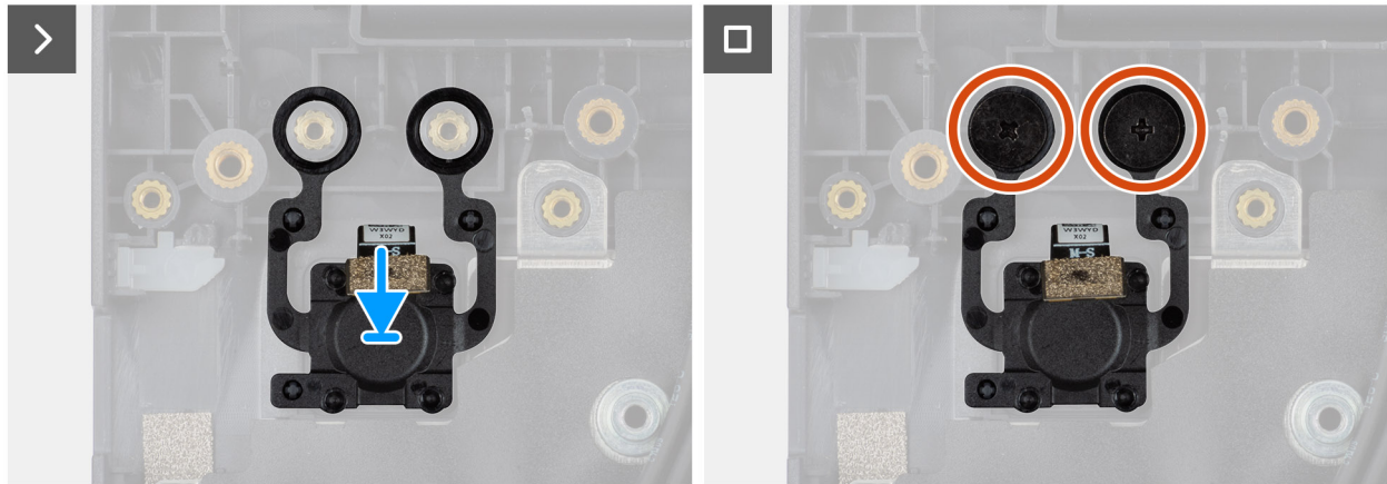
Figure 41. Installing the power button with a fingerprint reader
