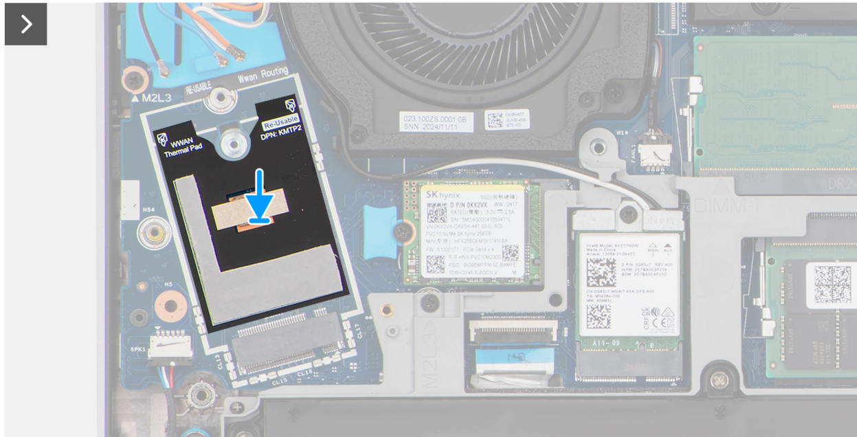
Figure 31. Installing the WWAN module
