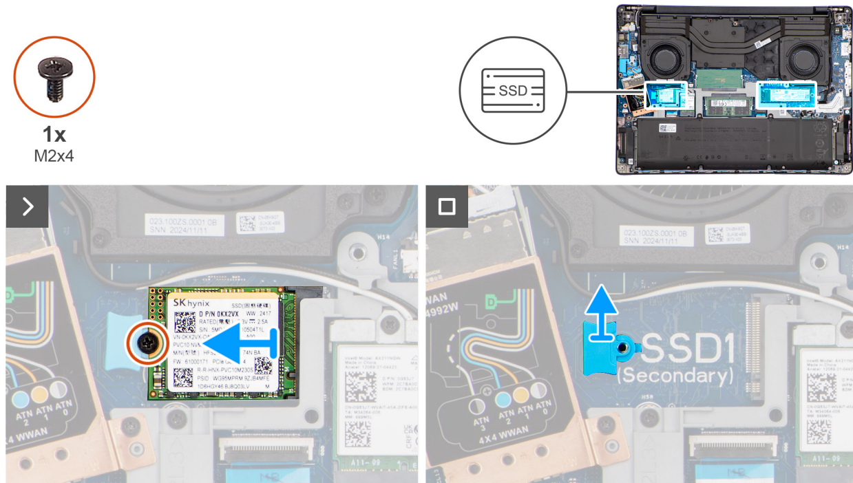
Figure 23. Removing the M.2 2230 solid state drive
