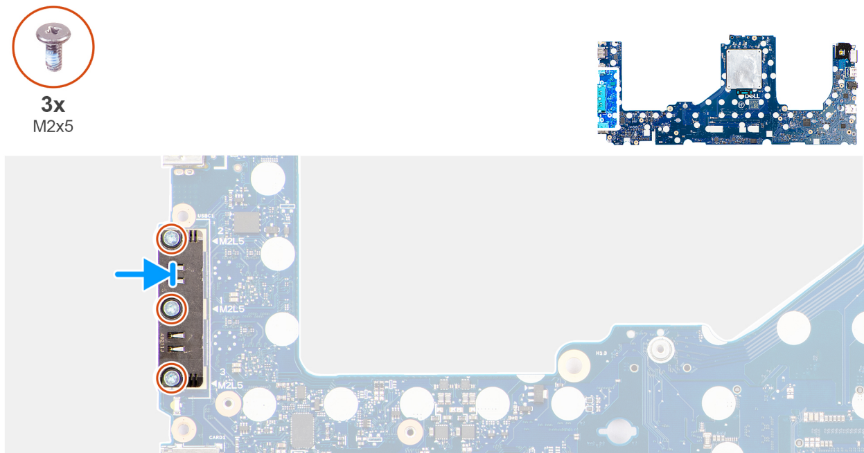
Figure 95. Installing the USB Type-C module
