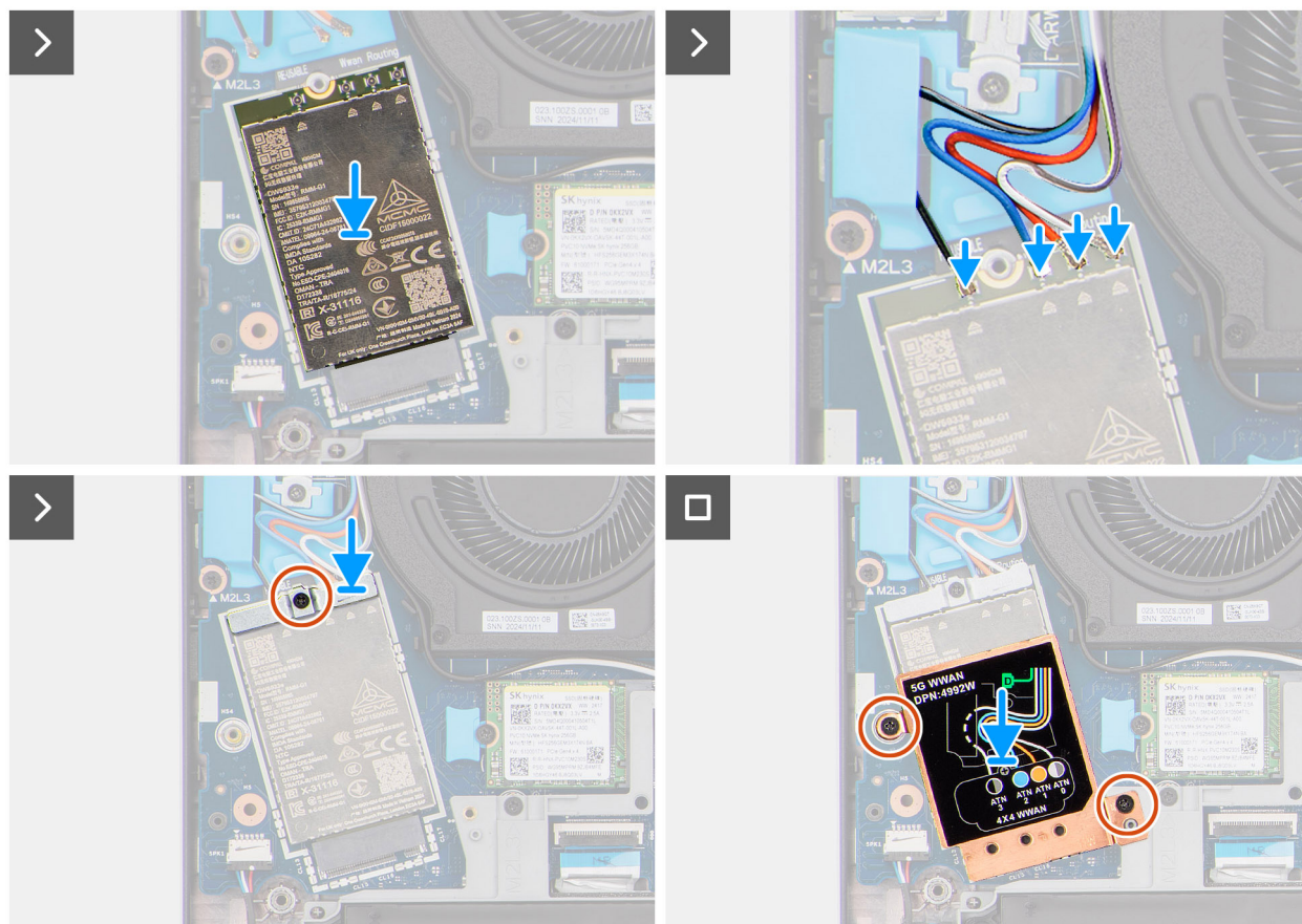
Figure 32. Installing the WWAN module
