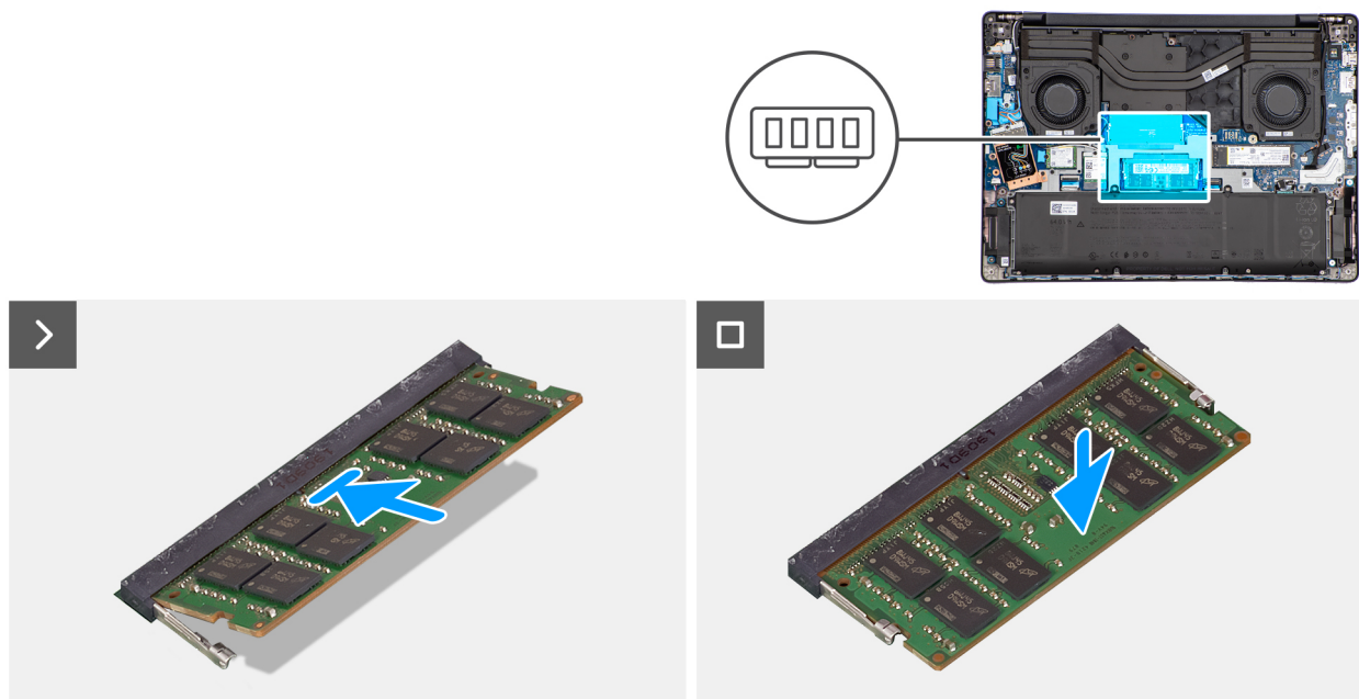
Figure 22. Installing the memory module
