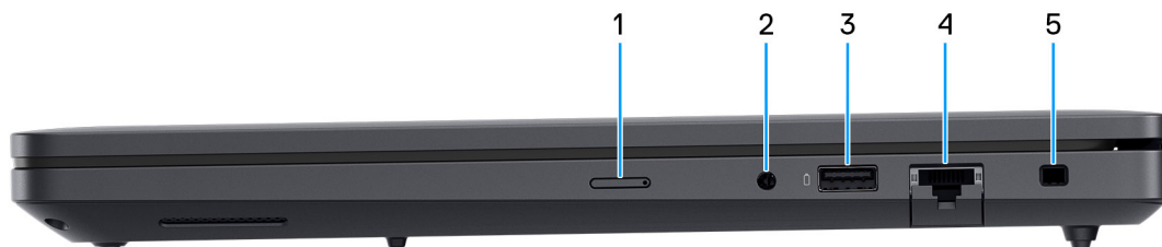
Figure 1. Right view
