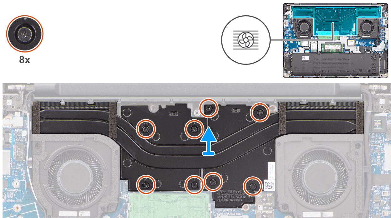
Figure 42. Removing the heat sink
