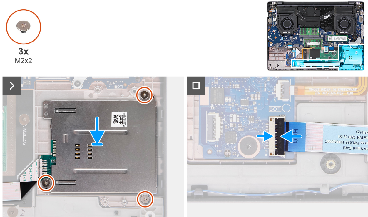
Figure 53. Installing the smart-card reader
