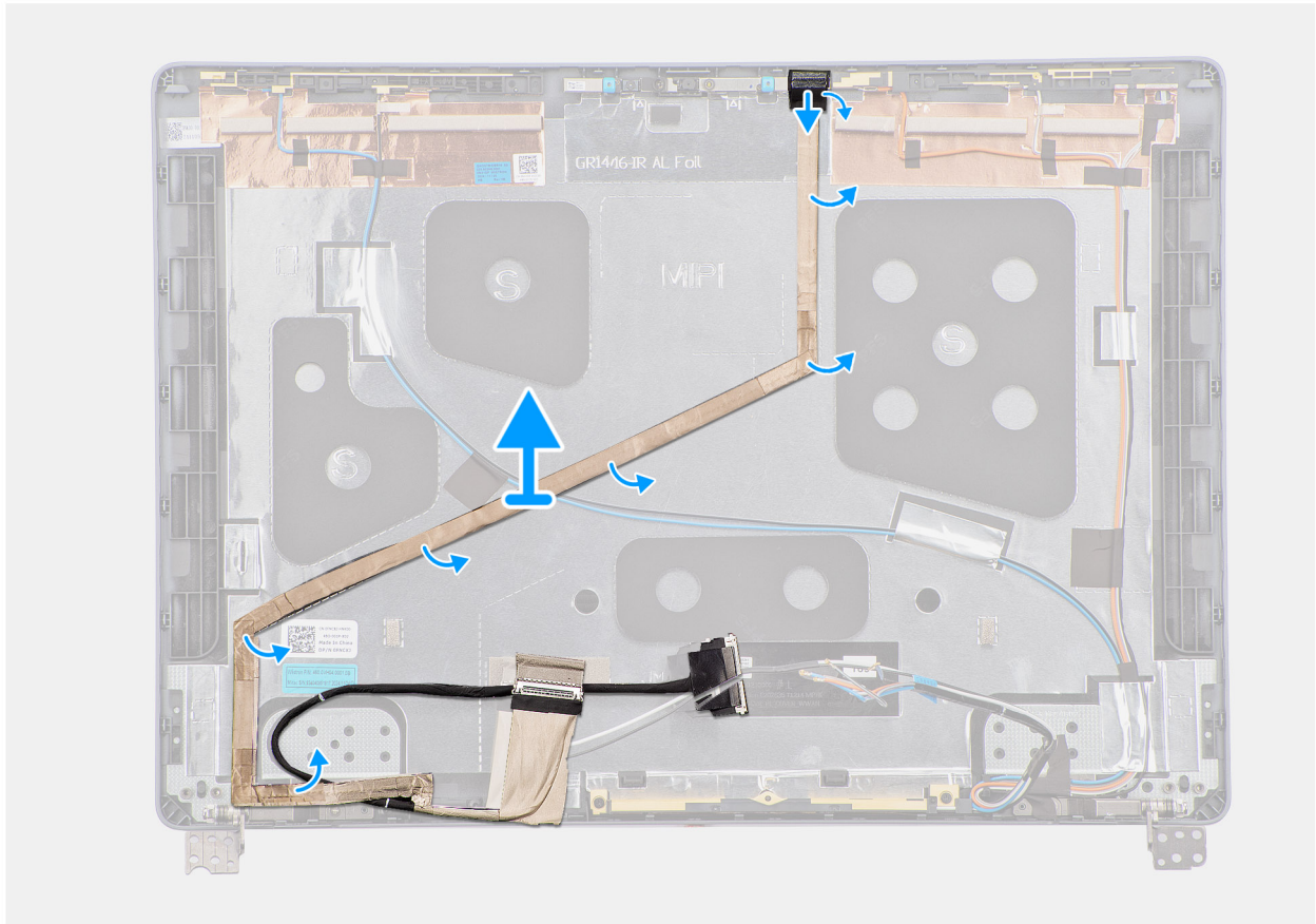
Figure 76. Removing the display cable
