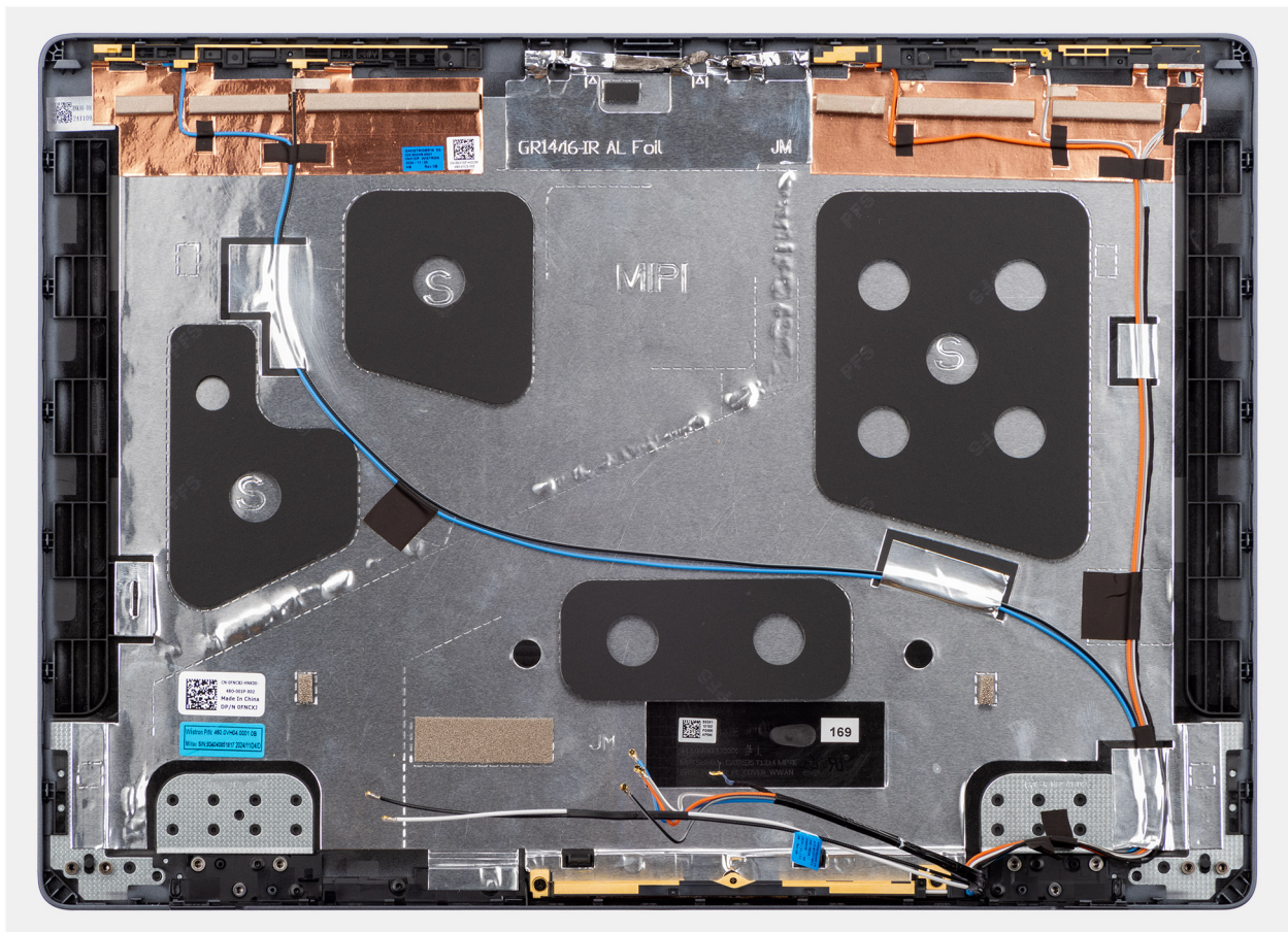
Figure 80. Display back-cover and antenna assembly
