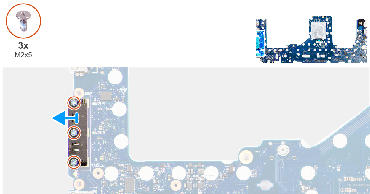
Figure 94. Removing the USB Type-C module
