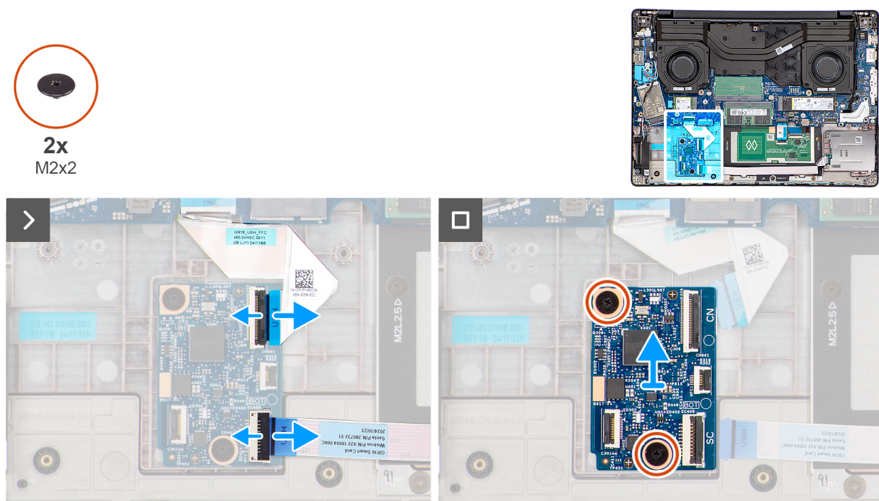
Figure 50. Removing the USH board
