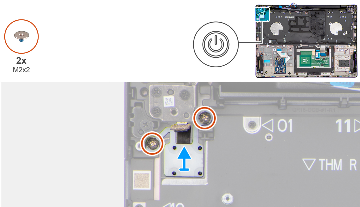
Figure 96. Removing the power button
