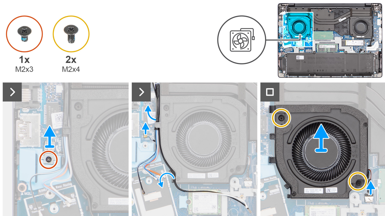
Figure 36. Removing the right/processor fan
