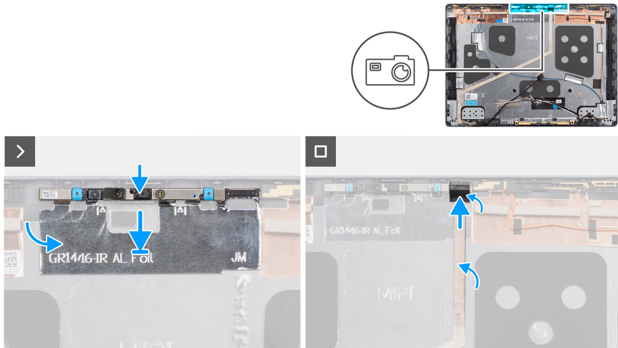
Figure 79. Installing the camera
