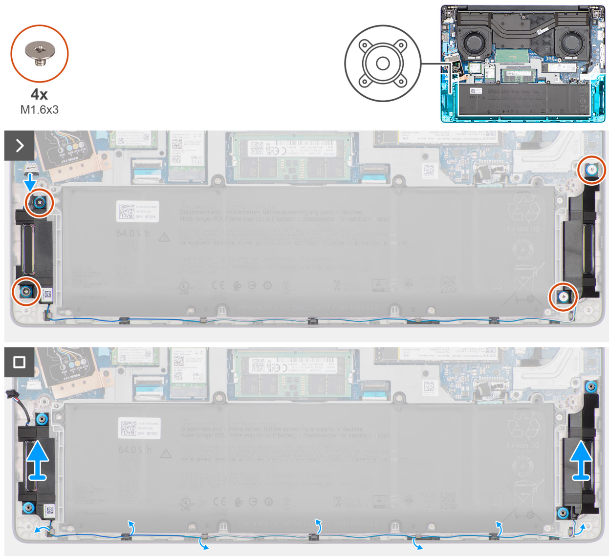
Figure 33. Removing the speakers
