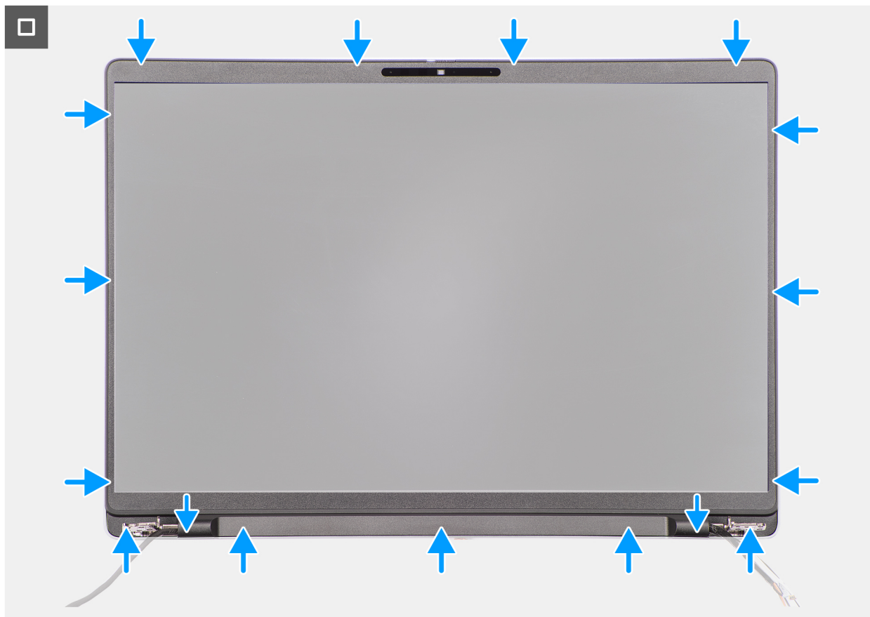
Figure 67. Installing the display bezel
