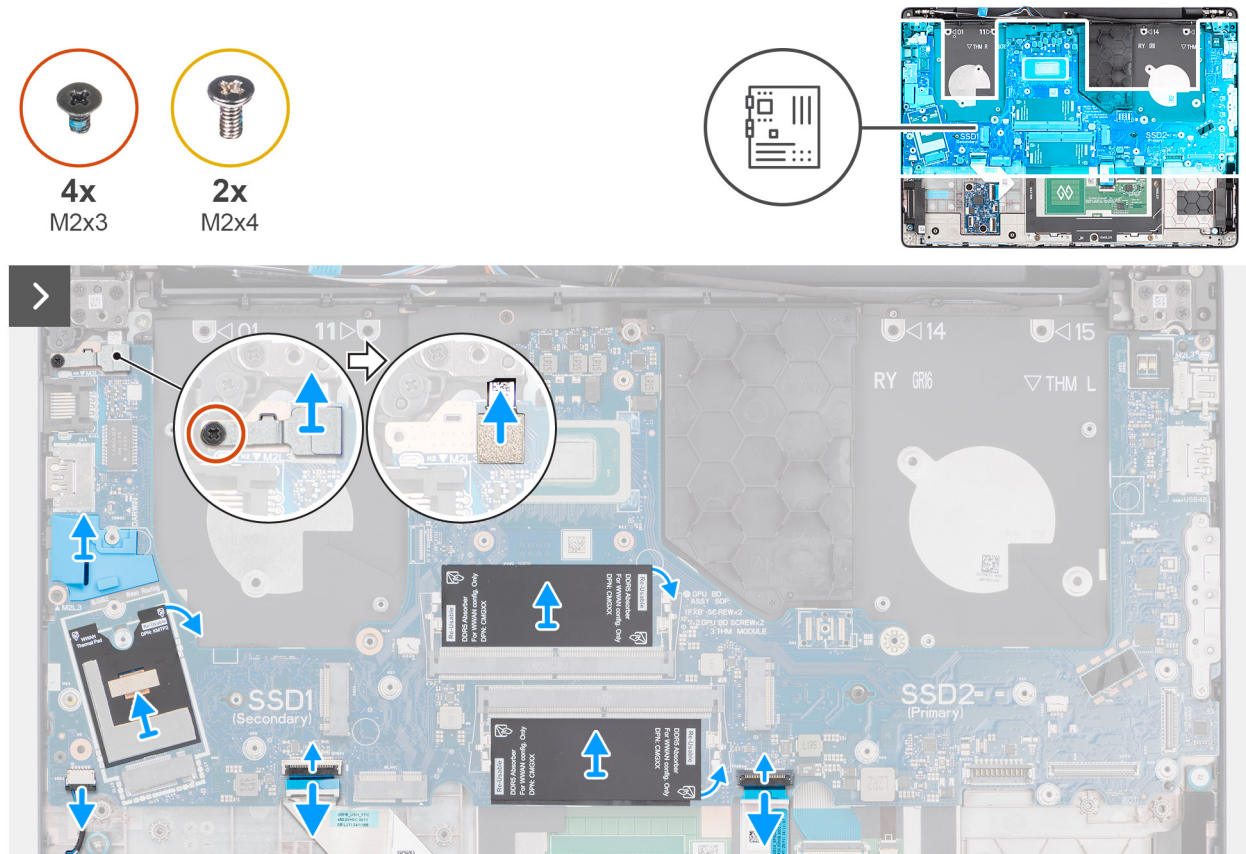
Figure 83. Removing the system board
