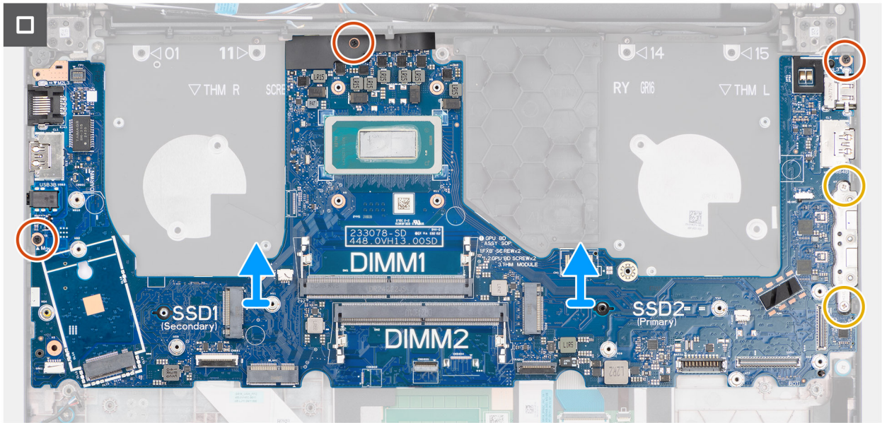
Figure 84. Removing the system board
