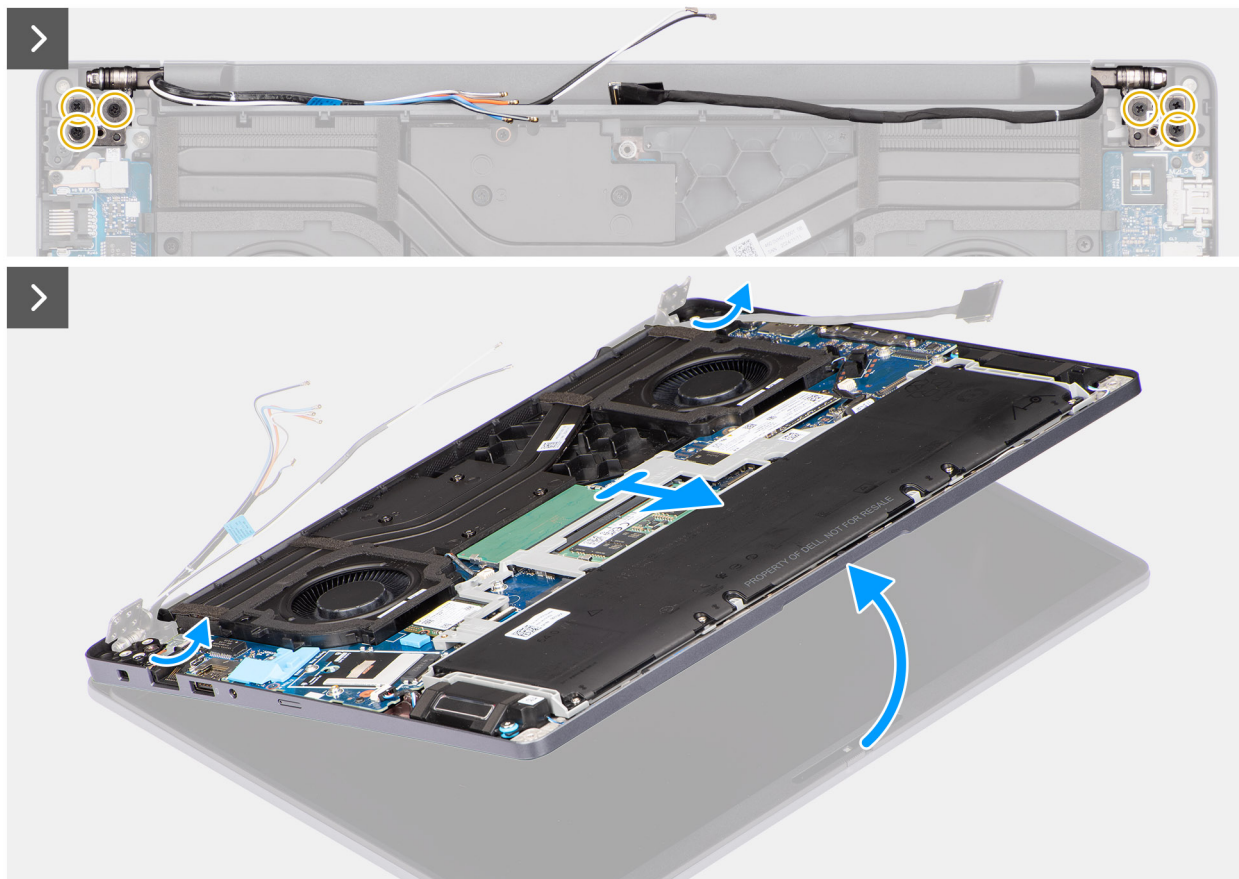
Figure 55. Removing the display assembly
