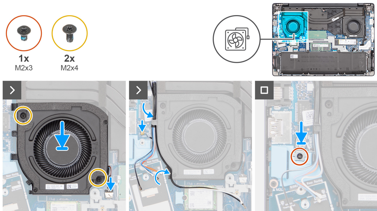
Figure 37. Installing the right/processor fan
