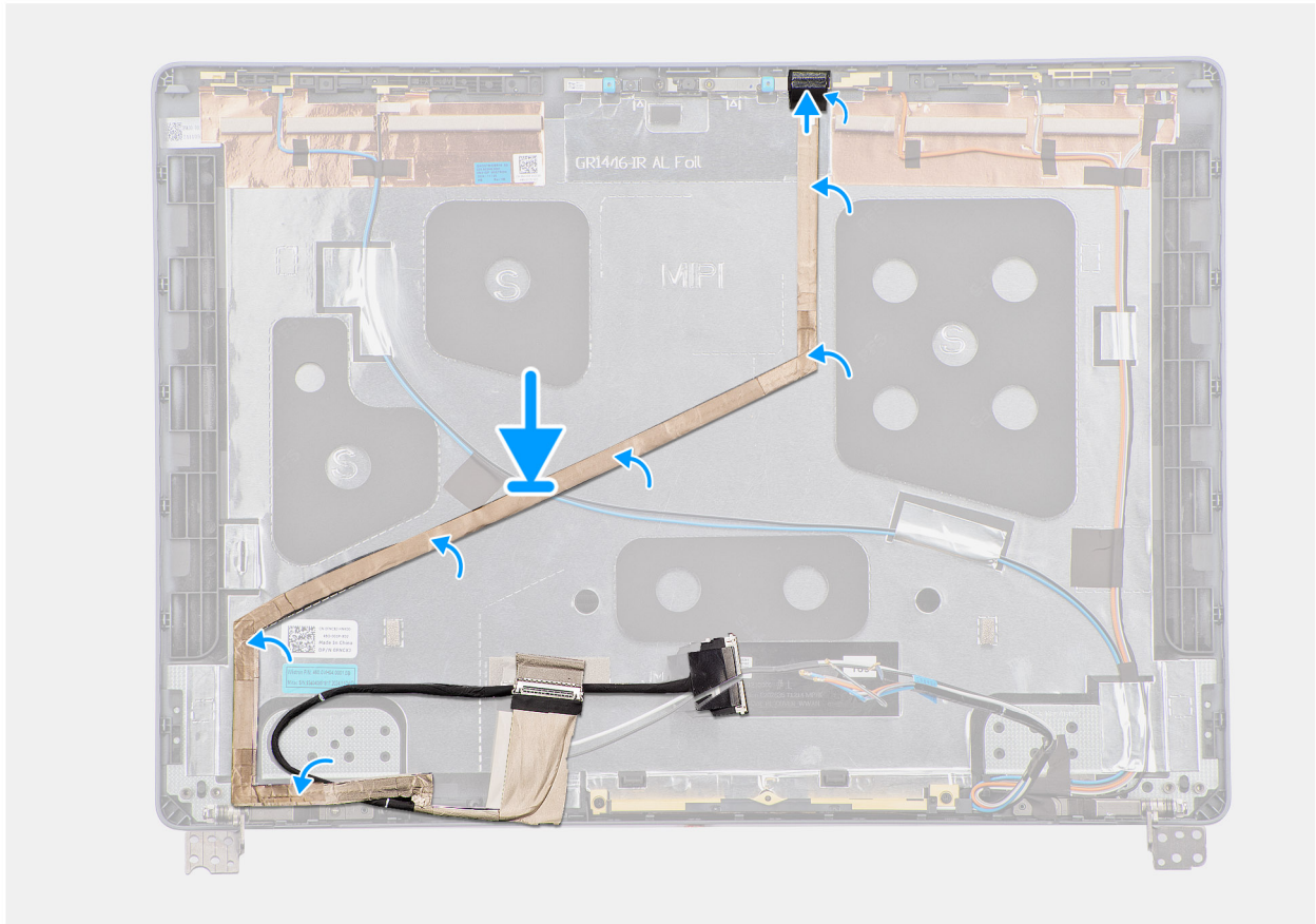
Figure 77. Installing the display cable
