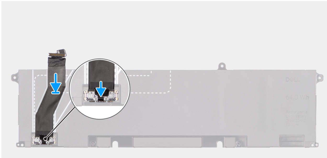
Figure 20. Connecting the battery cable
