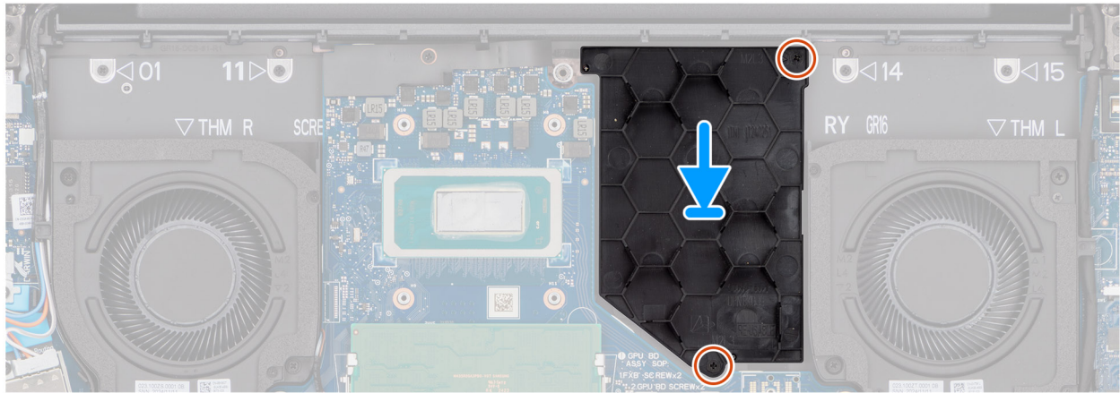
Figure 45. Installing the GPU filler
