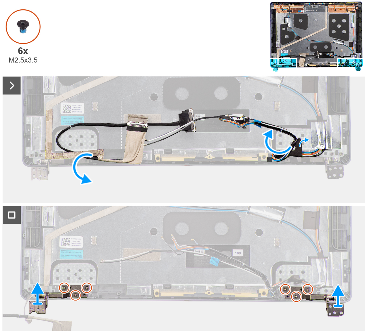
Figure 74. Removing the display hinges
