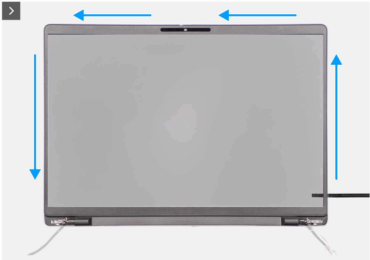
Figure 62. Removing the display bezel
