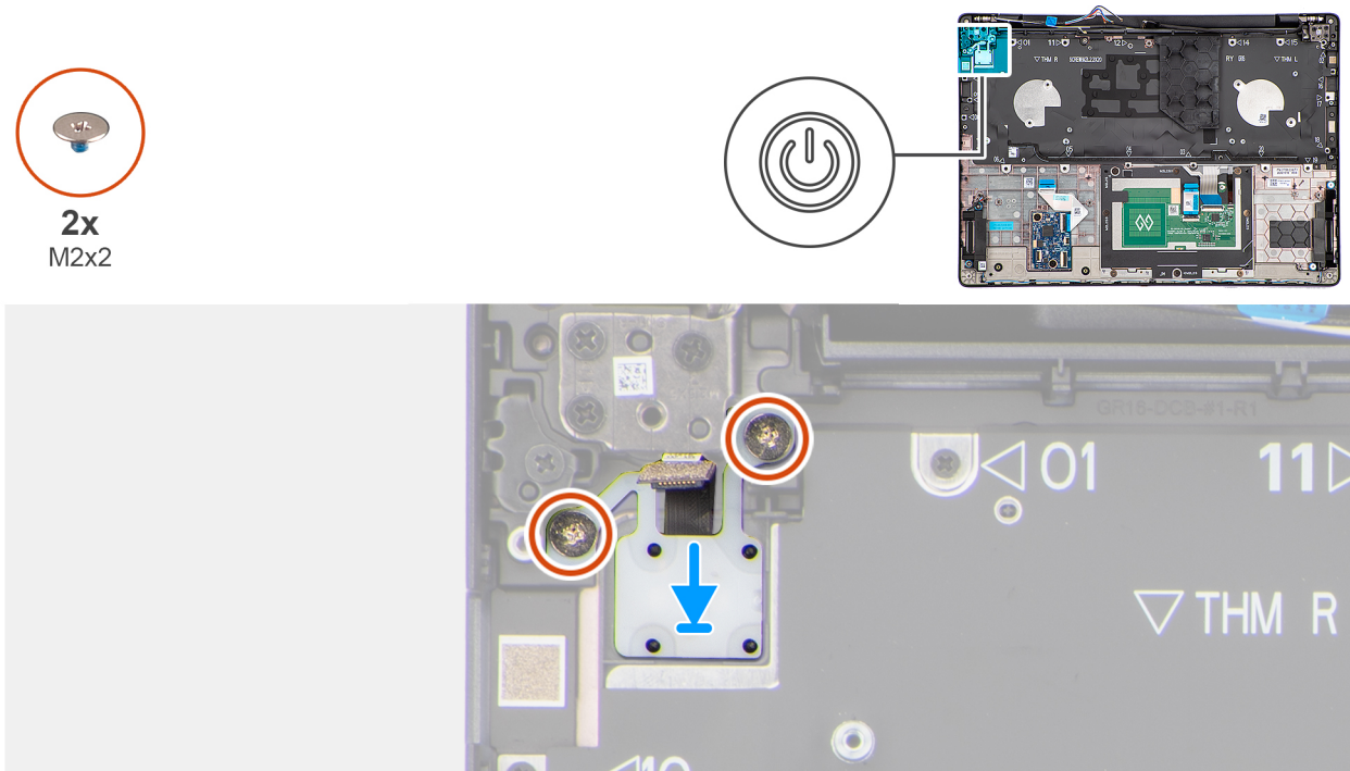
Figure 97. Installing the power button
