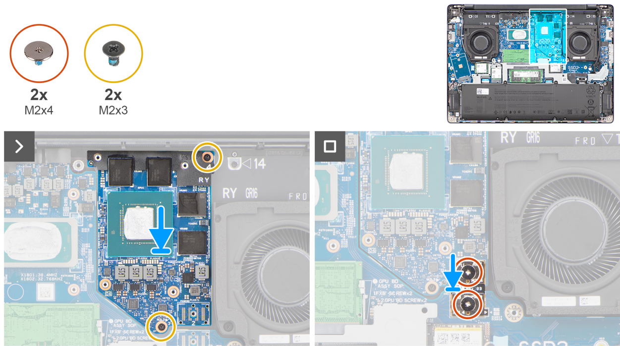
Figure 47. Installing the GPU
