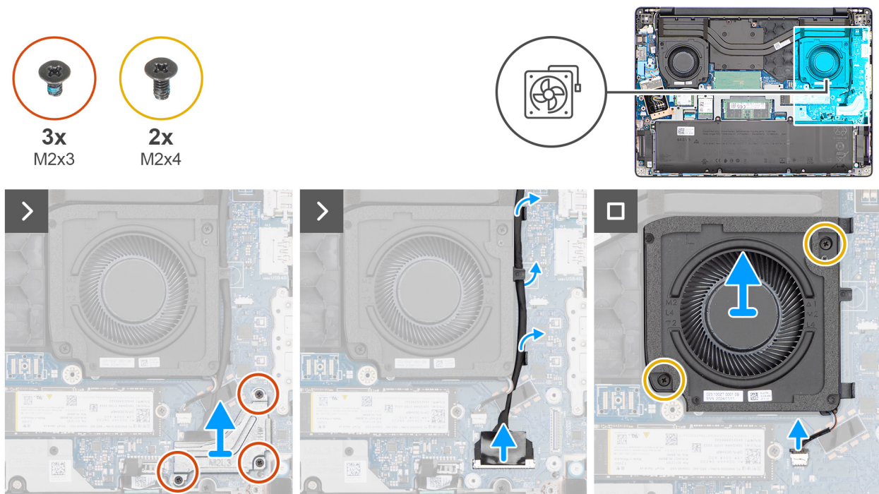
Figure 38. Removing the left/video fan
