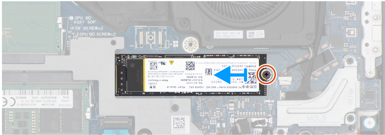
Figure 25. Removing the M.2 2280 solid state drive
