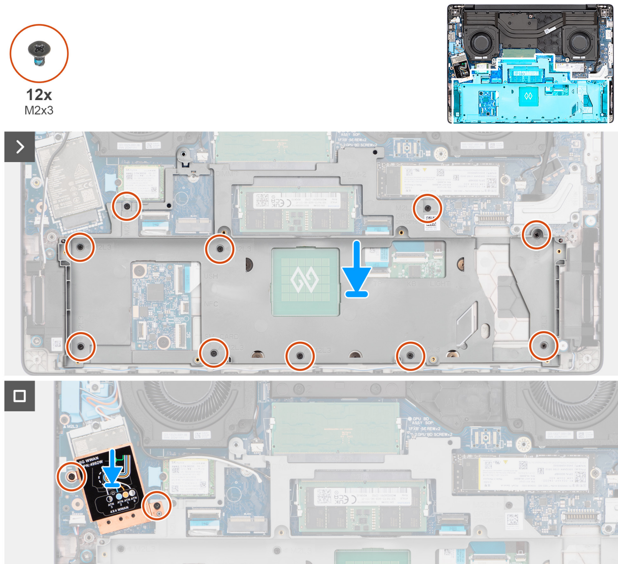
Figure 49. Installing the battery frame
