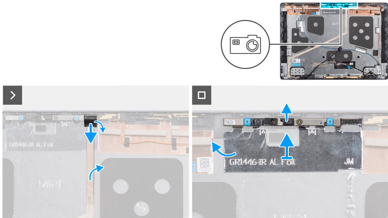
Figure 78. Removing the camera
