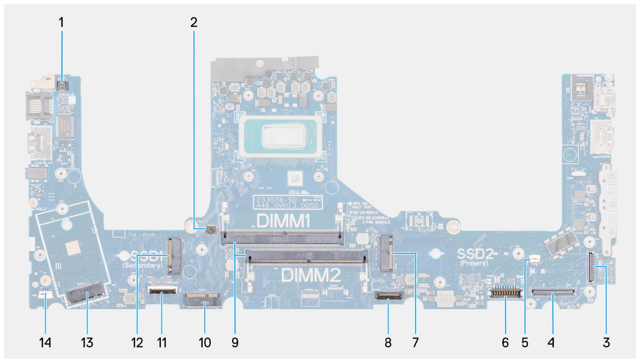
Figure 85. System board connectors
