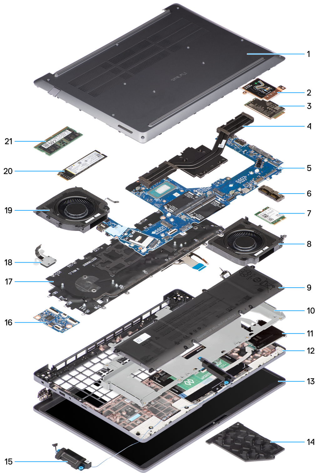
Figure 11. Major components of your Dell Pro Max 16 MC16250
