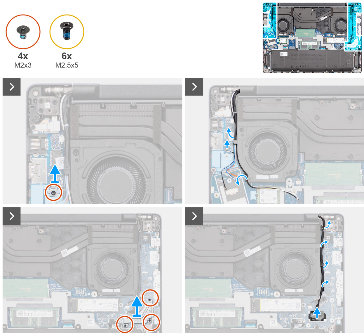
Figure 54. Removing the display assembly
