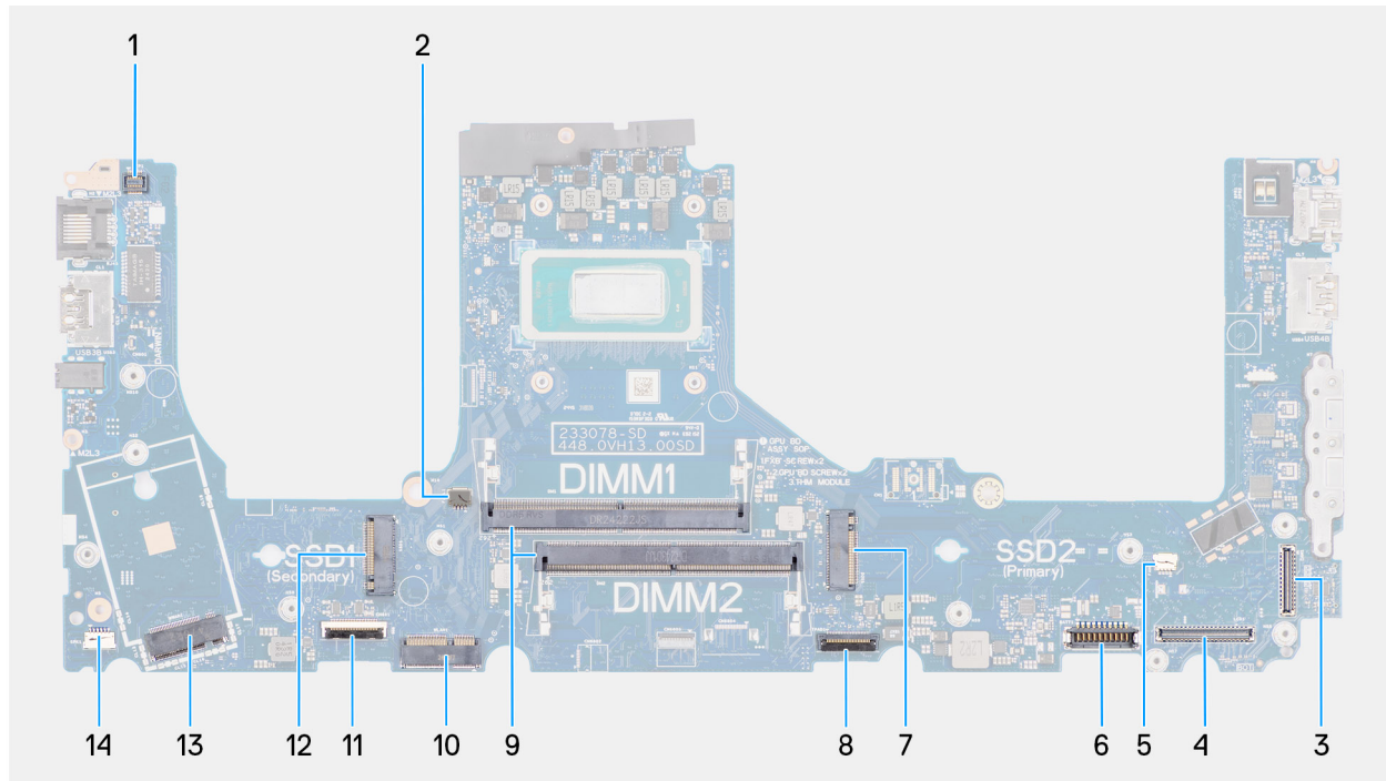
Figure 88. System board connectors
