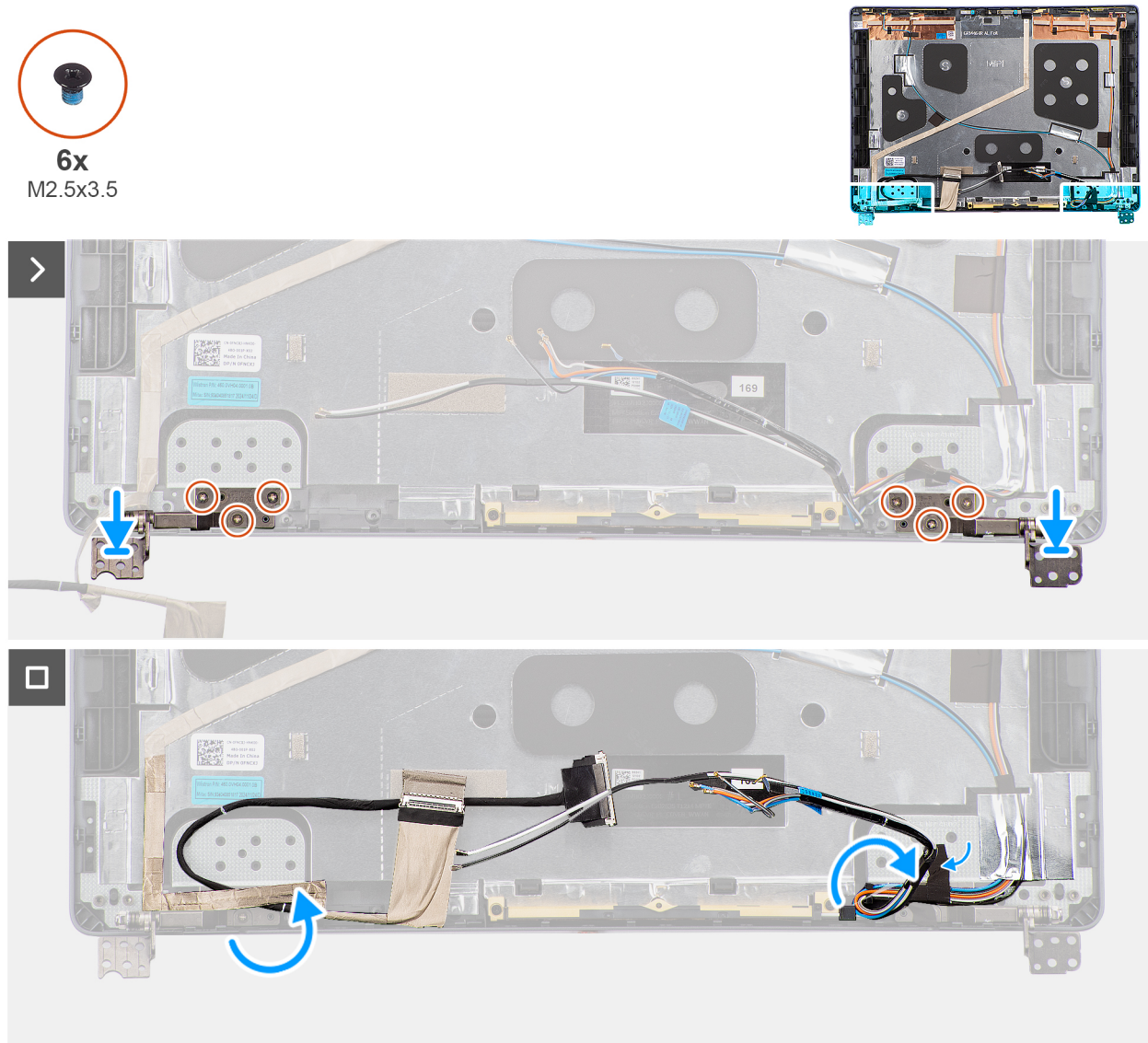
Figure 75. Installing the display hinges
