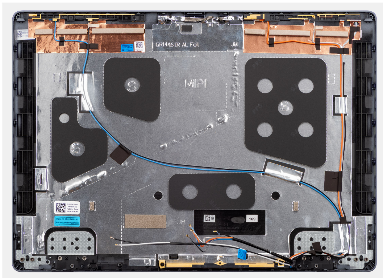
Figure 81. Display back-cover and antenna assembly
