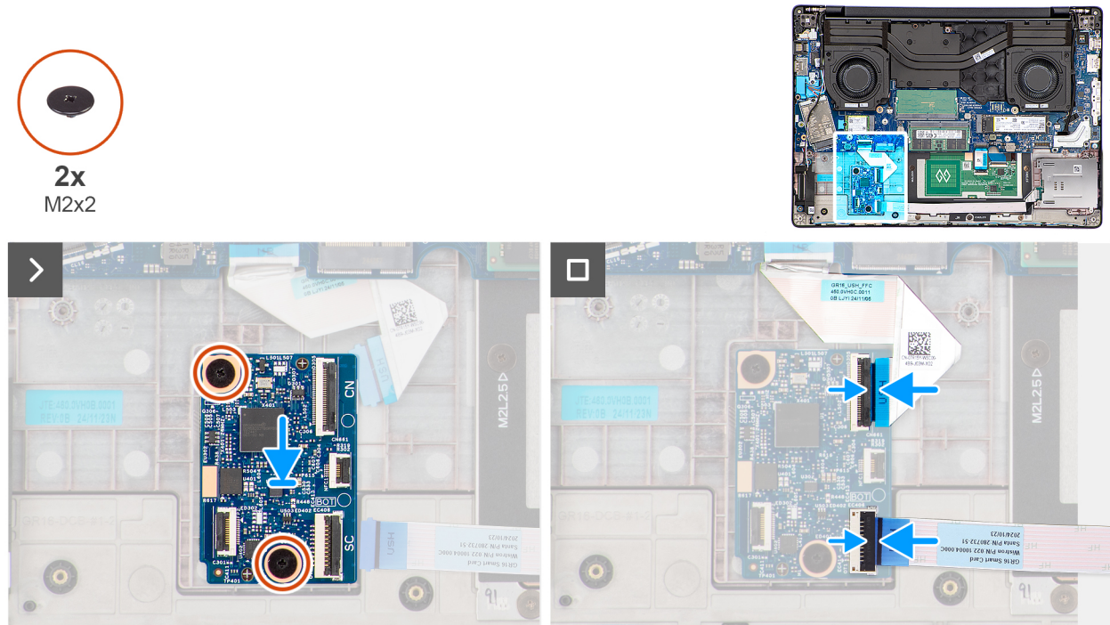
Figure 51. Installing the USH board
