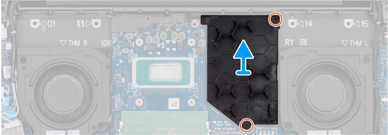
Figure 44. Removing the GPU filler
