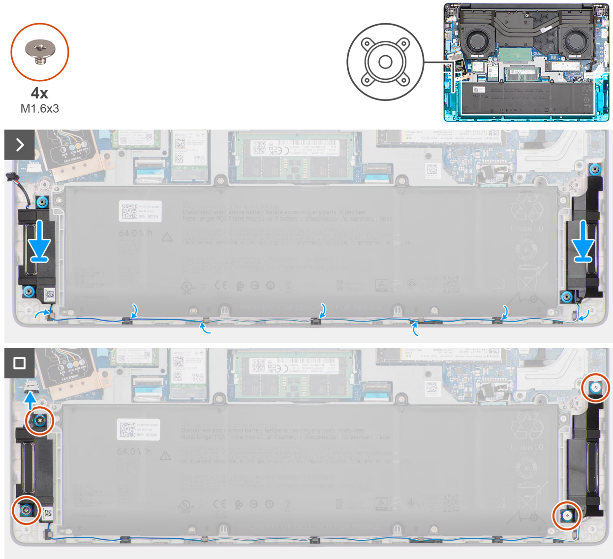
Figure 34. Installing the speakers
