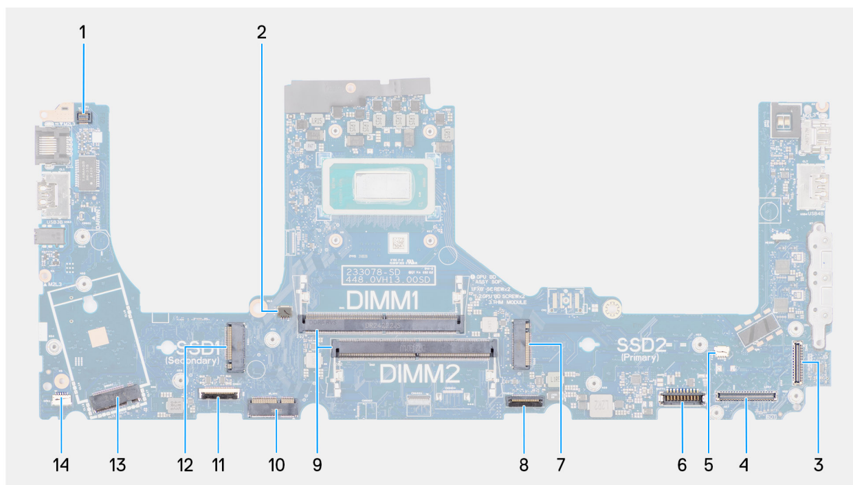
Figure 82. System board connectors
