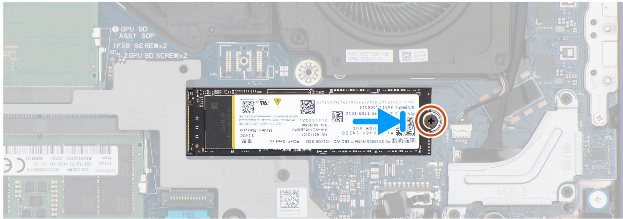
Figure 26. Installing the M.2 2280 solid state drive
