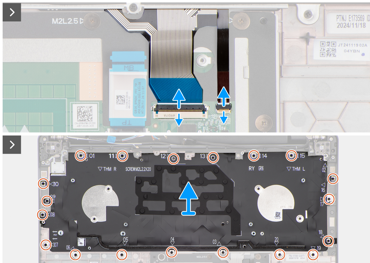
Figure 98. Removing the keyboard
