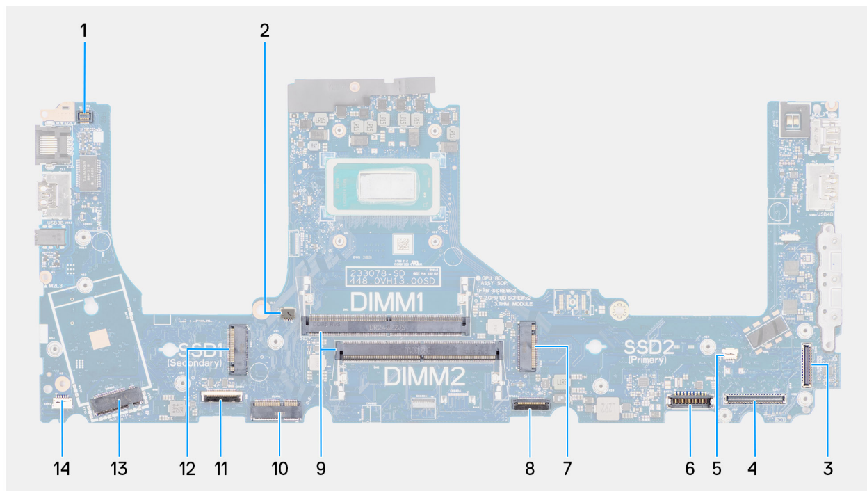
Figure 91. System board connectors
