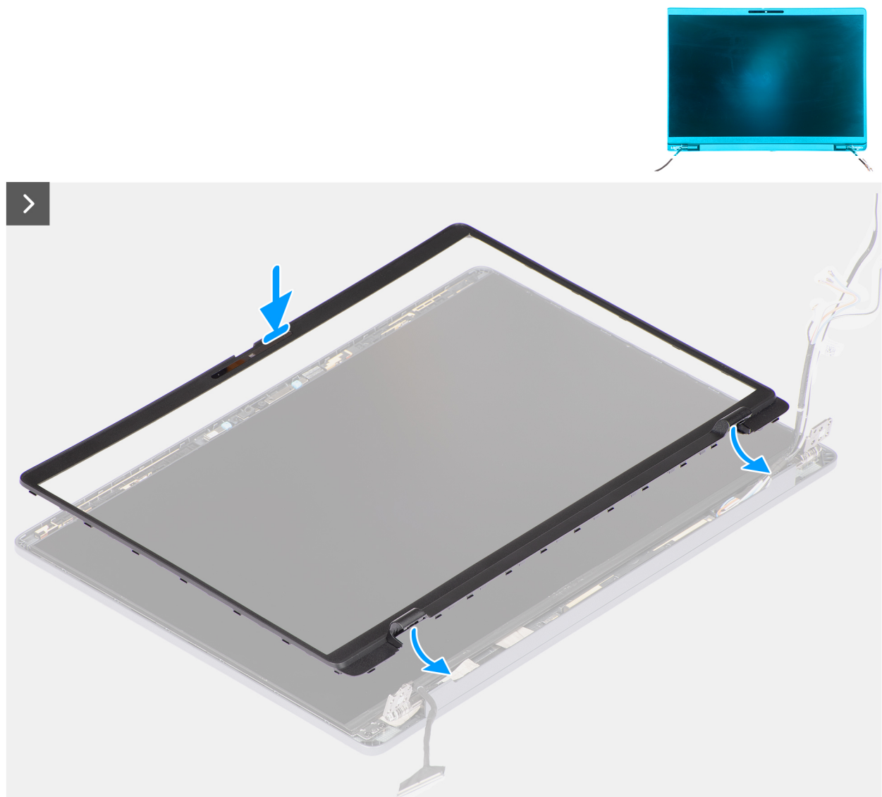
Figure 66. Installing the display bezel
