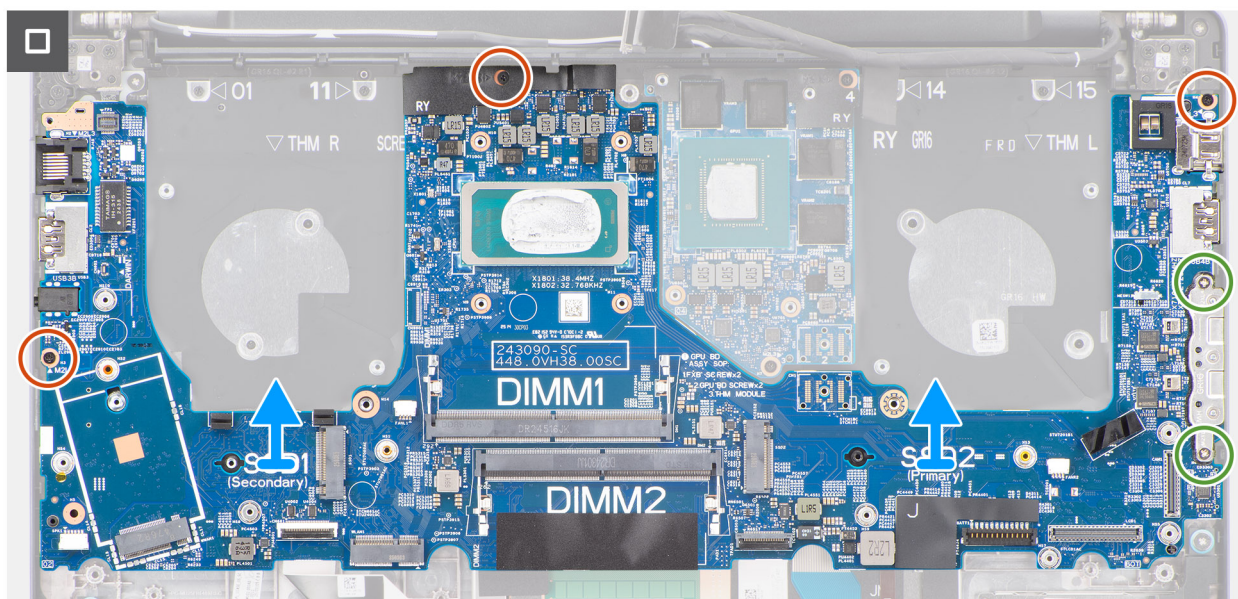
Figure 90. Removing the system board
