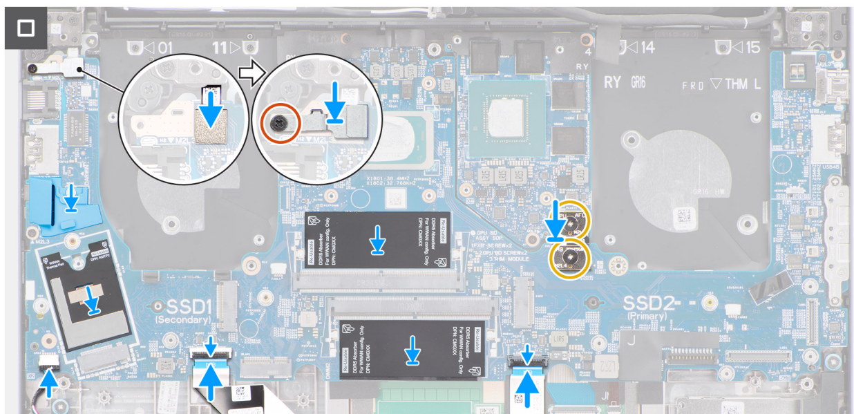
Figure 93. Installing the system board
