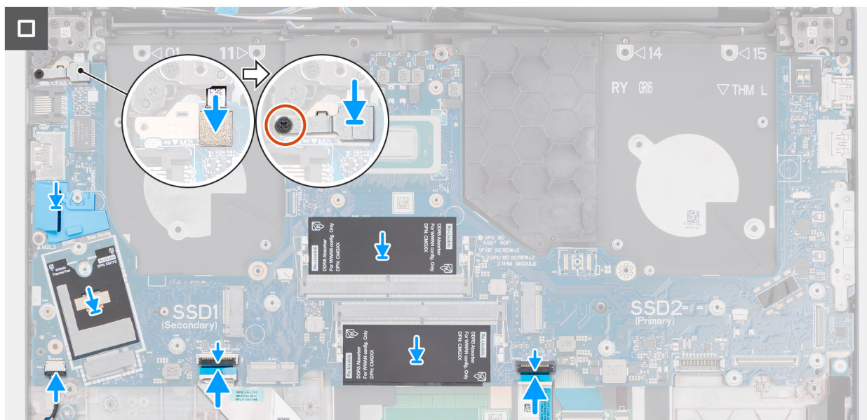
Figure 87. Installing the system board
