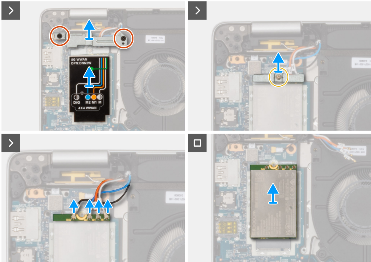
Figure 23. Removing the 5G WWAN card
