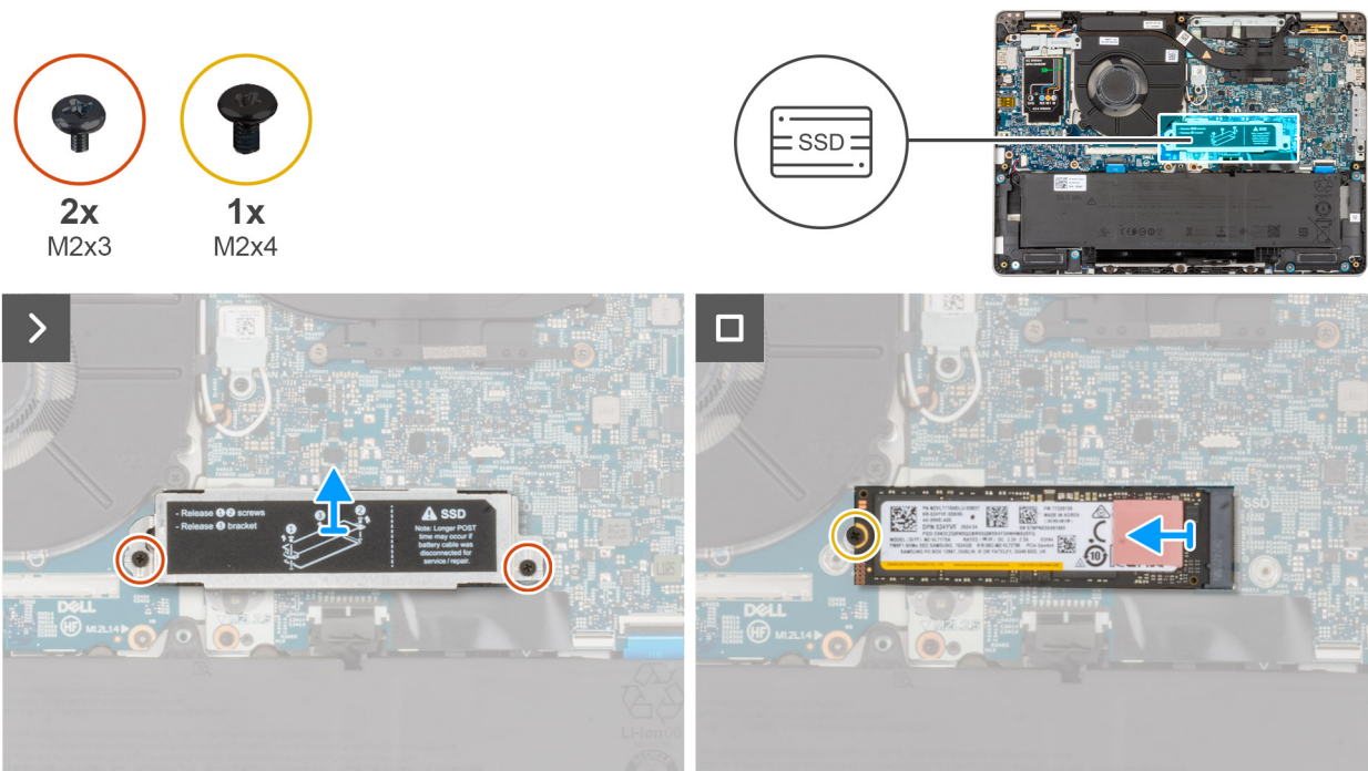
Figure 27. Removing the M.2 2280 SSD
