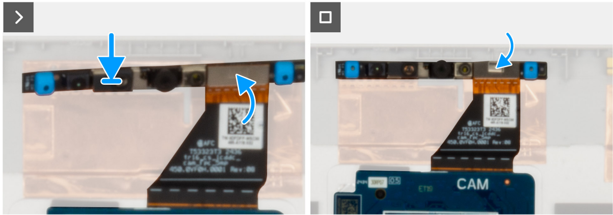
Figure 70. Installing the camera module
