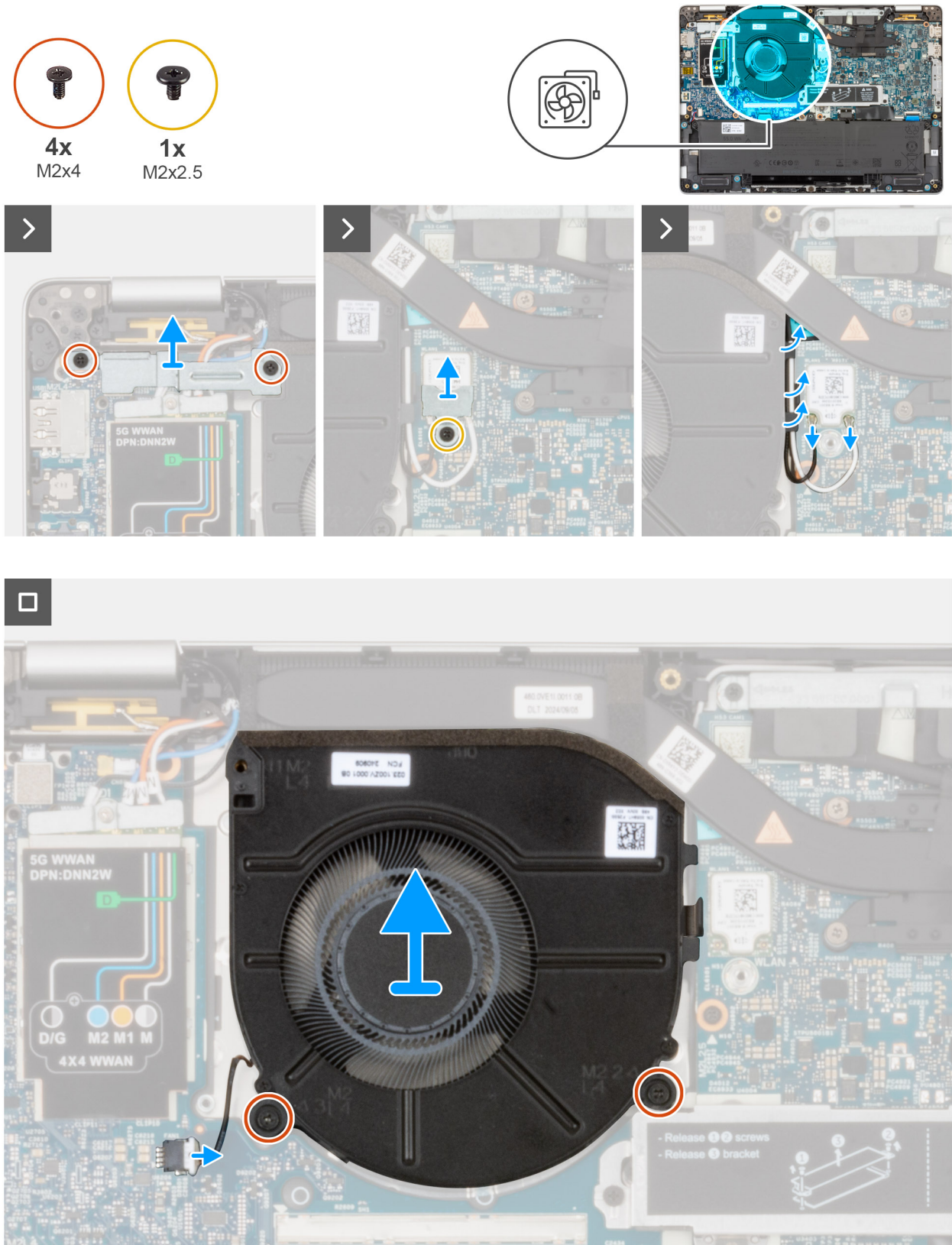
Figure 31. Removing the fan
