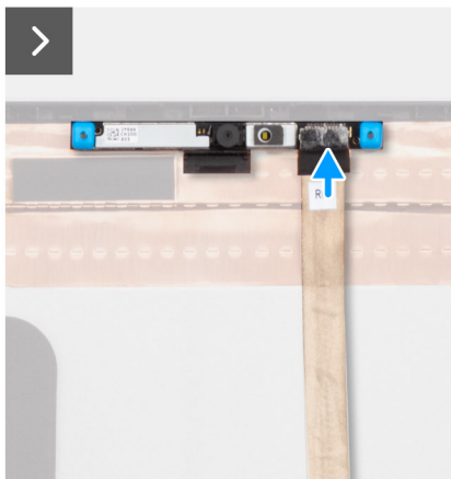
Figure 72. Installing the display cable
