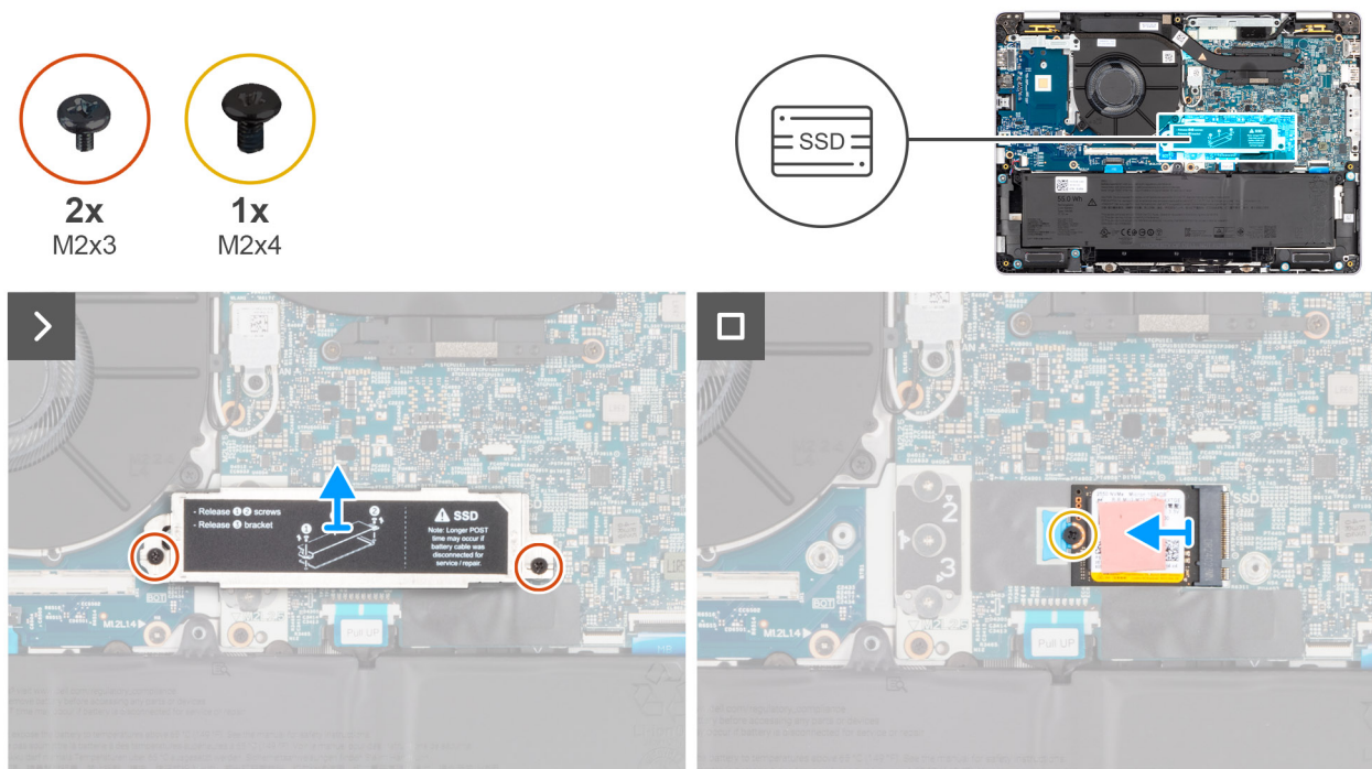
Figure 25. Removing the M.2 2230 SSD
