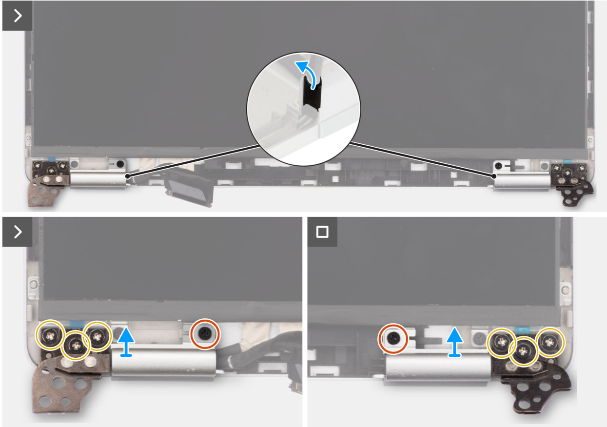
Figure 64. Removing the display hinges
