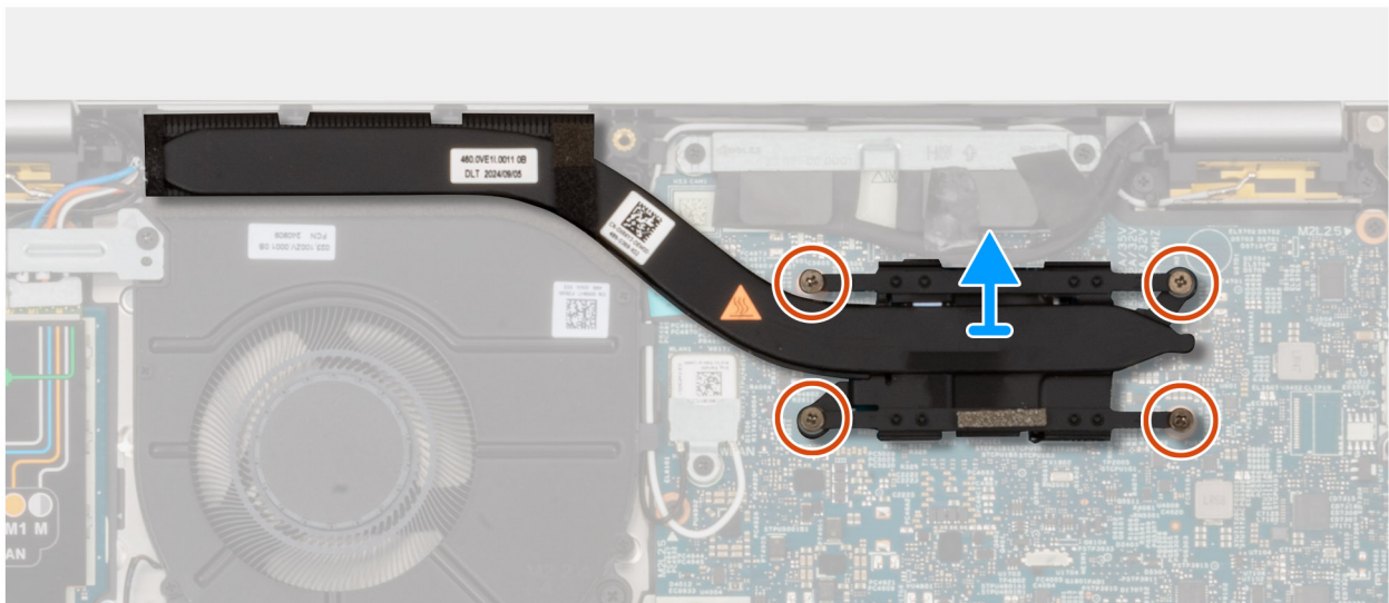
Figure 38. Removing the heat sink
