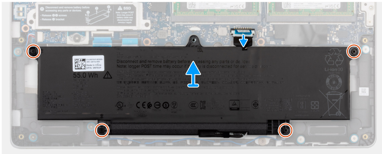
4x M2x4.5
