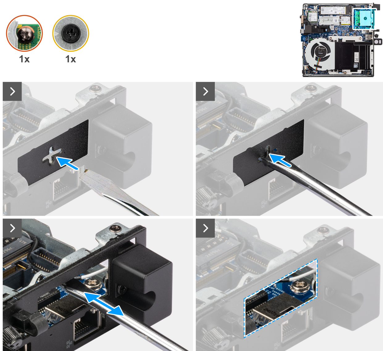
Figure 66. Installation du module de port Ethernet RJ45
