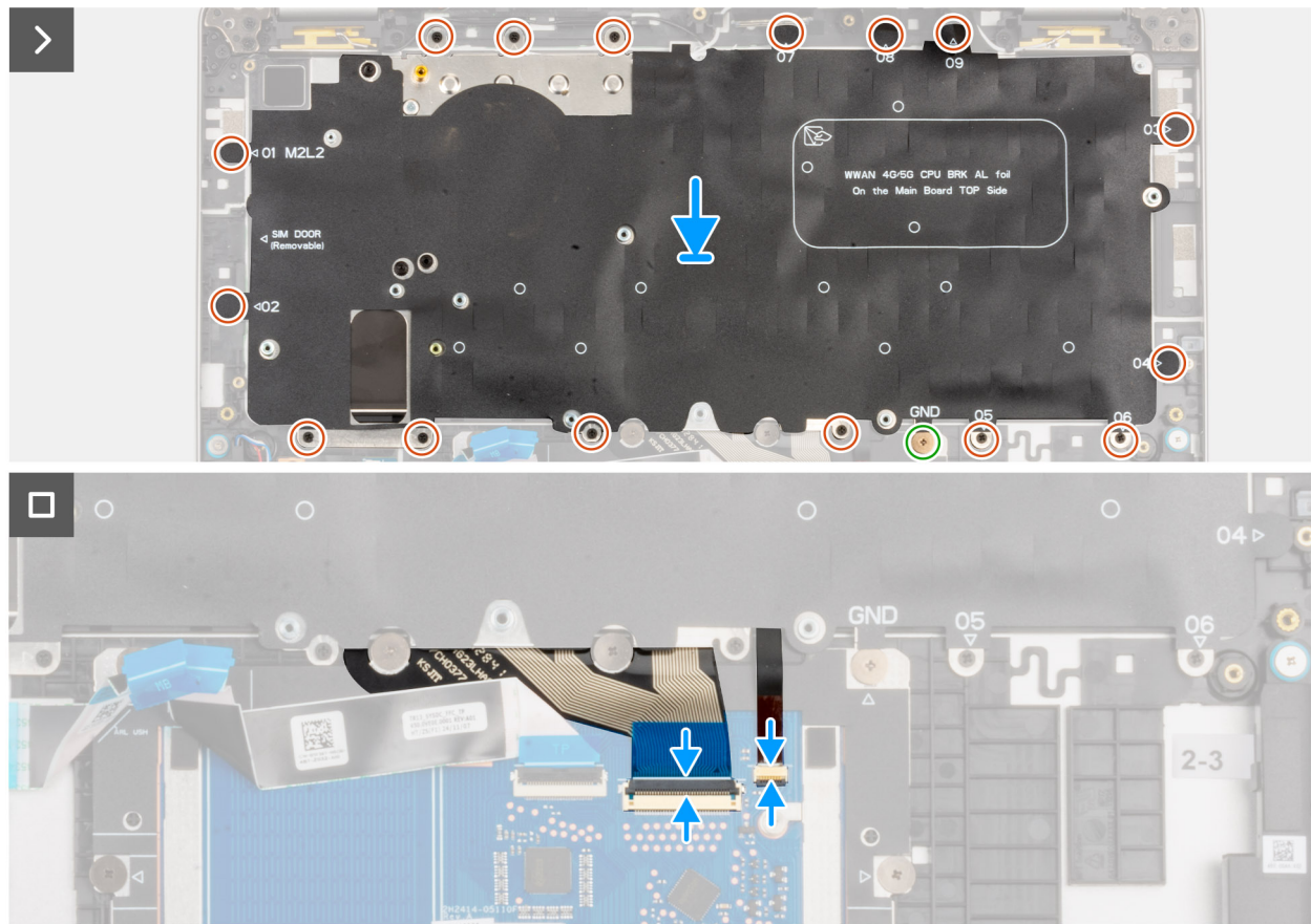
Figure 69. Installing the keyboard
