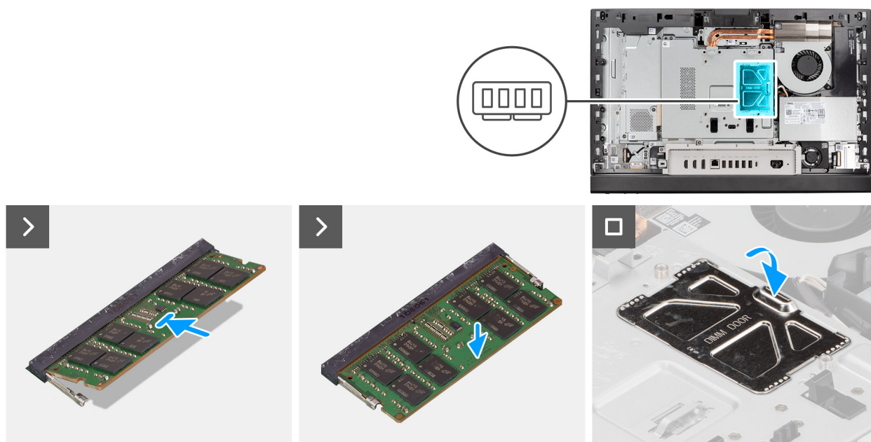
Figure 24. Installation de la mémoire
