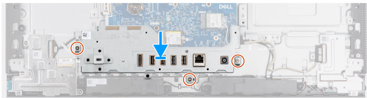
Figure 39. Installation du support d'E/S
