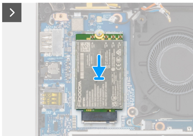
2x M2x4
