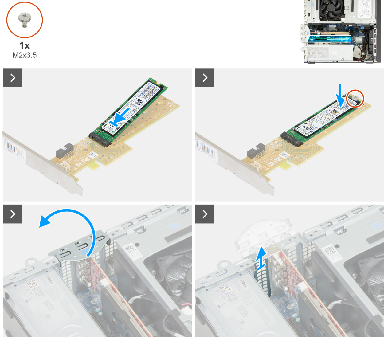
Figure 39. Installing the solid state drive expansion card
