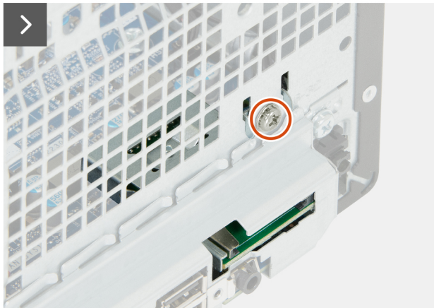
Figure 66. Removing the media-card reader
