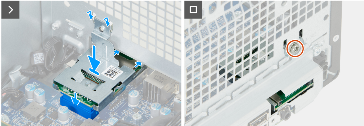
Figure 67. Installing the media-card reader
