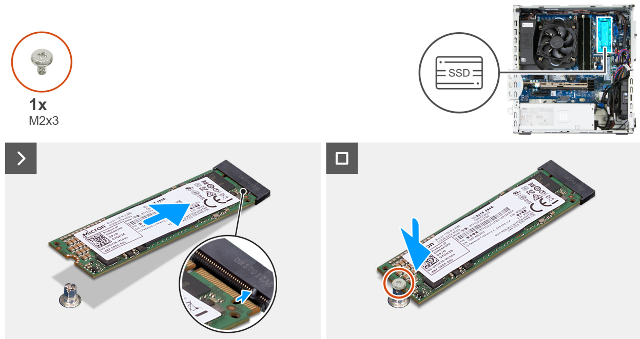
Figure 32. Installing the M.2 2280 solid state drive in slot 2
