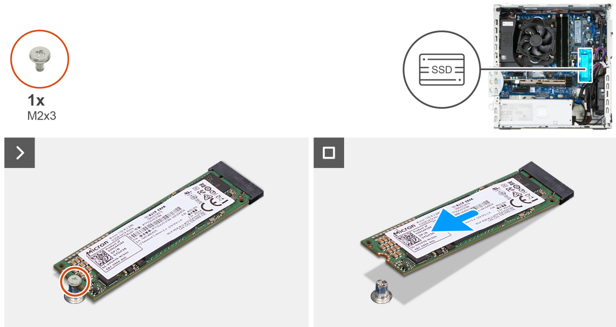
Figure 24. Removing the M.2 2280 solid state drive from slot 0
