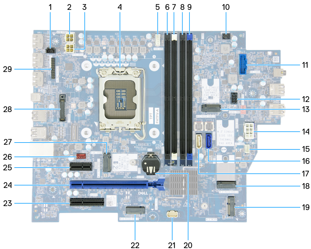
Figure 86. System board overview
