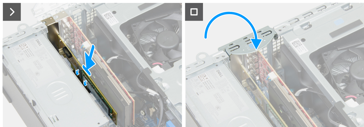
Figure 40. Installing the solid state drive expansion card
