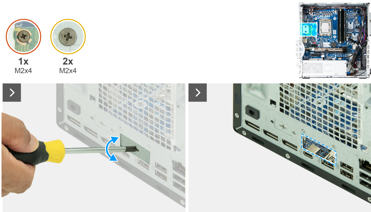
Figure 82. Installing the fiber-optic port module
