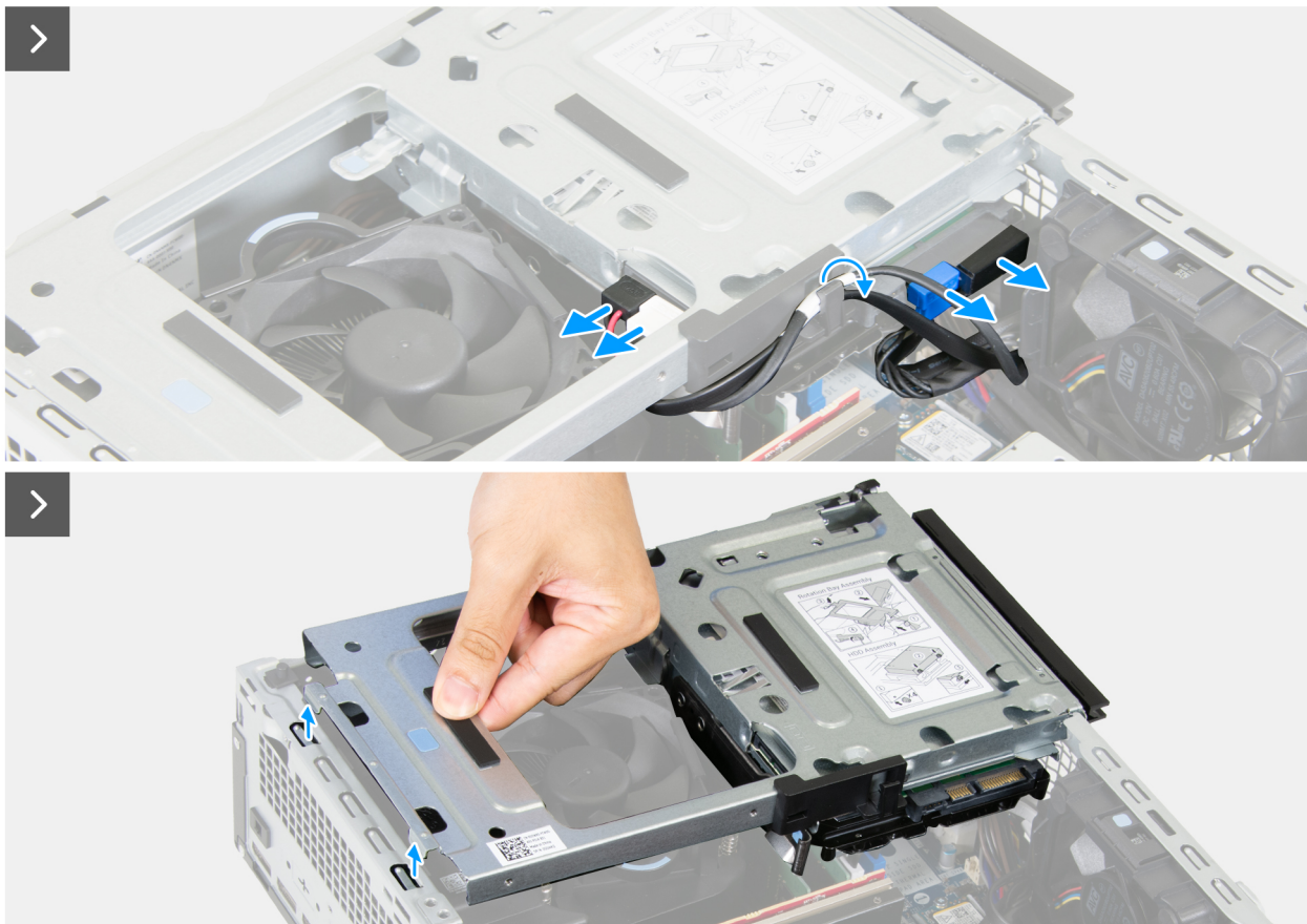
Figure 49. Removing the drive bay
