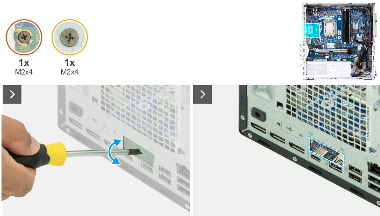
Figure 79. Installing the optional-port module
