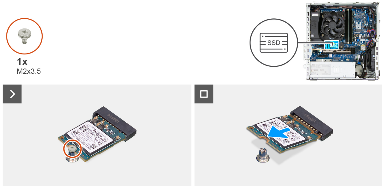
Figure 27. Removing the M.2 2230 solid state drive from slot 1
