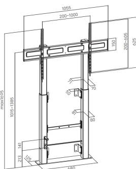
Dimensions (mm)
