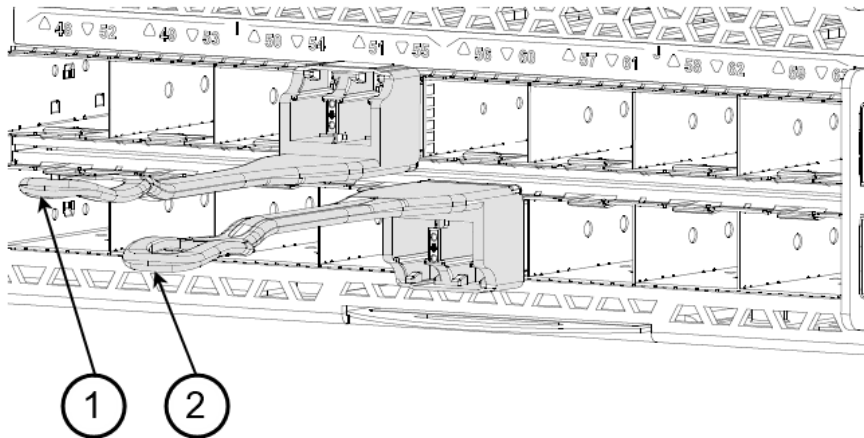
Figure 28: Installing SFP+ Transceivers
