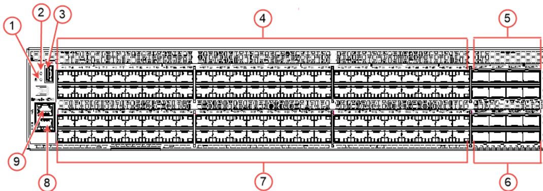
Figure 1: Port-Side View
