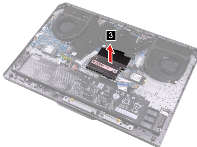
Figure 13. Remove the DIMM shielding
