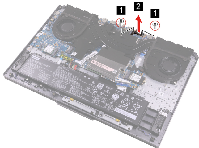
Figure 23. Remove two screws and remove the DC-in bracket
