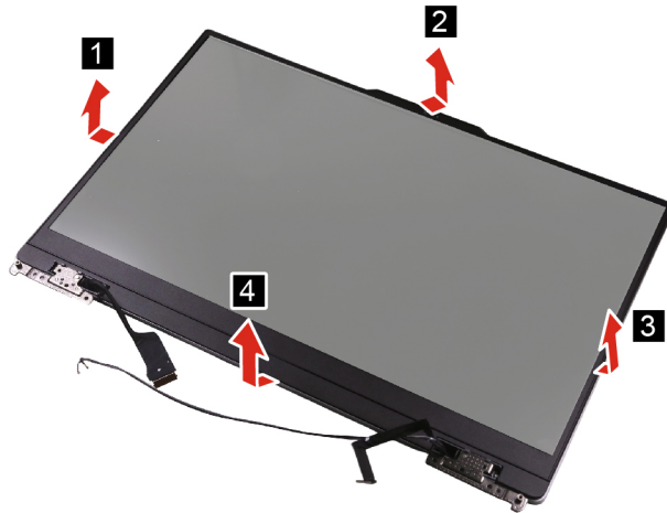
Figure 35. Remove the LCD bezel
