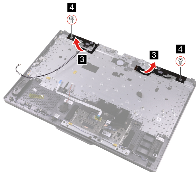
Figure 33. Lift the camera cable and the EDP cable and remove two screws
