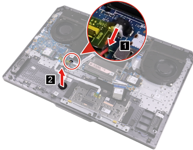
Figure 18. Disconnect the CMOS battery cable and remove the CMOS battery
