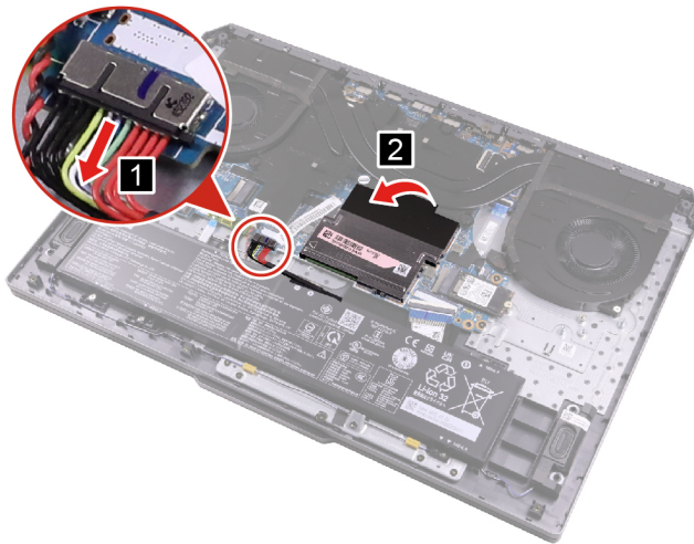
Figure 12. Disconnect the battery pack cable and peel back the mylar
