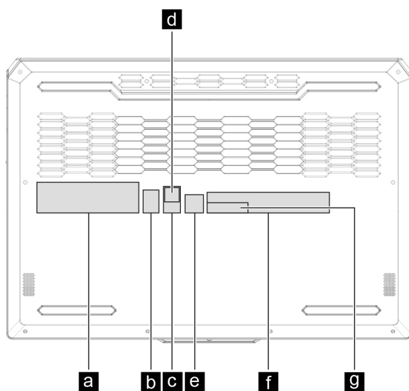
Figure 48. EAA: Label layout on the back side of the base cover
