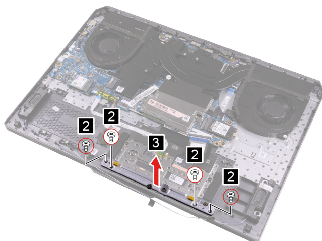
Figure 20. Remove four screws and remove the touchpad bracket
