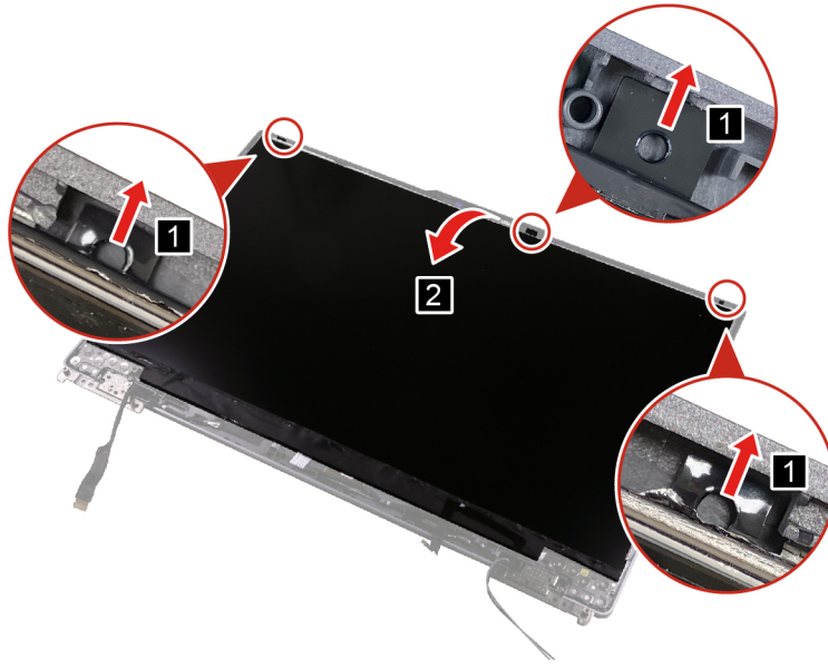
Figure 36. Pull out three pieces of the removable tape and turn over the LCD panel
