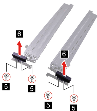
Figure 40. Remove four screws and remove the hinge caps
