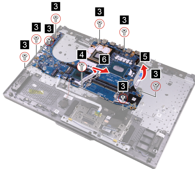
Figure 29. Remove nine screws, lift the I/O cable, and remove the system board
