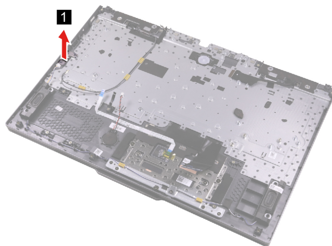
Figure 31. Remove the Type-C bracket
