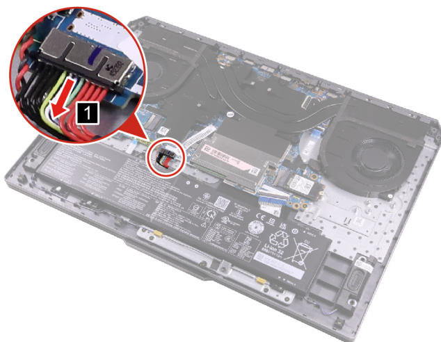
Figure 7. Disconnect the battery pack cable
