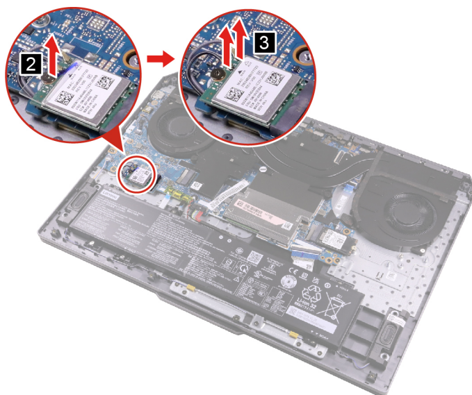
Figure 8. Remove the Wi-Fi mylar and disconnect the antennas from the Wi-Fi card
