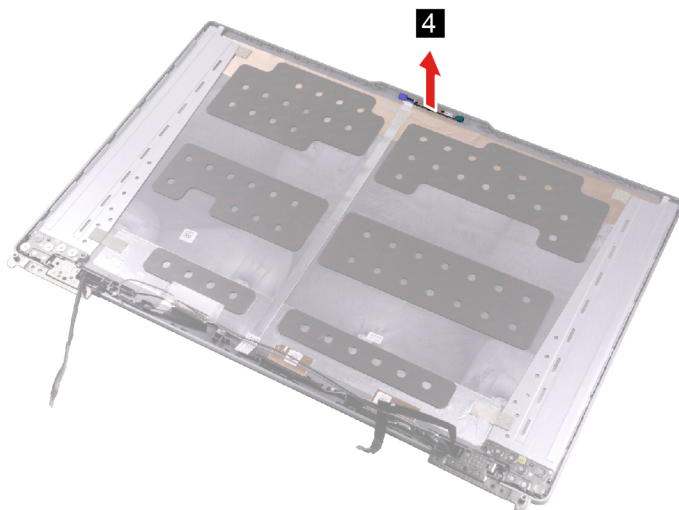
Figure 45. Remove the camera board
