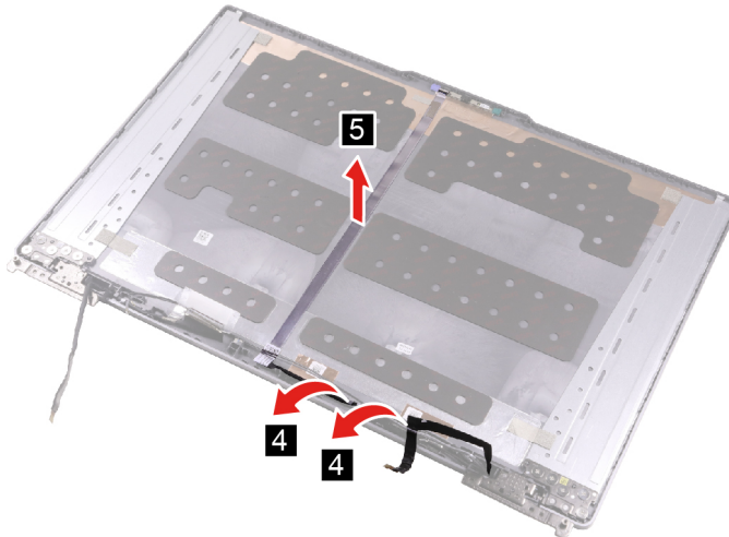
Figure 43. Release and remove the camera cable
