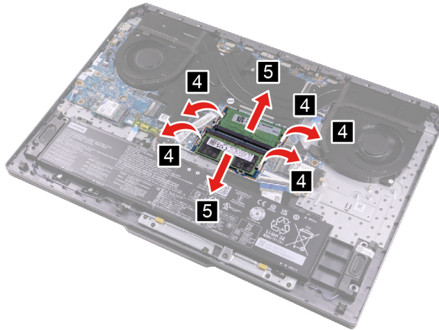
Figure 14. Open the latches and remove the memory module
