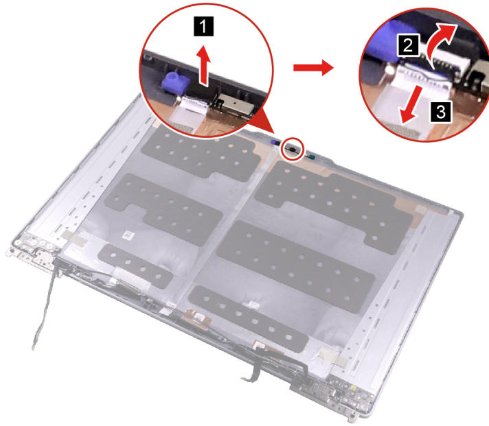
Figure 42. Remove the camera sponge and disconnect the camera cable
