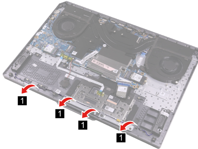
Figure 21. Release the speakers cable from the cable guide
