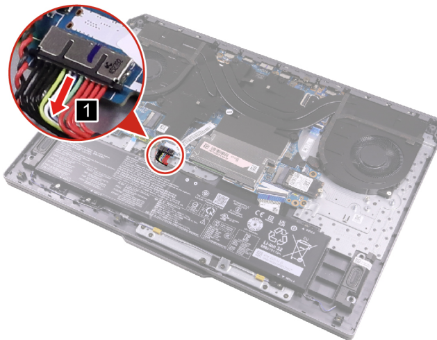
Figure 15. Disconnect the battery pack cable
