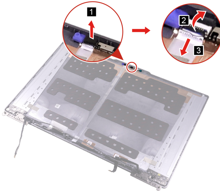
Figure 44. Remove the camera sponge and disconnect the camera cable
