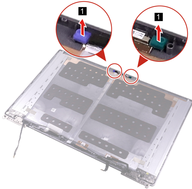
Figure 46. Remove the microphone rubbers
