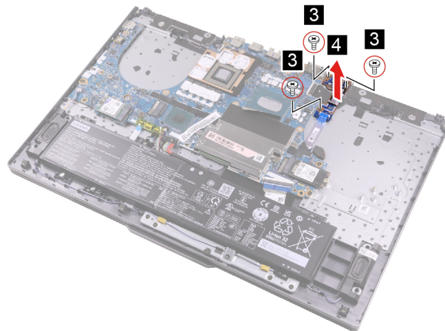
Figure 27. Remove three screws and remove the I/O board
