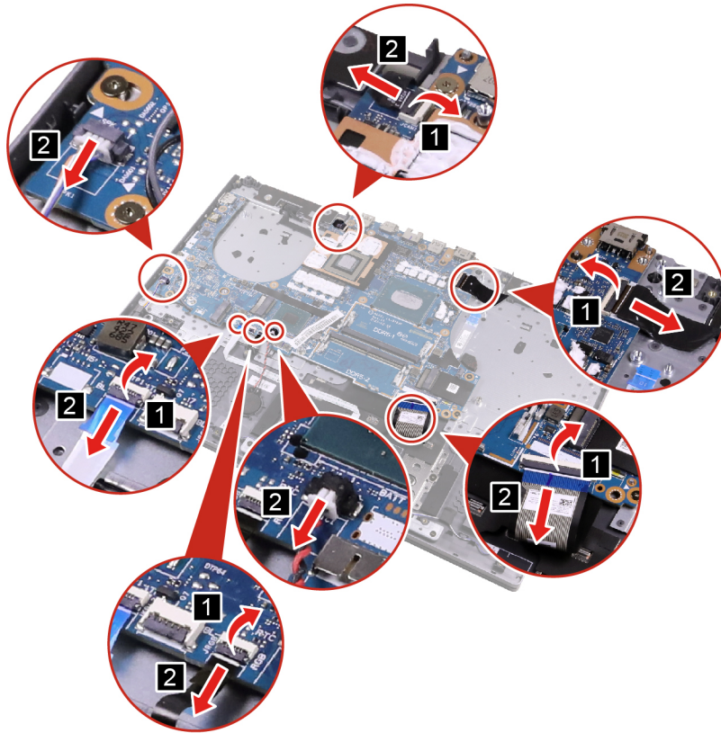
Figure 28. Disconnect all the cables
