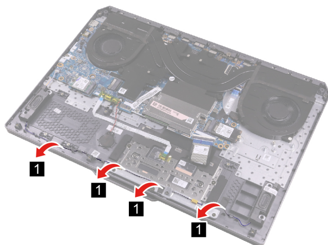
Figure 19. Release the speakers cable from the cable guide
