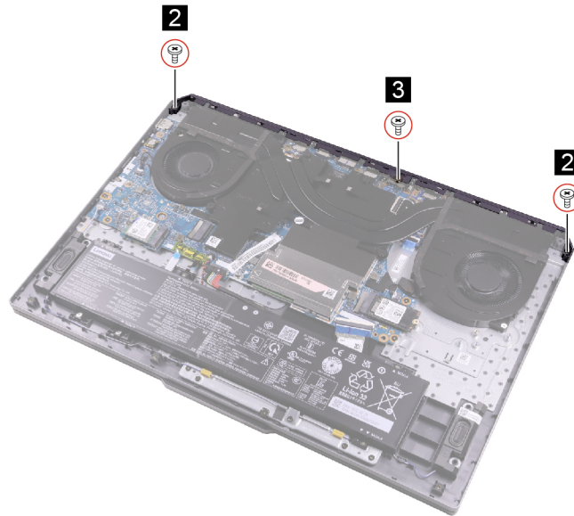
Figure 16. Remove three screws
