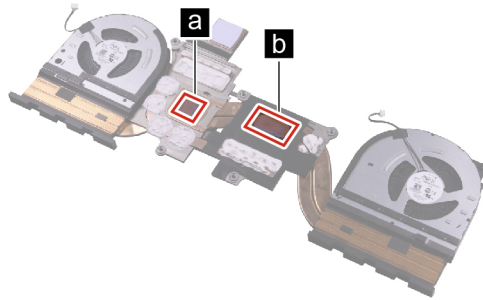
Figure 3. Areas on the thermal module where thermal interface materials should be applied
