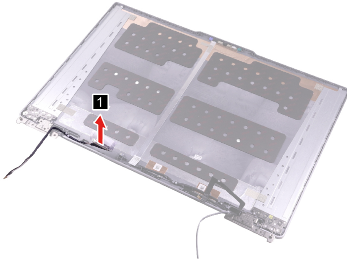
Figure 41. Remove the EDP cable
