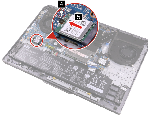
Figure 9. Remove one screw and the Wi-Fi card
