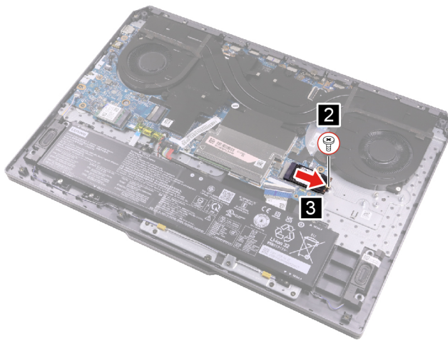
Figure 11. Remove one screw and remove the 2242 solid-state drive
