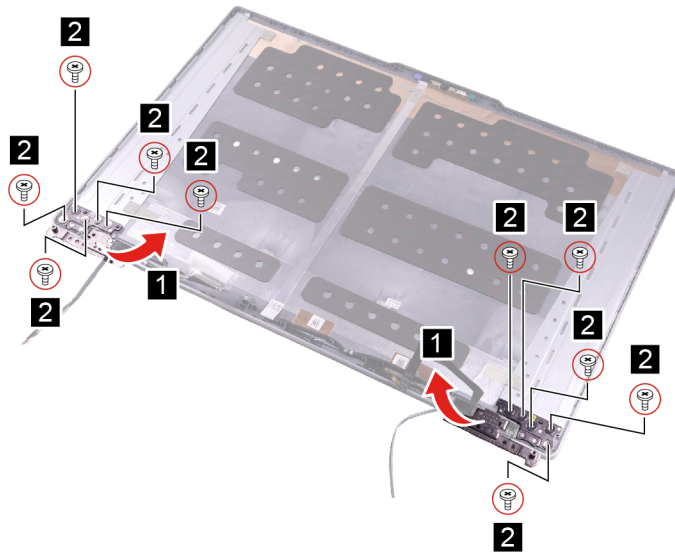
Figure 38. Release the EDP cable and the camera cable and remove ten screws
