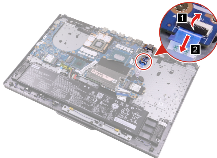
Figure 26. Disconnect I/O cable from the I/O board
