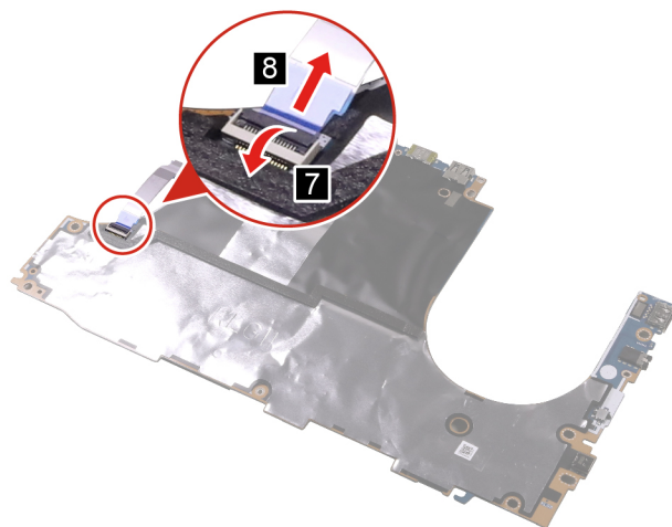
Figure 30. Remove the I/O cable
