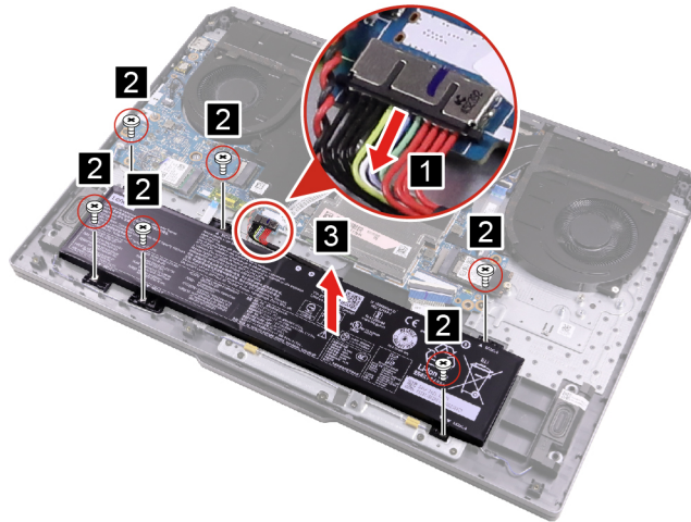
Figure 6. Remove six screws and the battery pack
