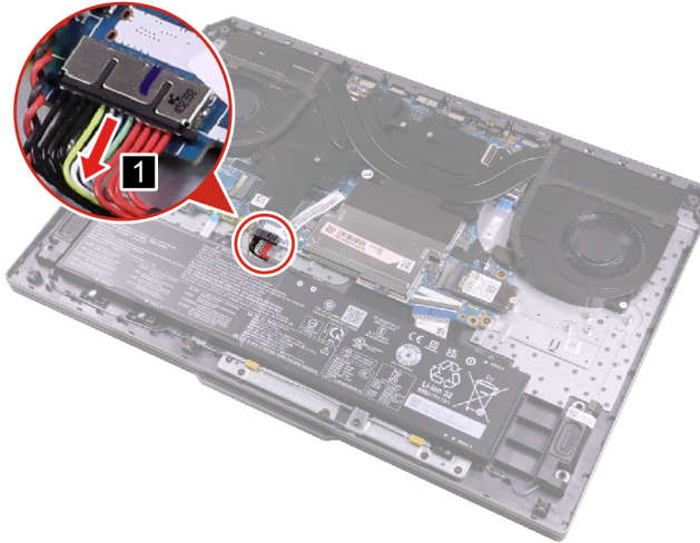
Figure 10. Disconnect the battery pack cable
