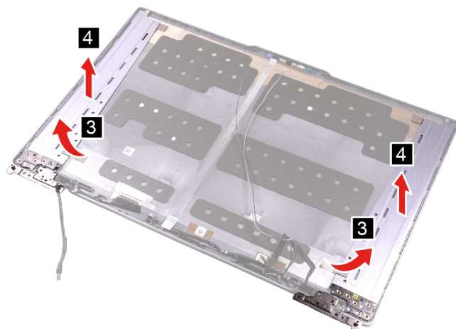
Figure 39. Lift the tape and remove the hinges from the LCD cover
