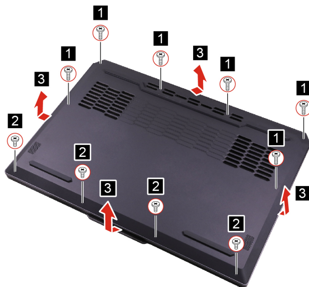
Figure 5. Remove ten screws and the lower case
