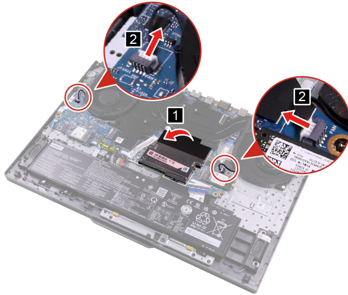
Figure 24. Peel back the mylar and disconnect the fan cables
