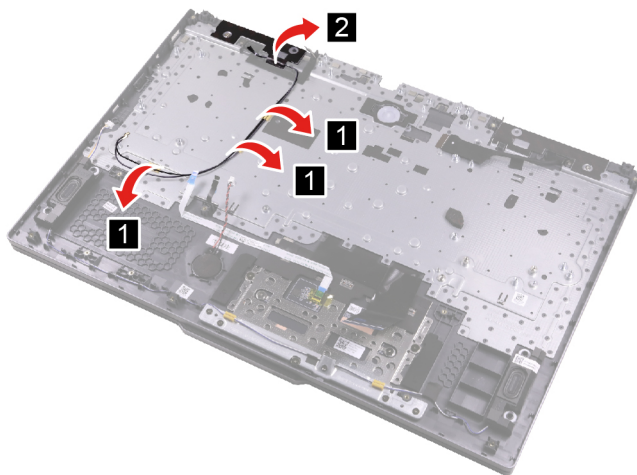
Figure 32. Remove the Wi-Fi antennas from the cable guide and peel back the tape
