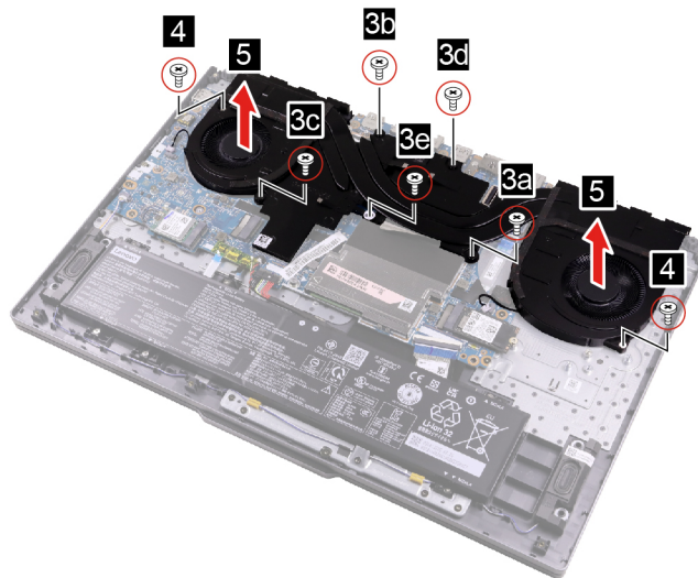
Figure 25. Loosen five heat sink screws, remove two fan screws, and remove the thermal module
