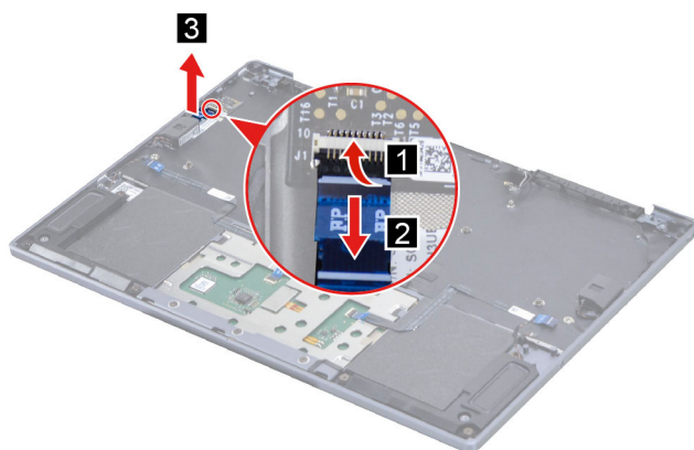
Figure 28. Remove the fingerprint board cable
