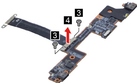
Figure 25. Remove the IO board cable (down)
