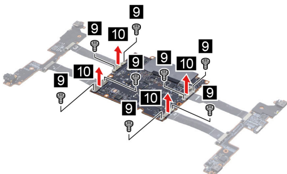
Figure 23. Remove the system board
