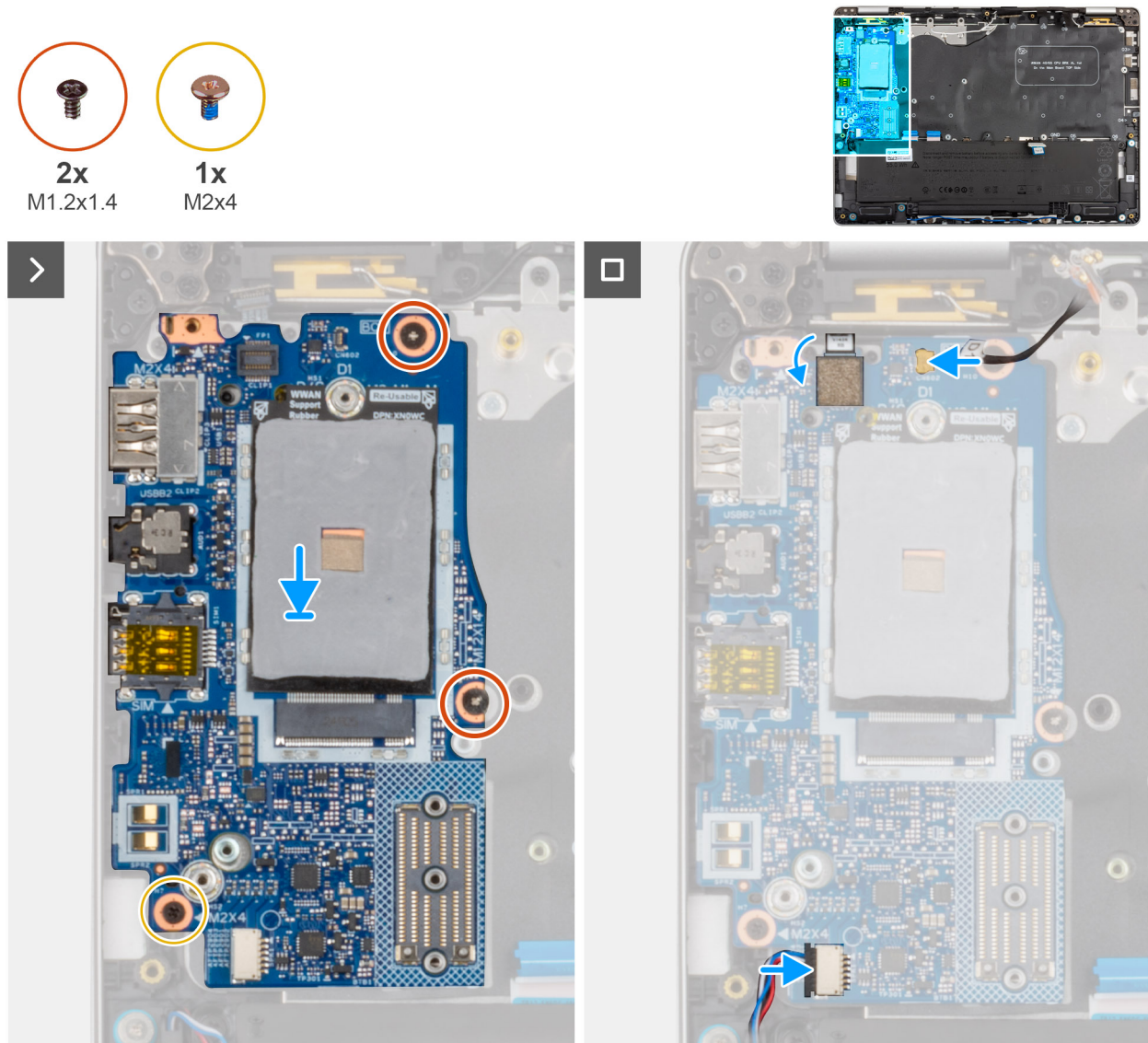
Figure 63. Installing the I/O board
