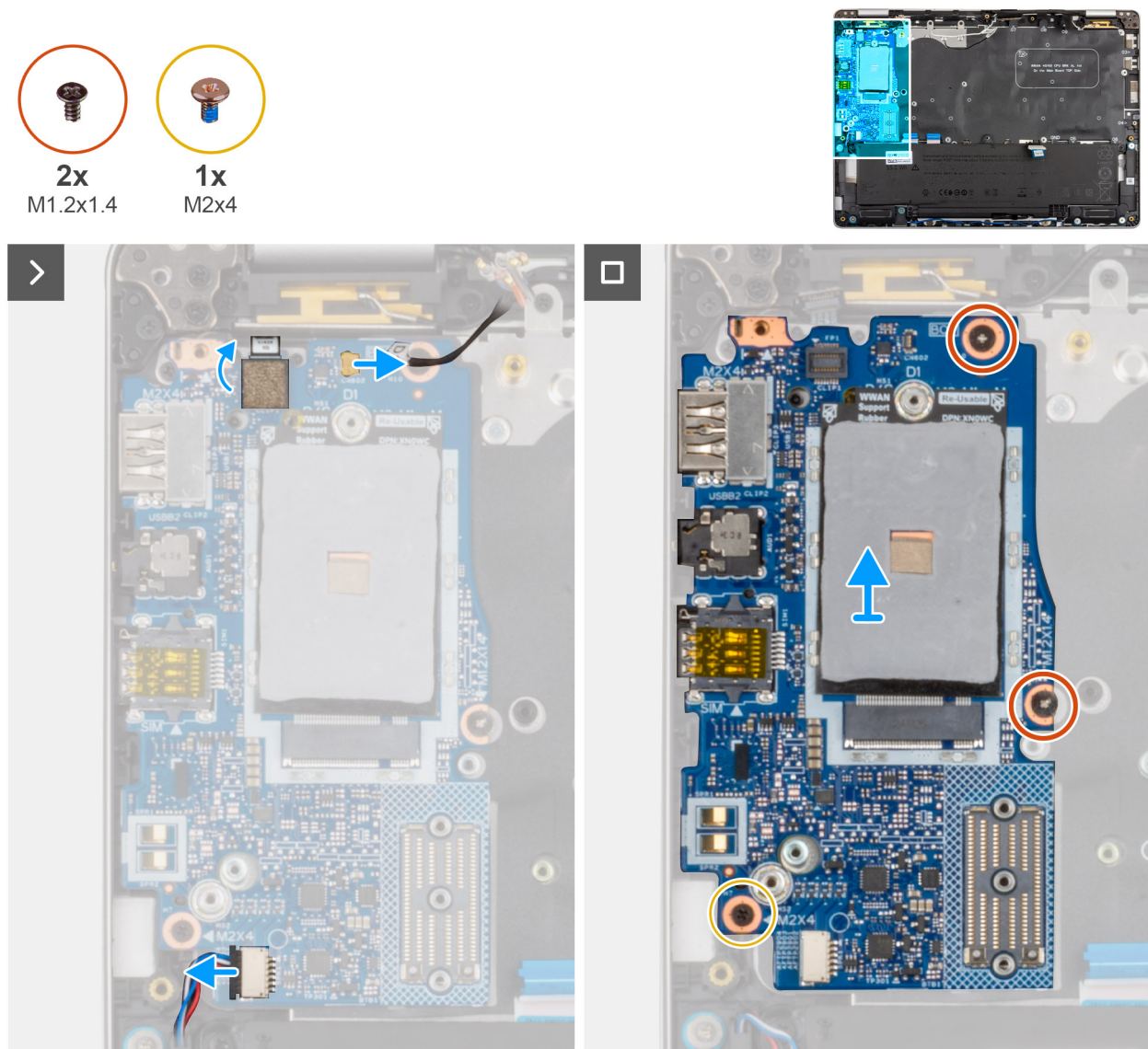
Figure 62. Image: Removing the I/O board
