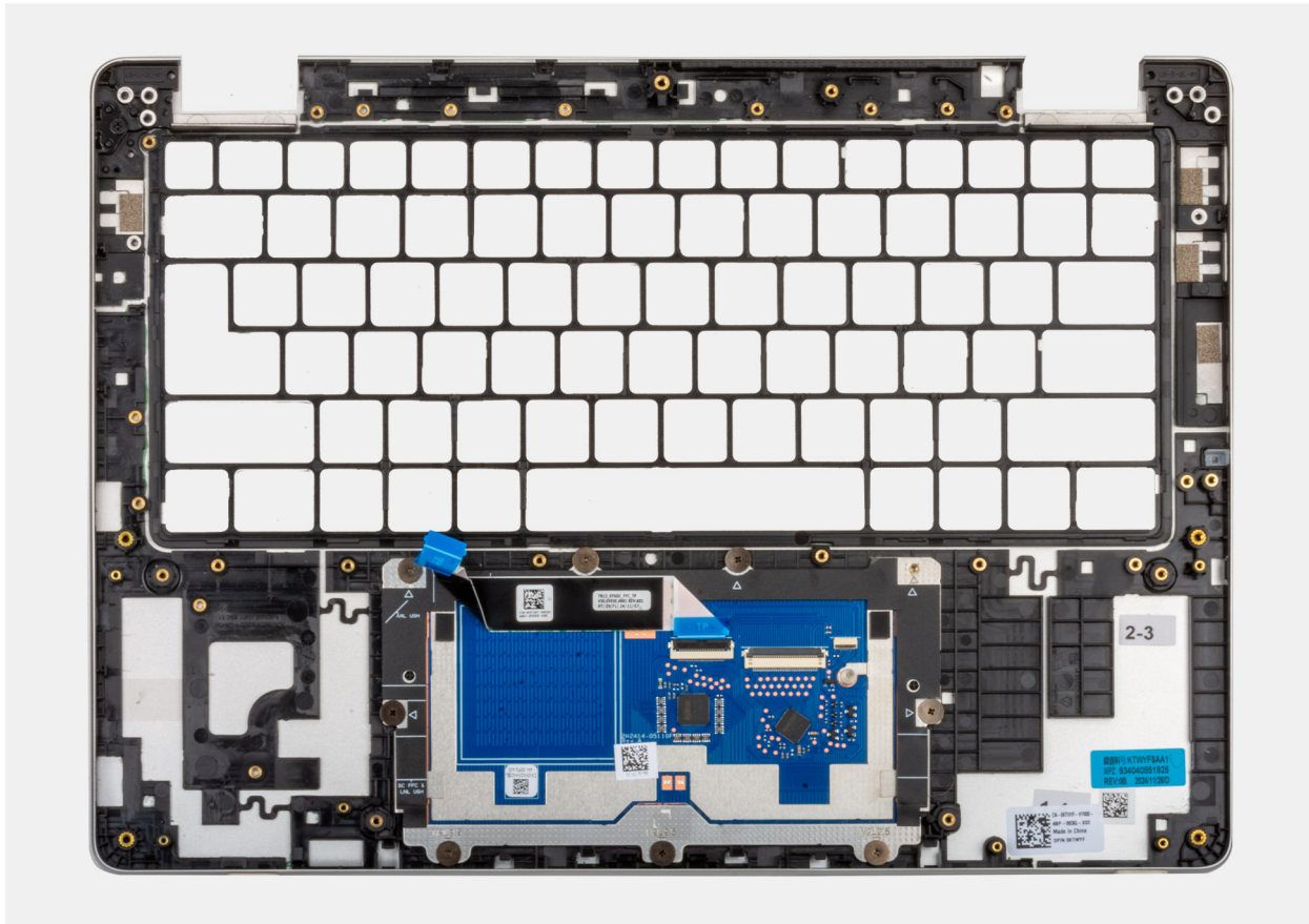
Figure 70. Removing the palm-rest assembly
