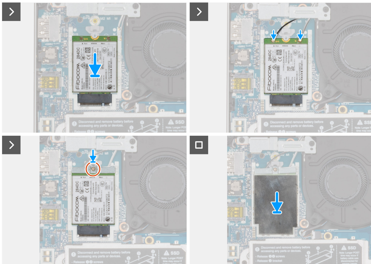
Figure 32. Installing the 5G WWAN card
