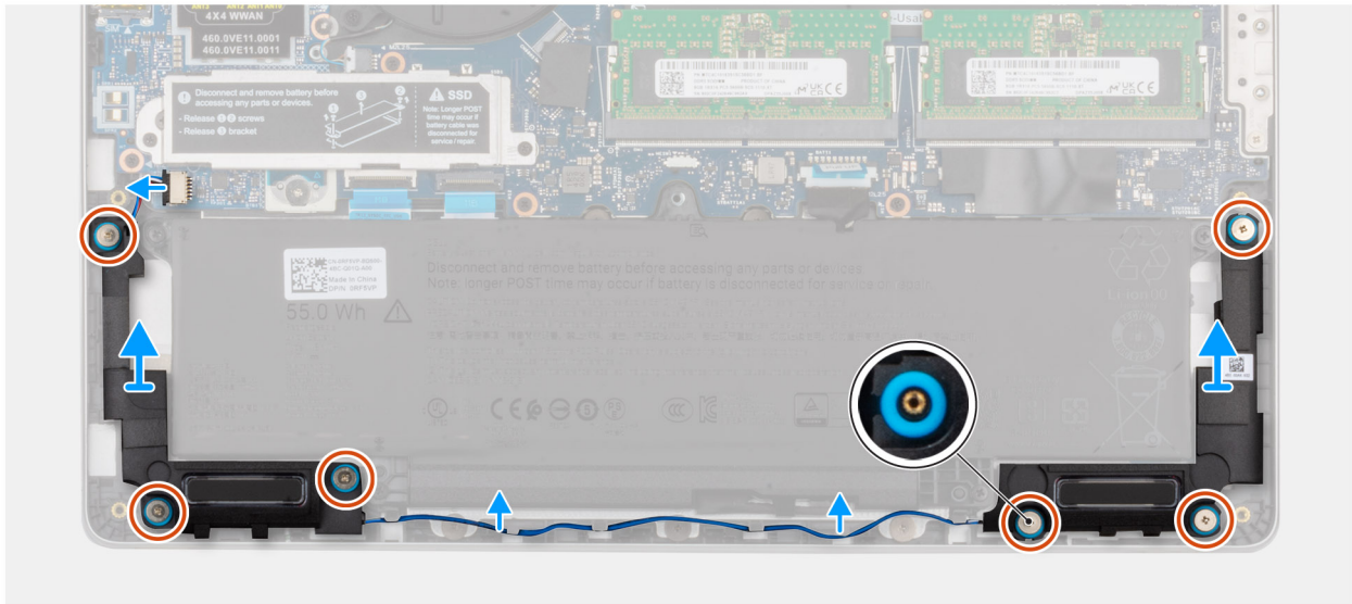
Figure 39. Removing the speakers
