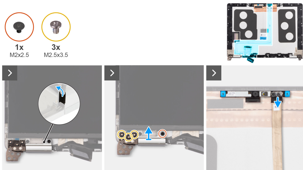
Figure 80. Removing the display cable
