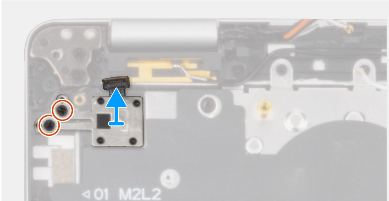
Figure 64. Removing the power button with an optional fingerprint reader
