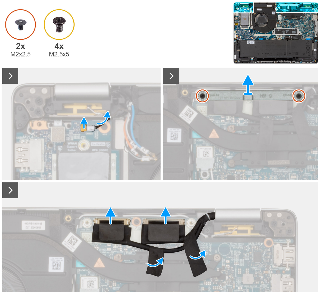
Figure 50. Removing the display assembly
