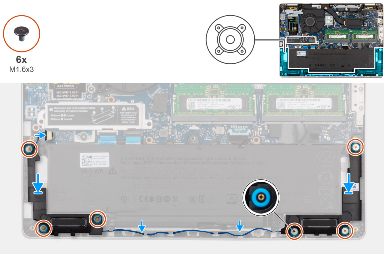
Figure 40. Installing the speakers
