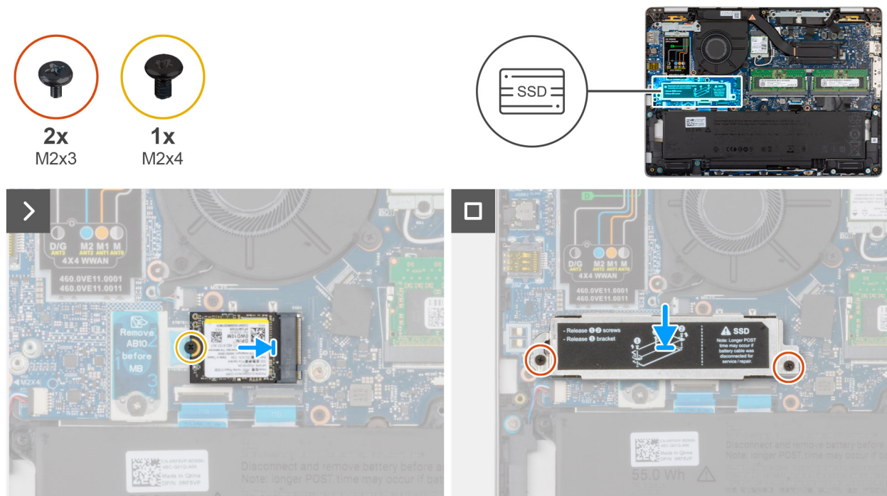
Figure 36. Installing the M.2 2230 SSD
