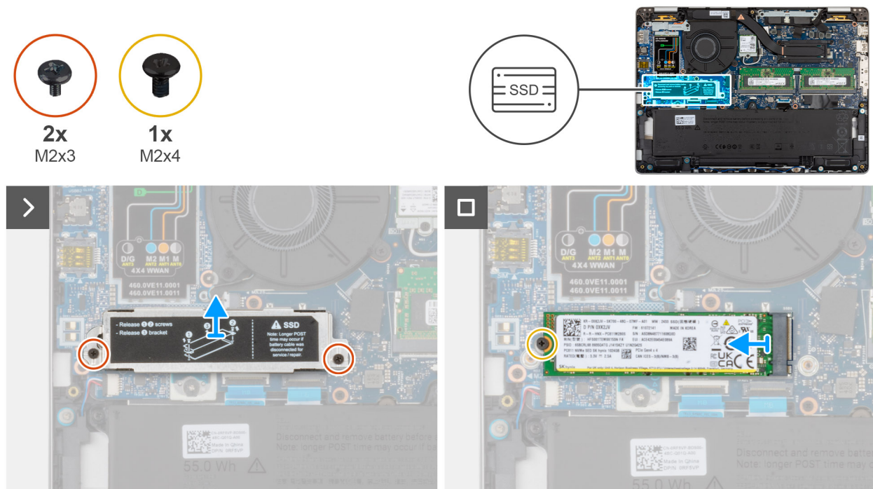
Figure 37. Removing the M.2 2280 SSD
