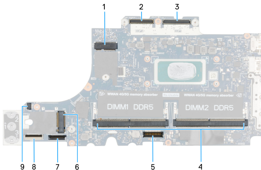
Figure 54. System board connectors
