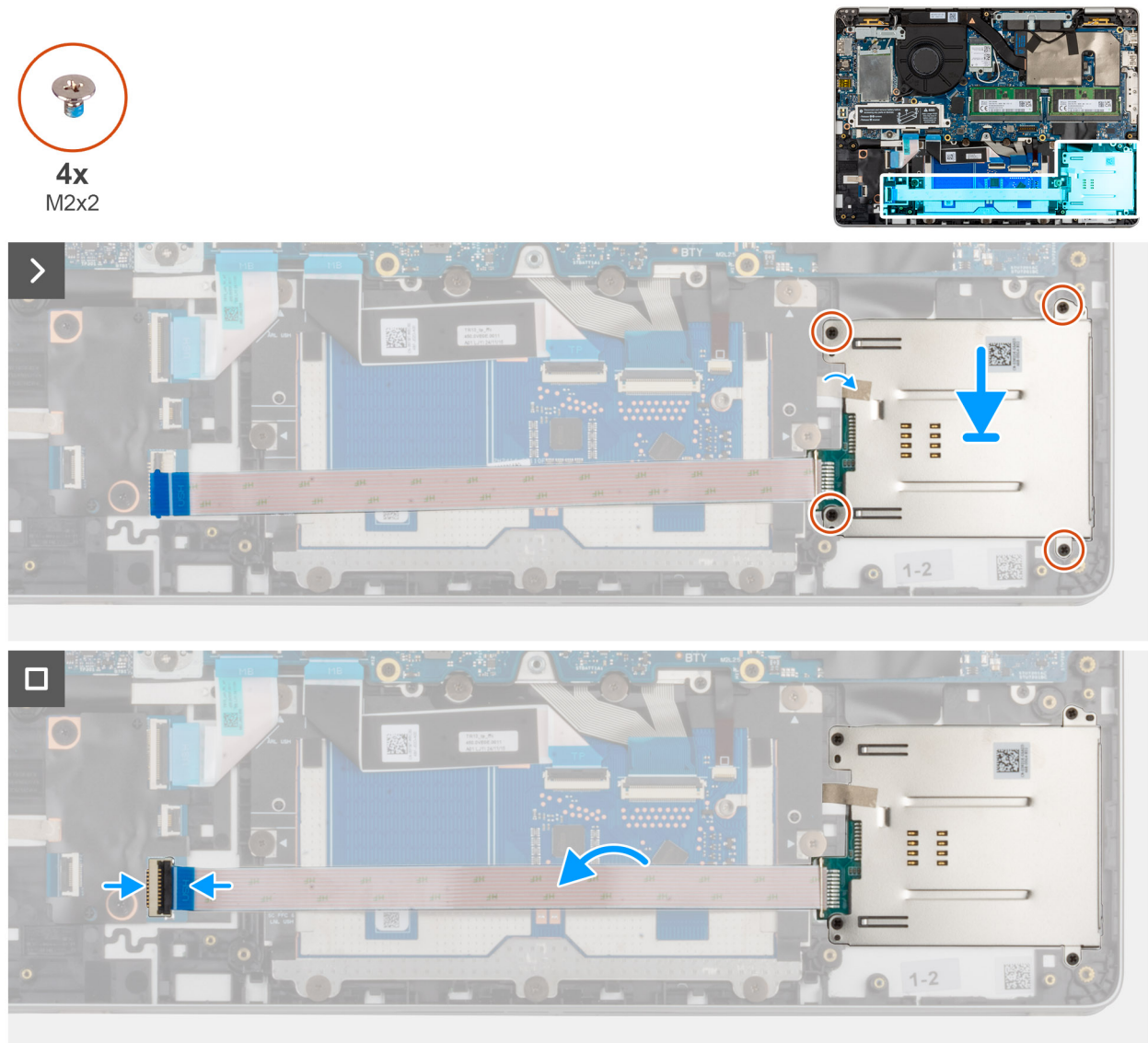
Figure 47. Installing the Smart card reader
