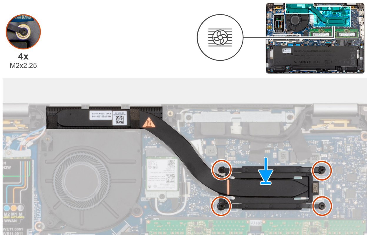
Figure 49. Installing the heat sink
