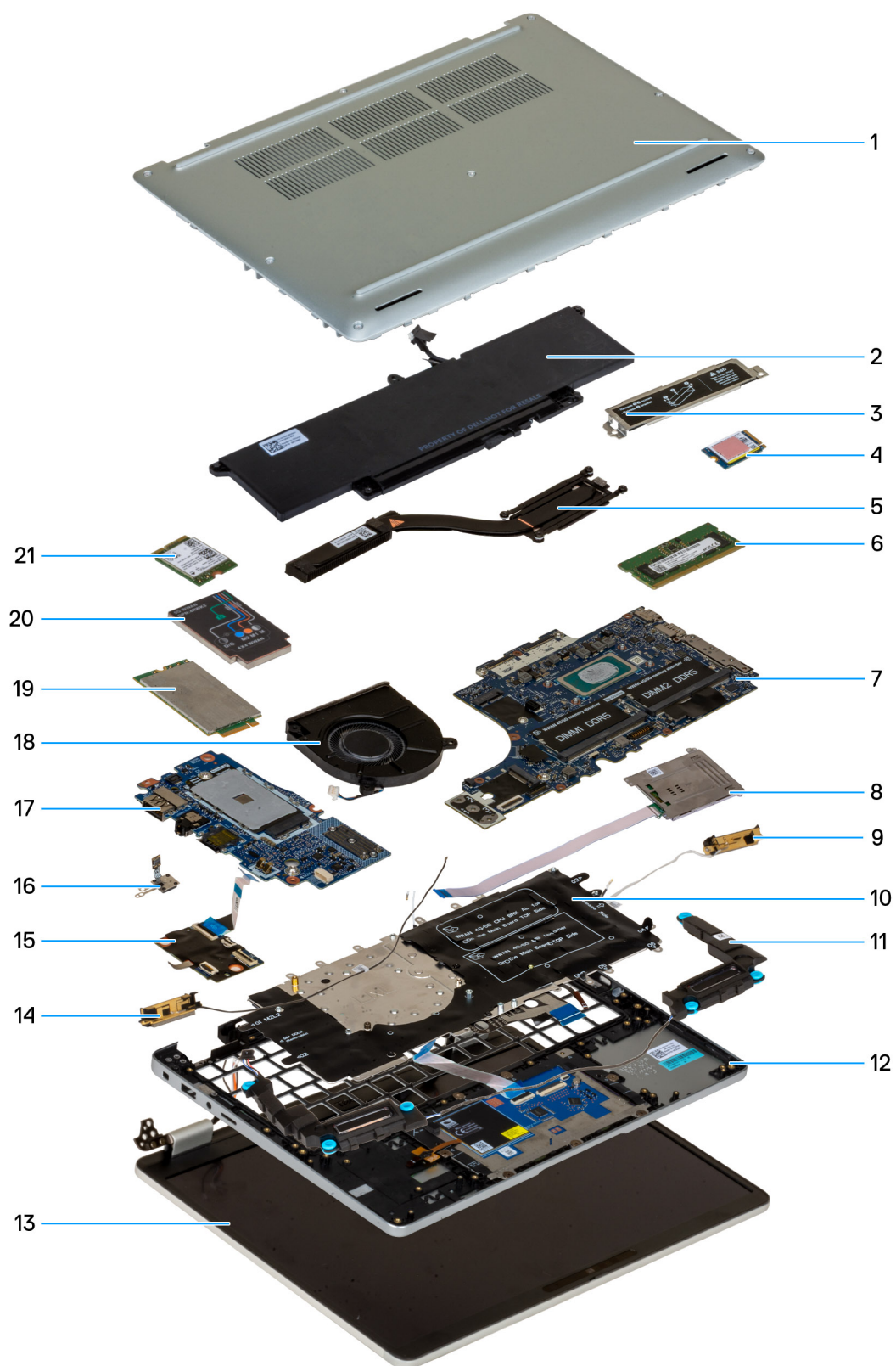
Figure 14. Major Components of your Dell Pro 13 Plus
