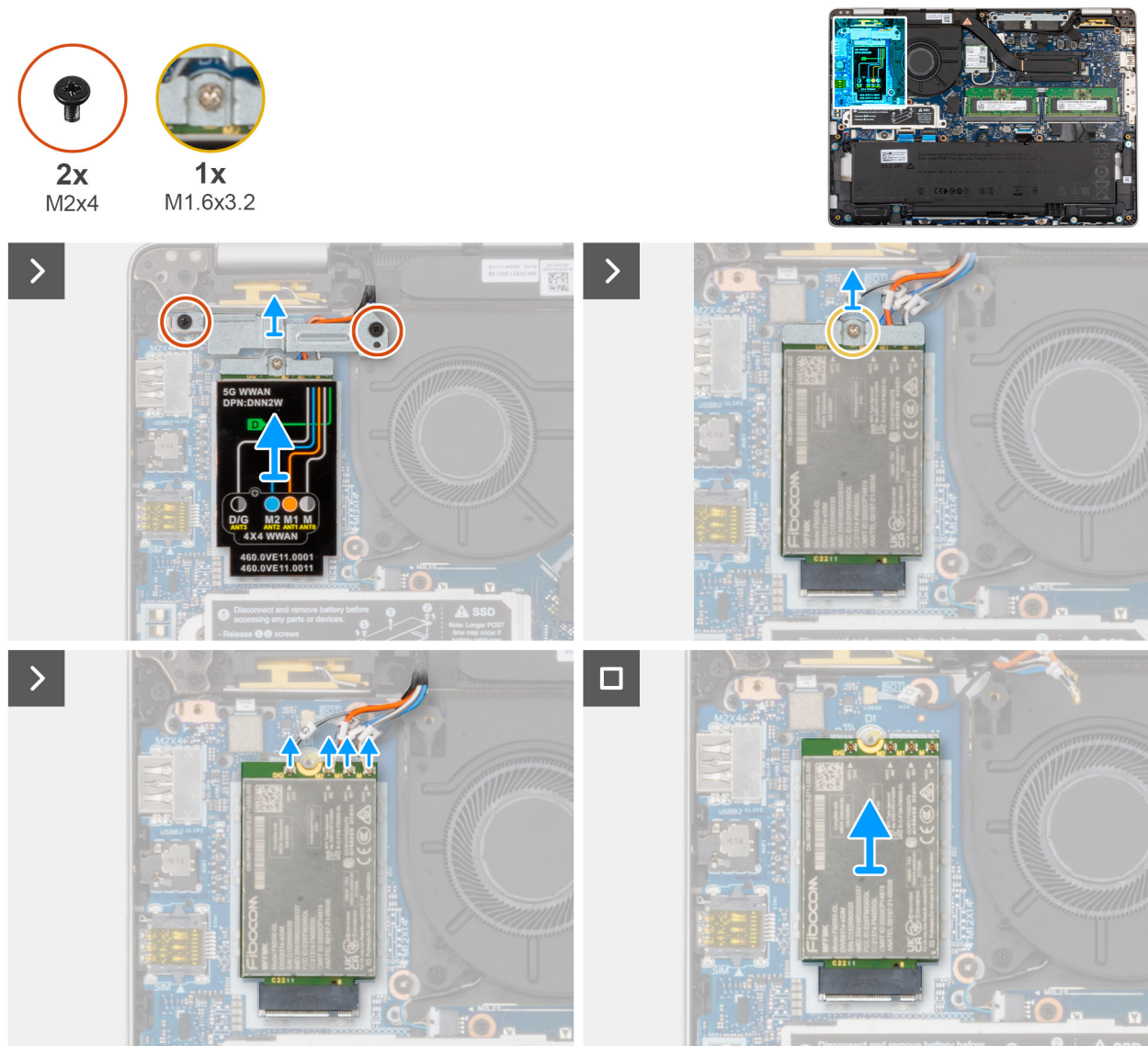
Figure 29. Removing the 5G WWAN card
