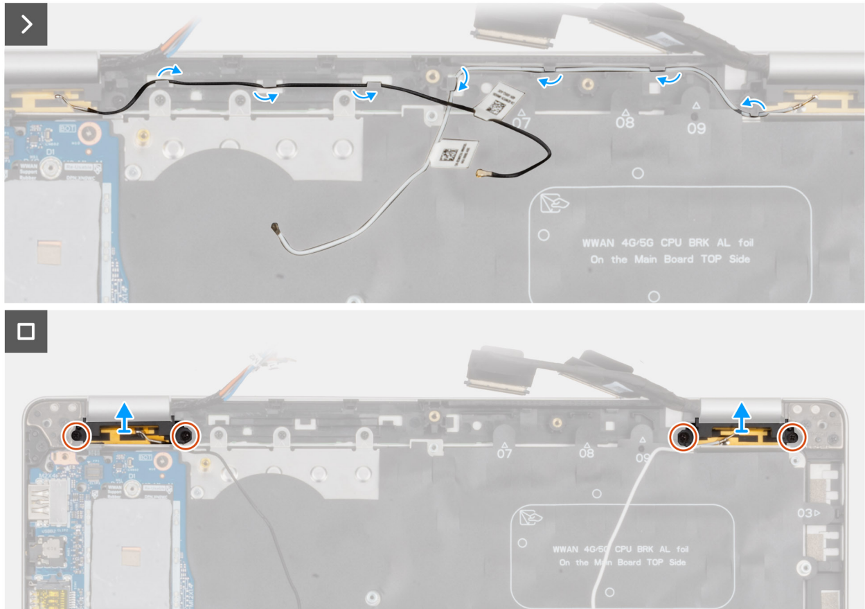
Figure 60. Removing the wireless antenna module
