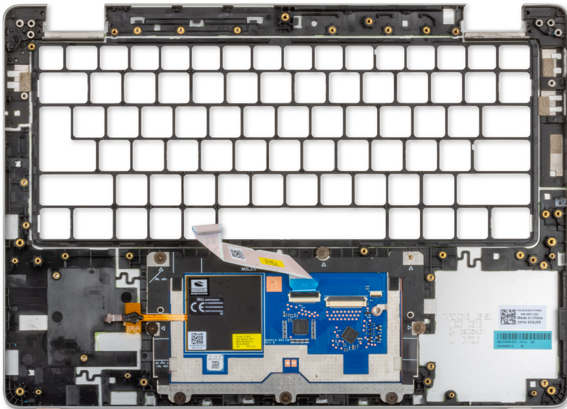
Figure 71. Installing the palm-rest assembly
