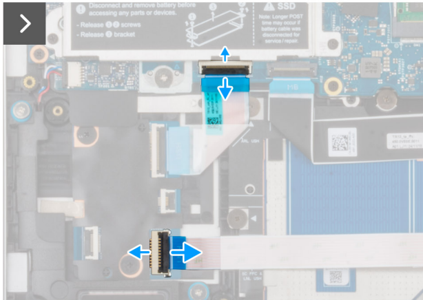
Figure 43. Removing the USH board
