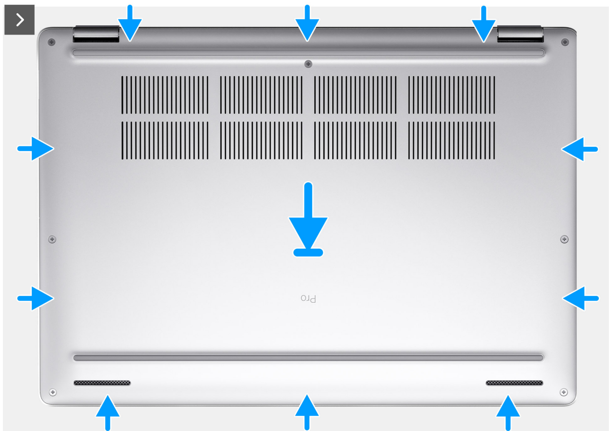
Figure 21. Installing the base cover
