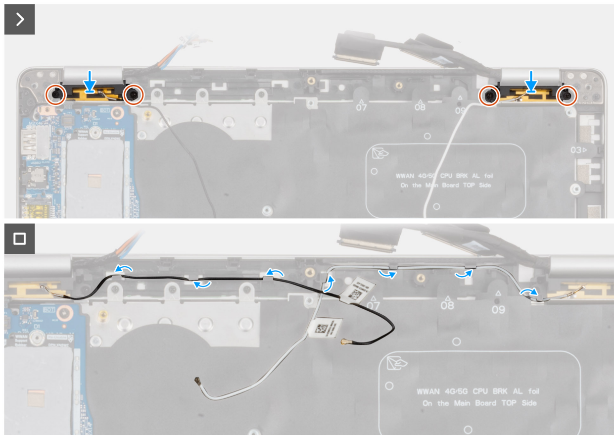
Figure 61. Installing the WLAN antenna module
