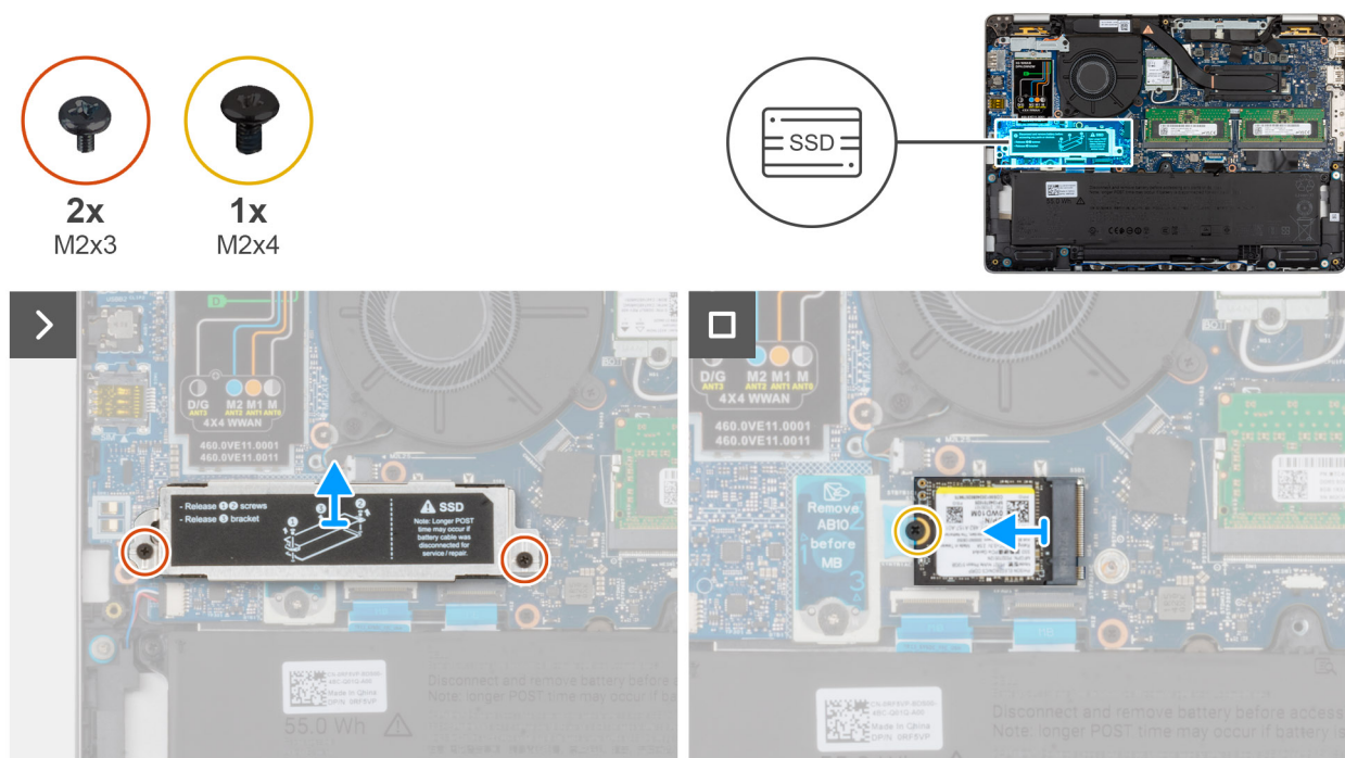
Figure 35. Removing the M.2 2230 SSD
