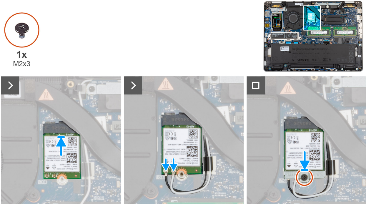
Figure 34. Installing the WLAN card
