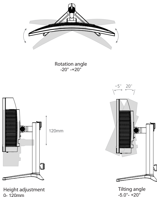
Figure 2-1 Angle Adjustment
