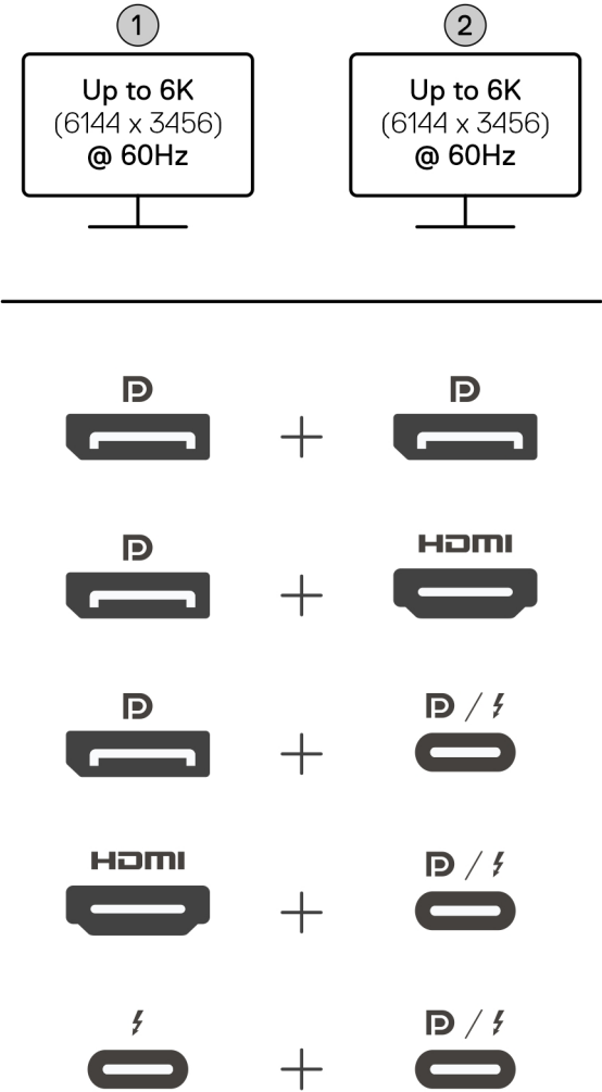
Figure 7. Dual-display setup
