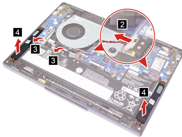
Figure 18. Disconnect the speakers cable and remove the speakers
