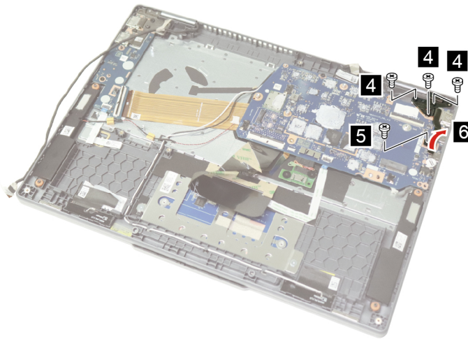
Figure 34. Remove four screws and open the right hinge
