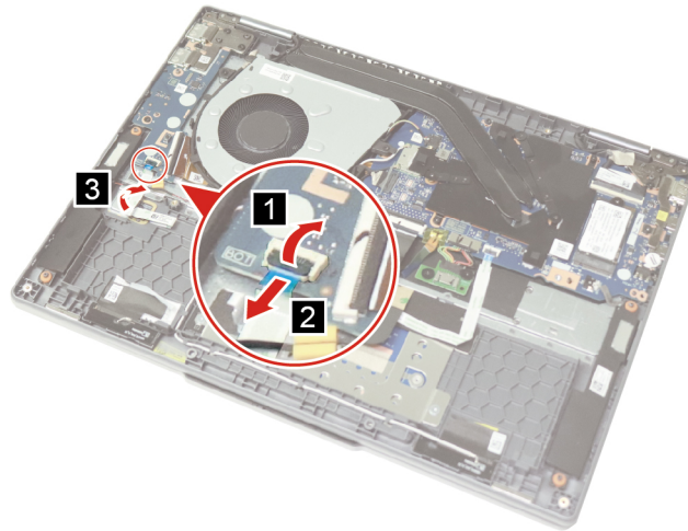
Figure 21. Disconnect and peel back the fingerprint cable
