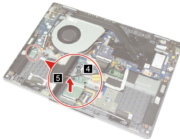
Figure 22. Remove one screw and the fingerprint bracket
