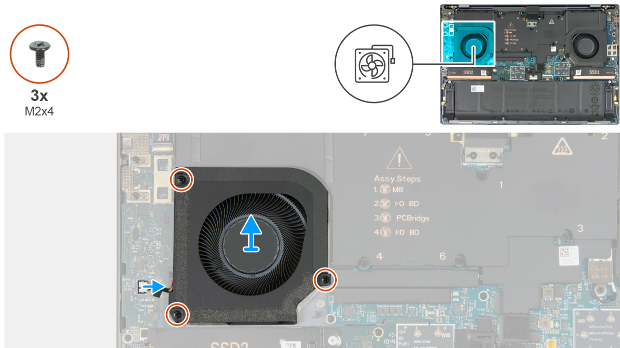
Figure 32. Removing the right fan
