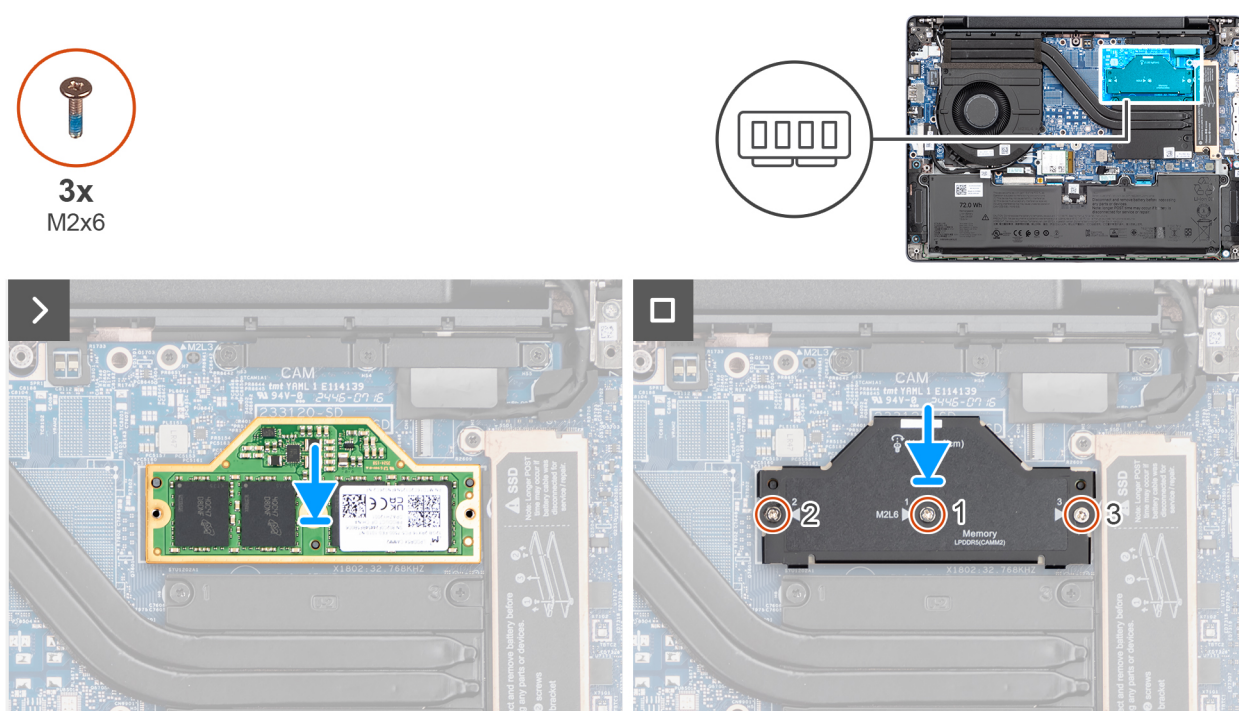
Figur 21. Installera minnesmodulen
