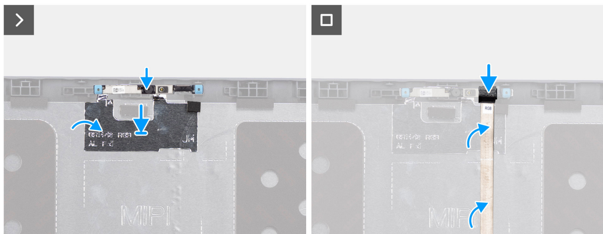
Figur 71. Installera kameran
