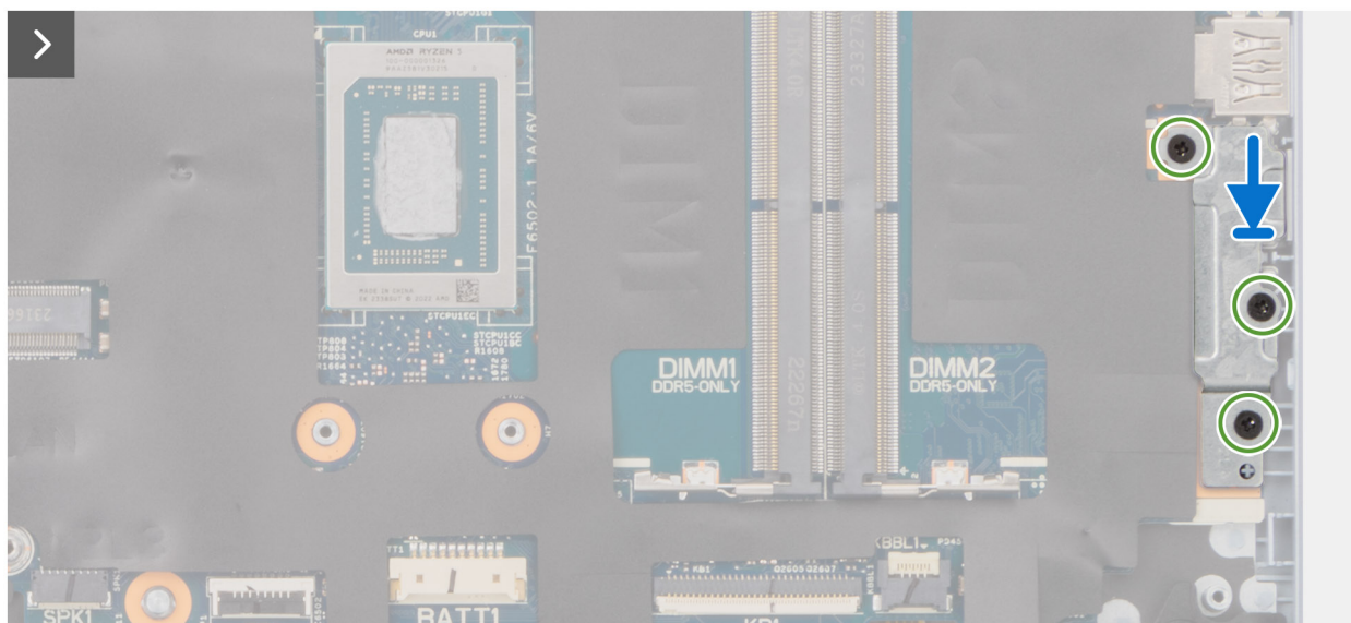
Figure 84. Installing the system board (for computers shipped with a plastic chassis)
