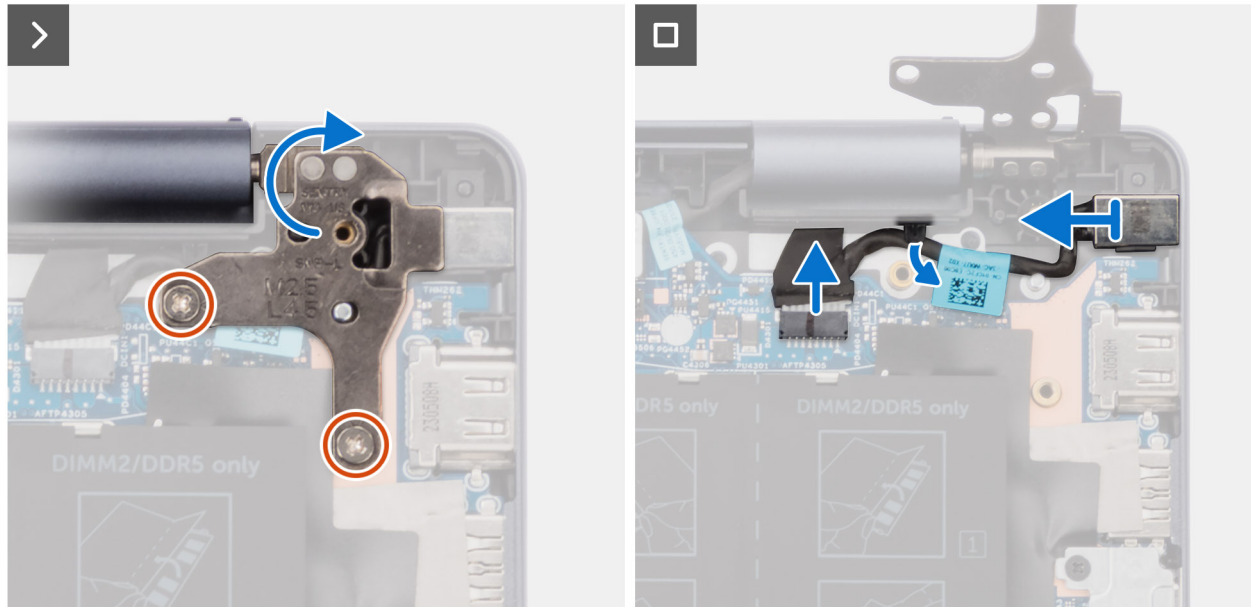
Figure 38. Removing the power-adaptor port (for computers shipped with an aluminum chassis)
