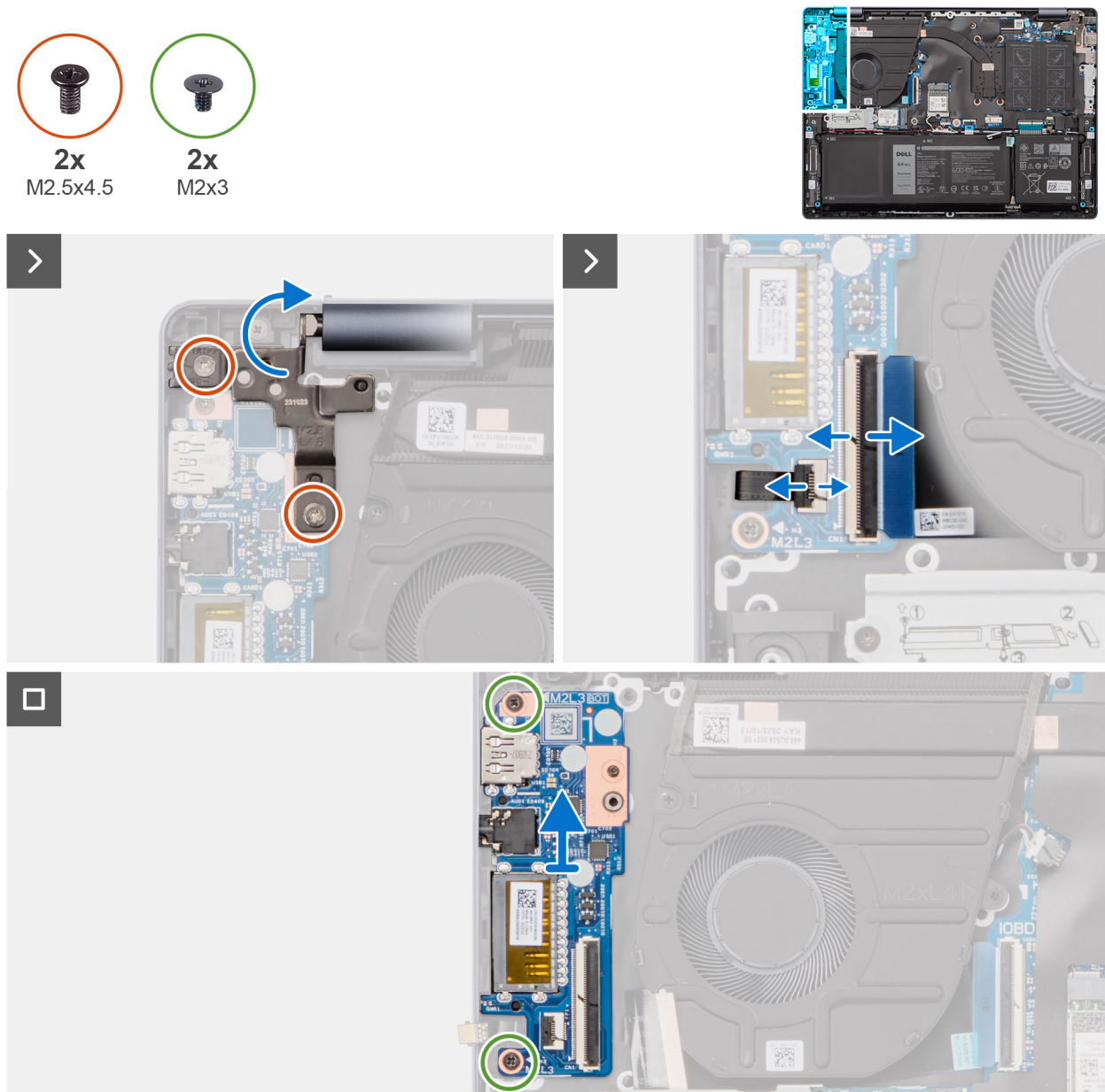
Figure 44. Removing the I/O board (for computers shipped with an aluminum chassis)
