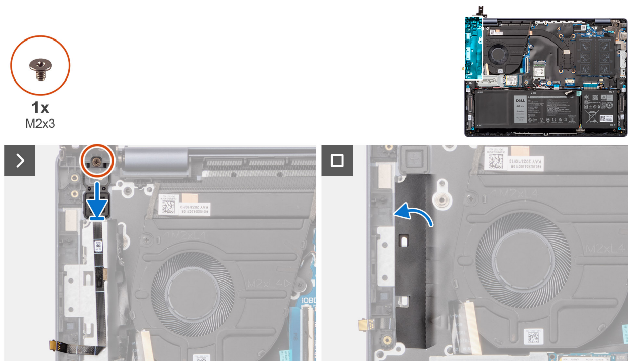
Figure 50. Installing the power button with the optional fingerprint reader
