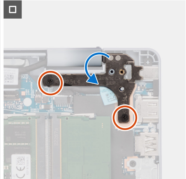
Figure 39. Installing the power-adaptor port (for computers shipped with a plastic chassis)
