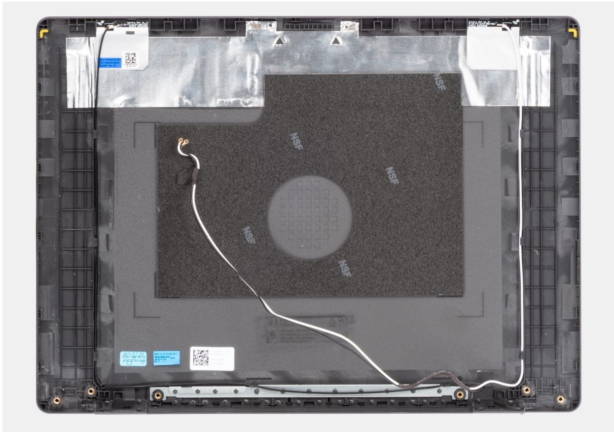
Figure 76. Display back-cover and antenna assembly
