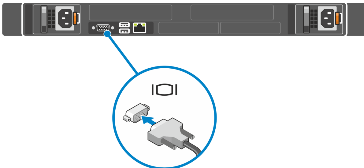
Figure 8. Display port
