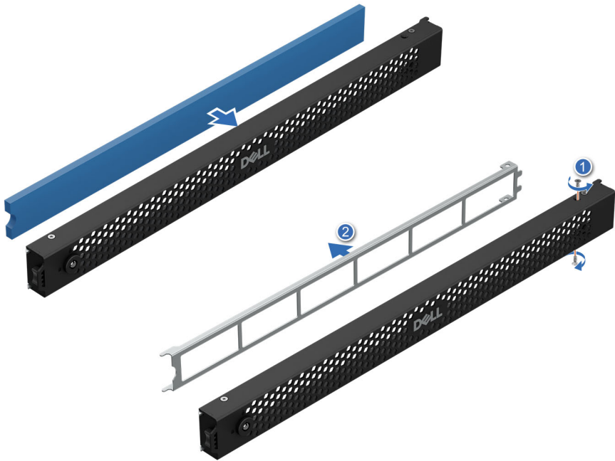
Figure 98. Installation du filtre
