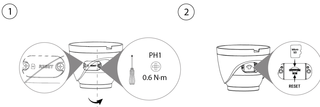
Figure 4-2 Install the SD card
