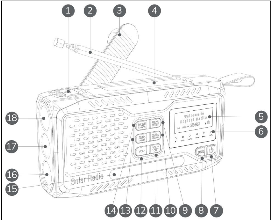
Figure 1: Front view.
