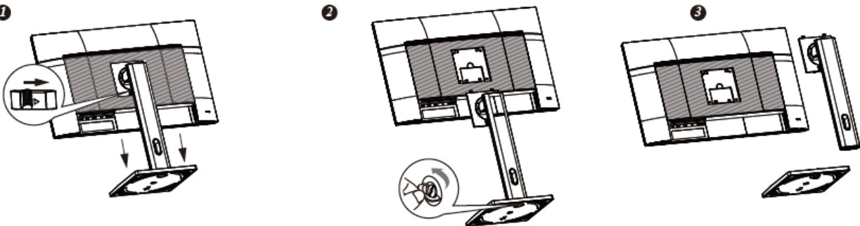
Figure.1. Installing and Removing the Base
