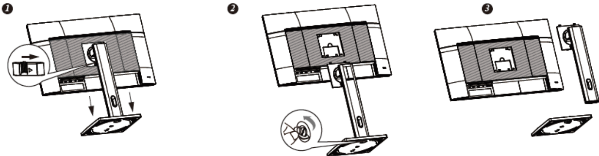
Figure.1. Installing and Removing the Base
