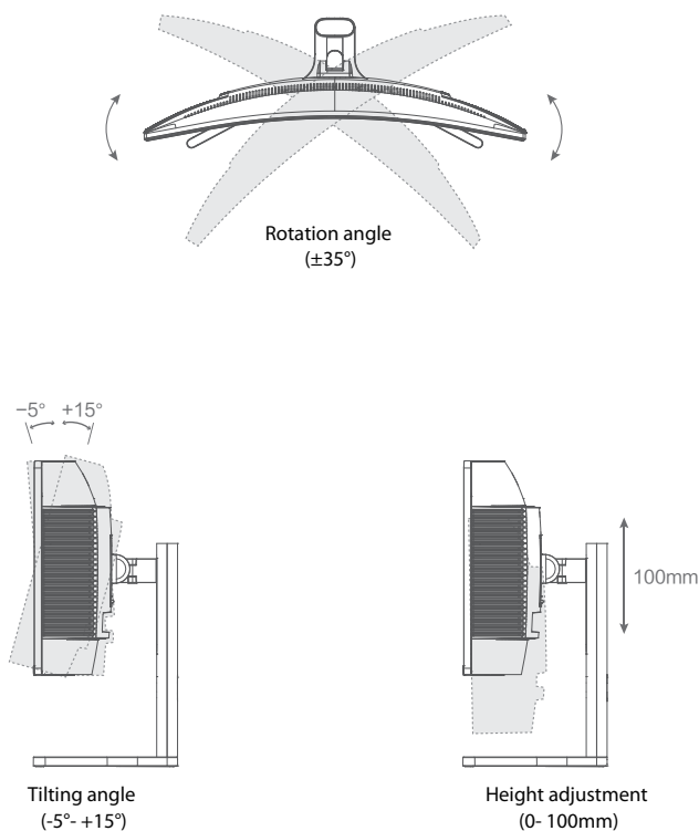
Figure 2-1 Angle Adjustment
