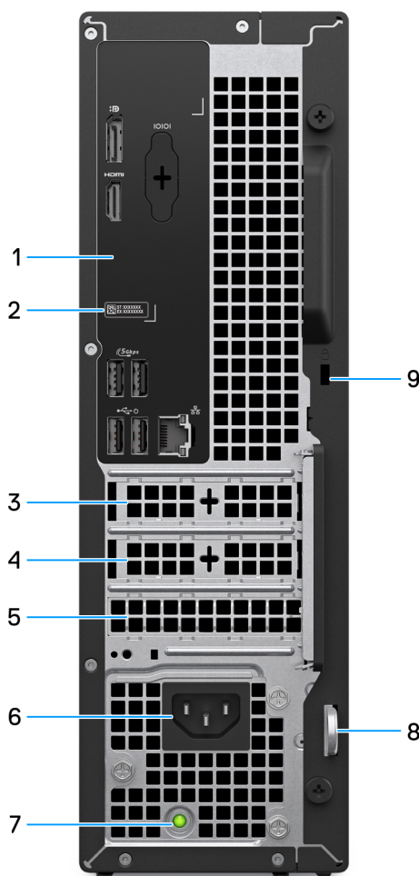
Figure 2. Vue arrière de Dell Pro Slim Essential QVS1260
