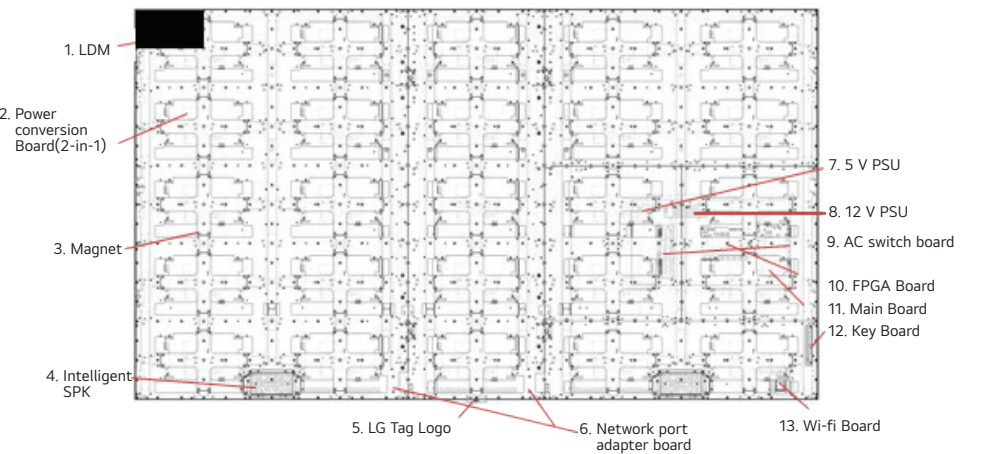
Figure 2.1 Major components placement for LAPA136-GF
