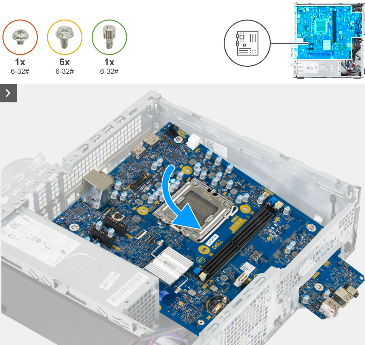
Figure 68. Installing the system board
