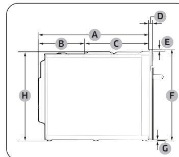
Oven (mm)
