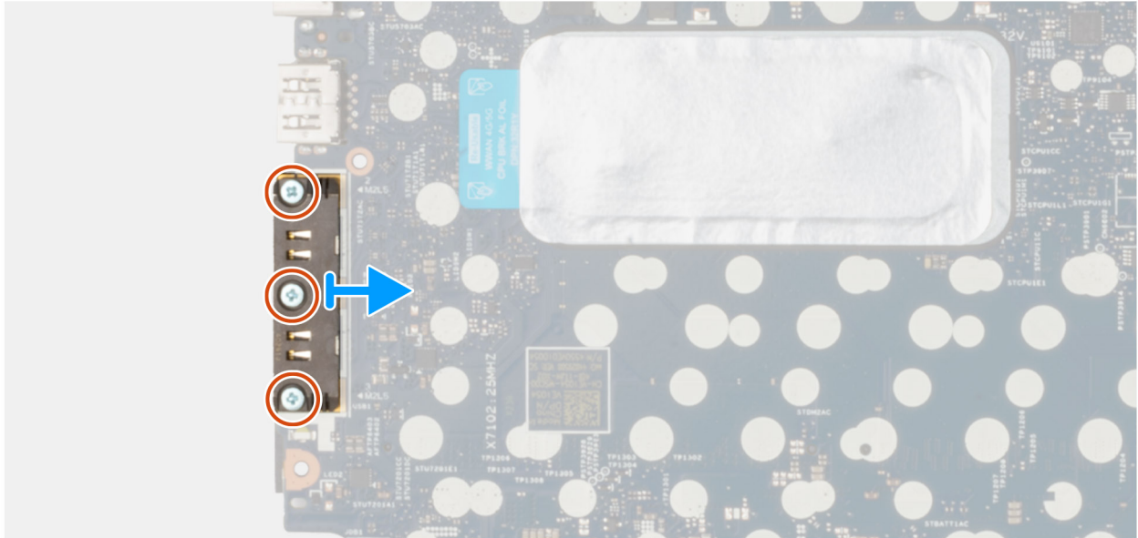
Figure 60. Removing the USB Type-C Connector Module
