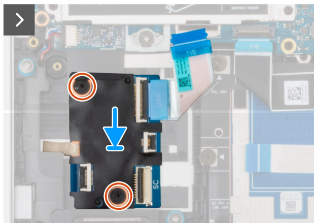
Figure 47. Installing the USH board
