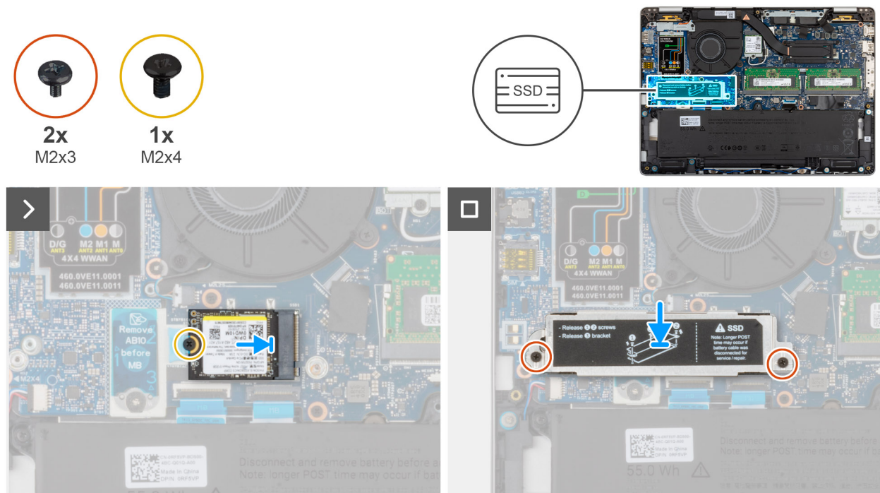
Figure 38. Installing the M.2 2230 SSD
