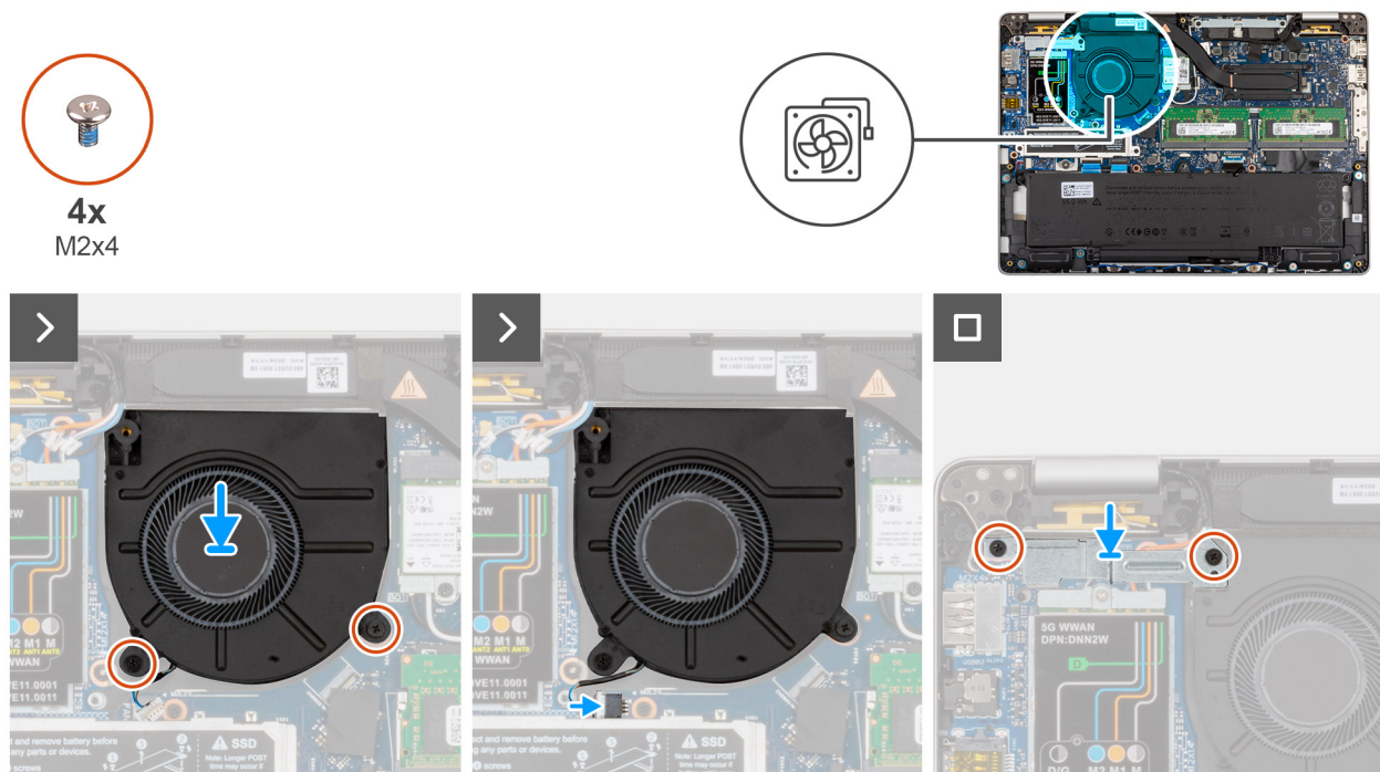
Figure 44. Installing the fan
