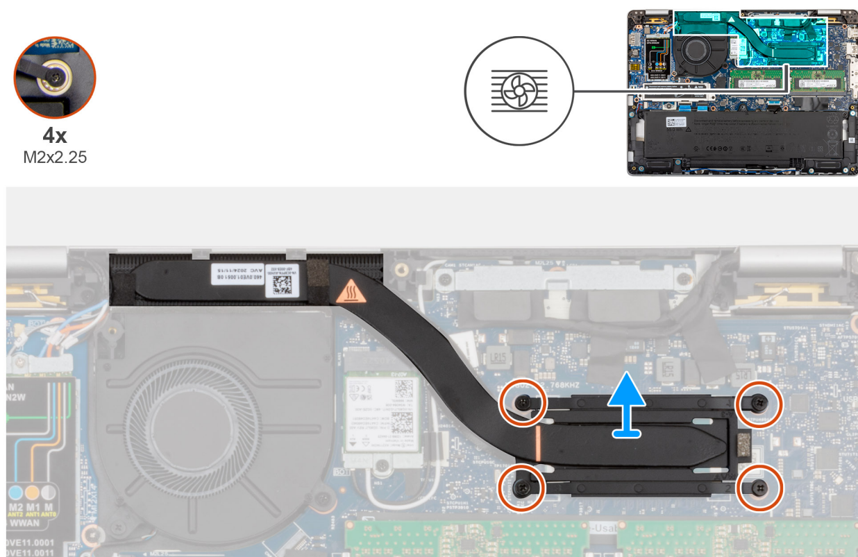
Figure 50. Removing the heat sink
