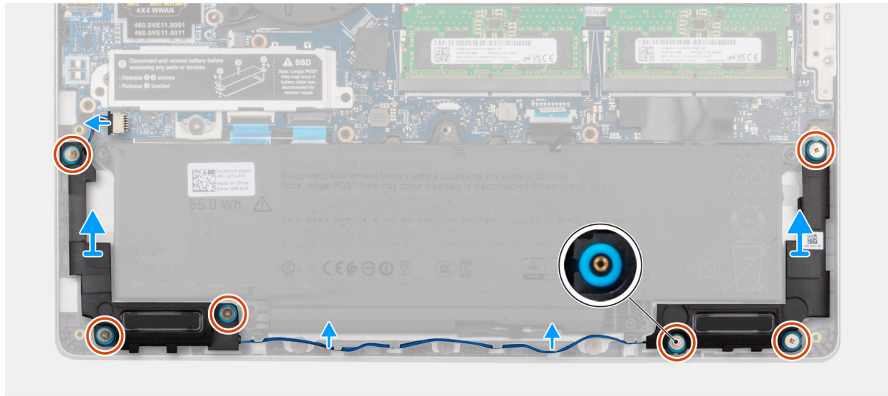
Figure 41. Removing the speakers
