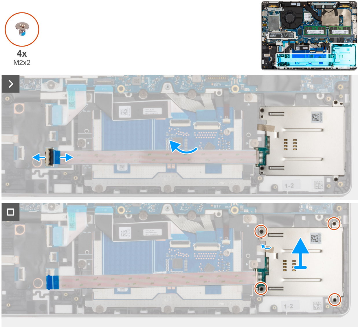
Figure 48. Removing the Smart card reader
