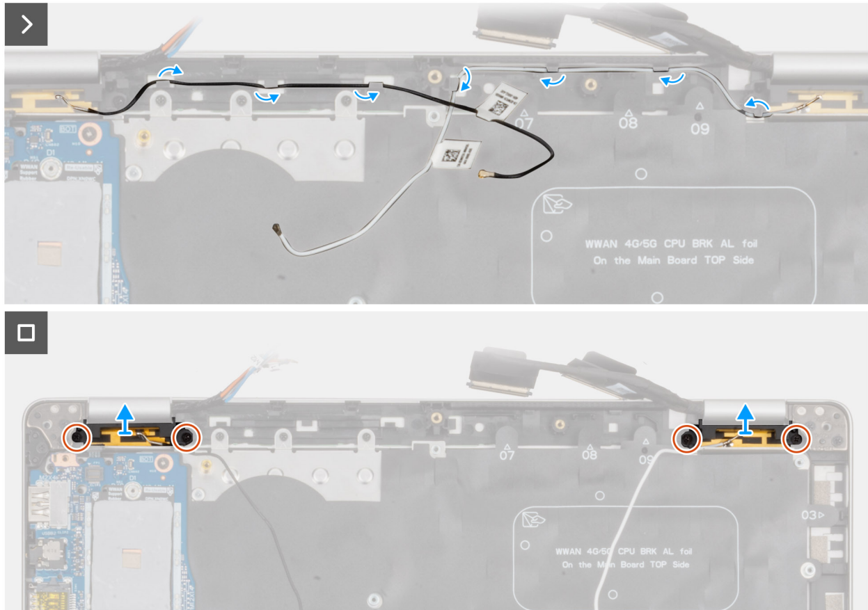
Figure 62. Removing the wireless antenna module
