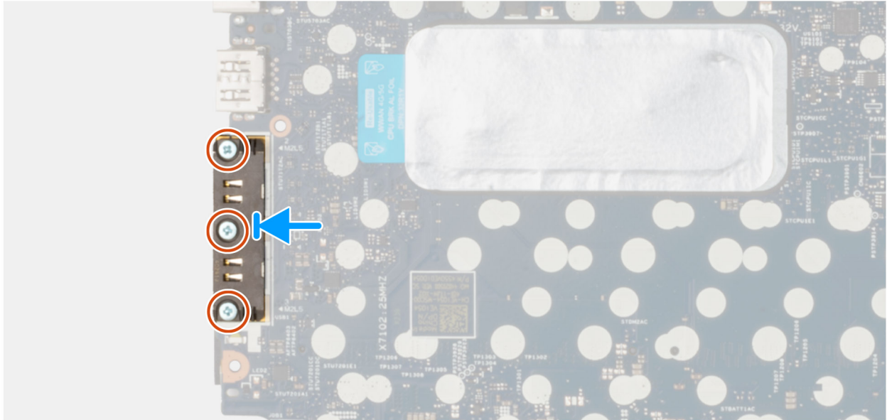
Figure 61. Installing the USB Type-C Connector Module
