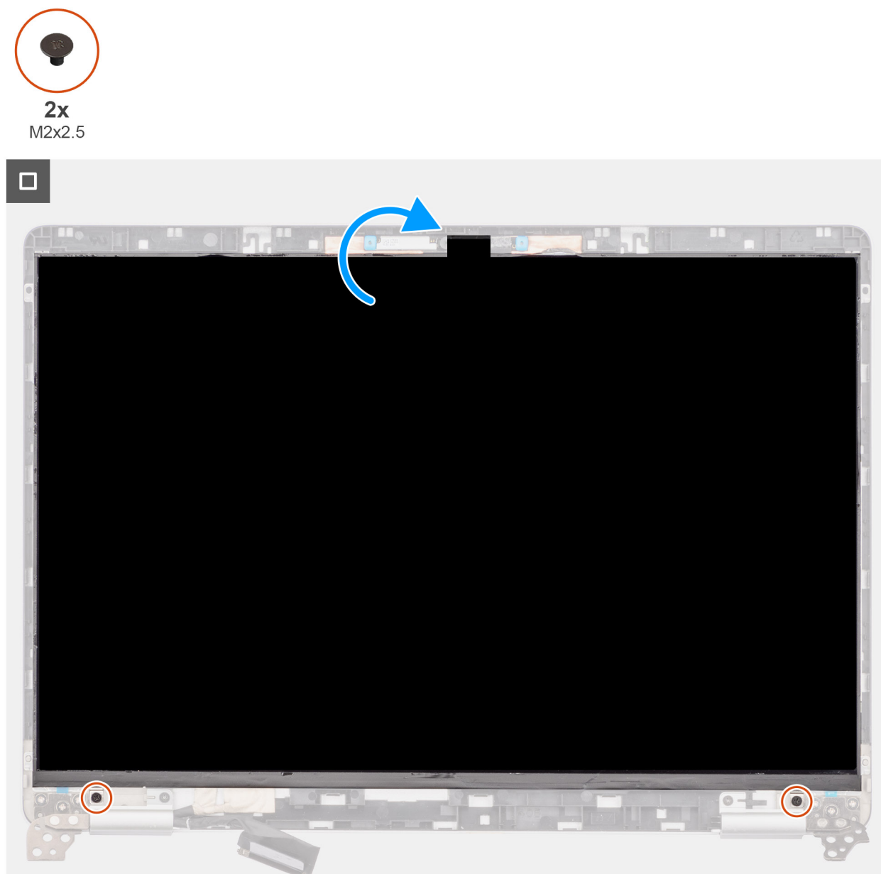
Figure 78. Installing the display panel
