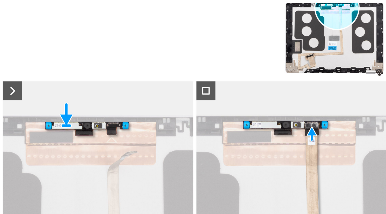
Figure 81. Installing the camera module
