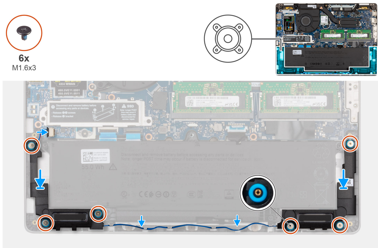
Figure 42. Installing the speakers
