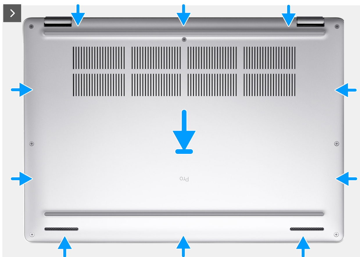
Figure 21. Installing the base cover
