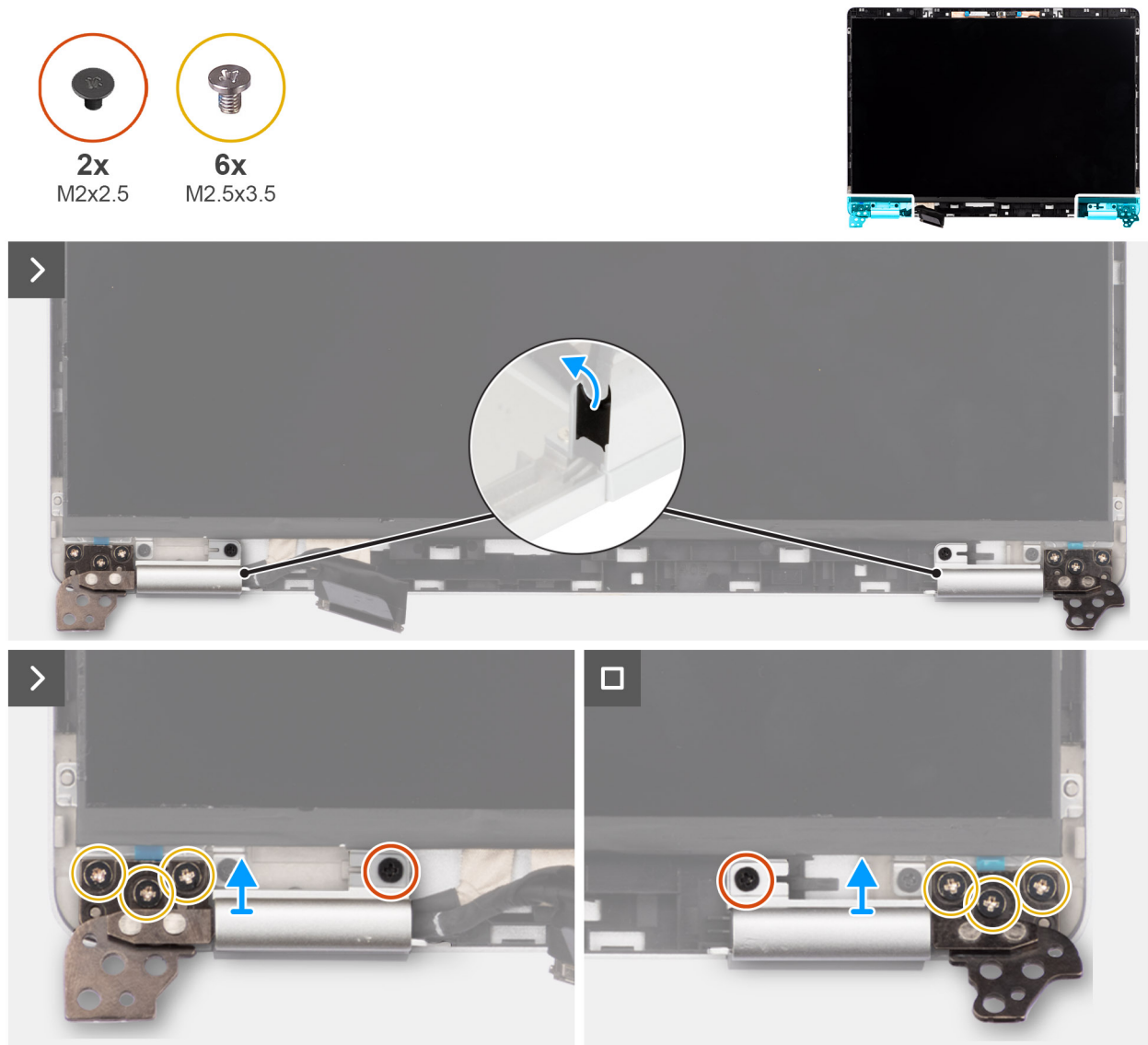
Figure 75. Removing the display hinges
