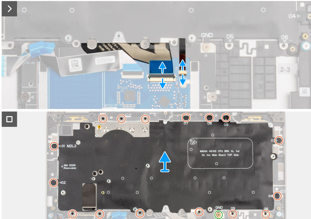
Figure 68. Removing the keyboard
