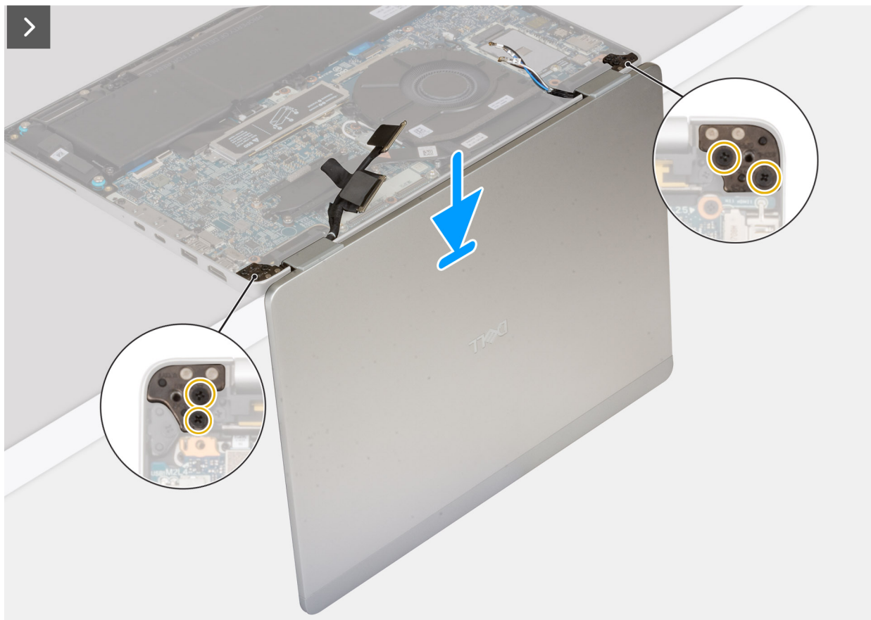
Figure 54. Installing the display assembly
