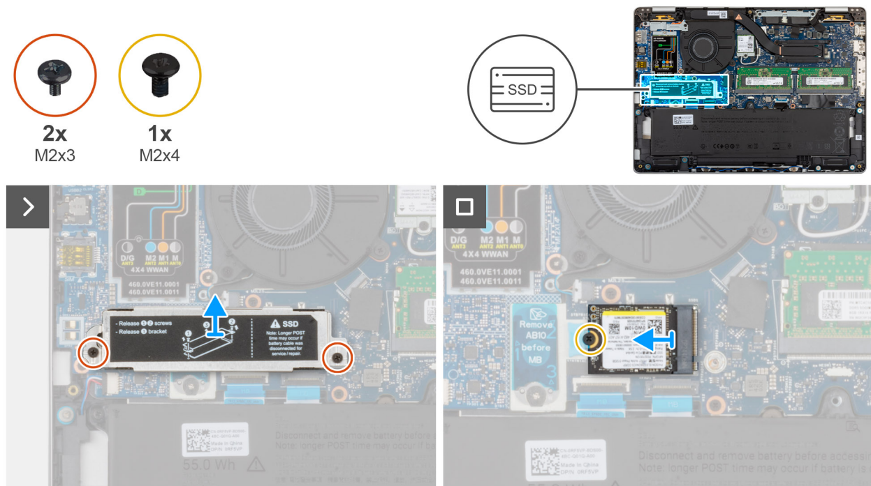
Figure 37. Removing the M.2 2230 SSD
