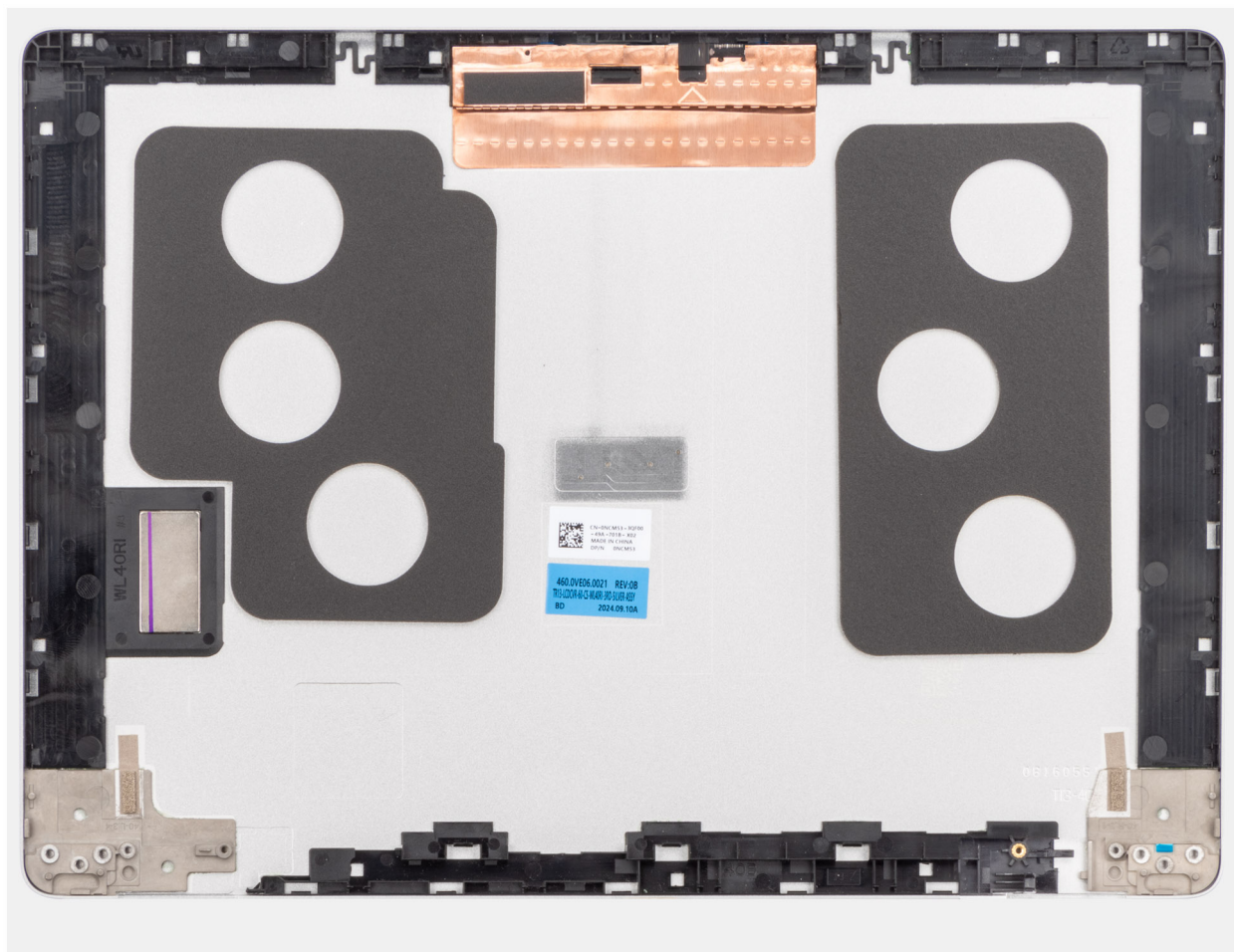
Figure 87. Installing the display back cover
