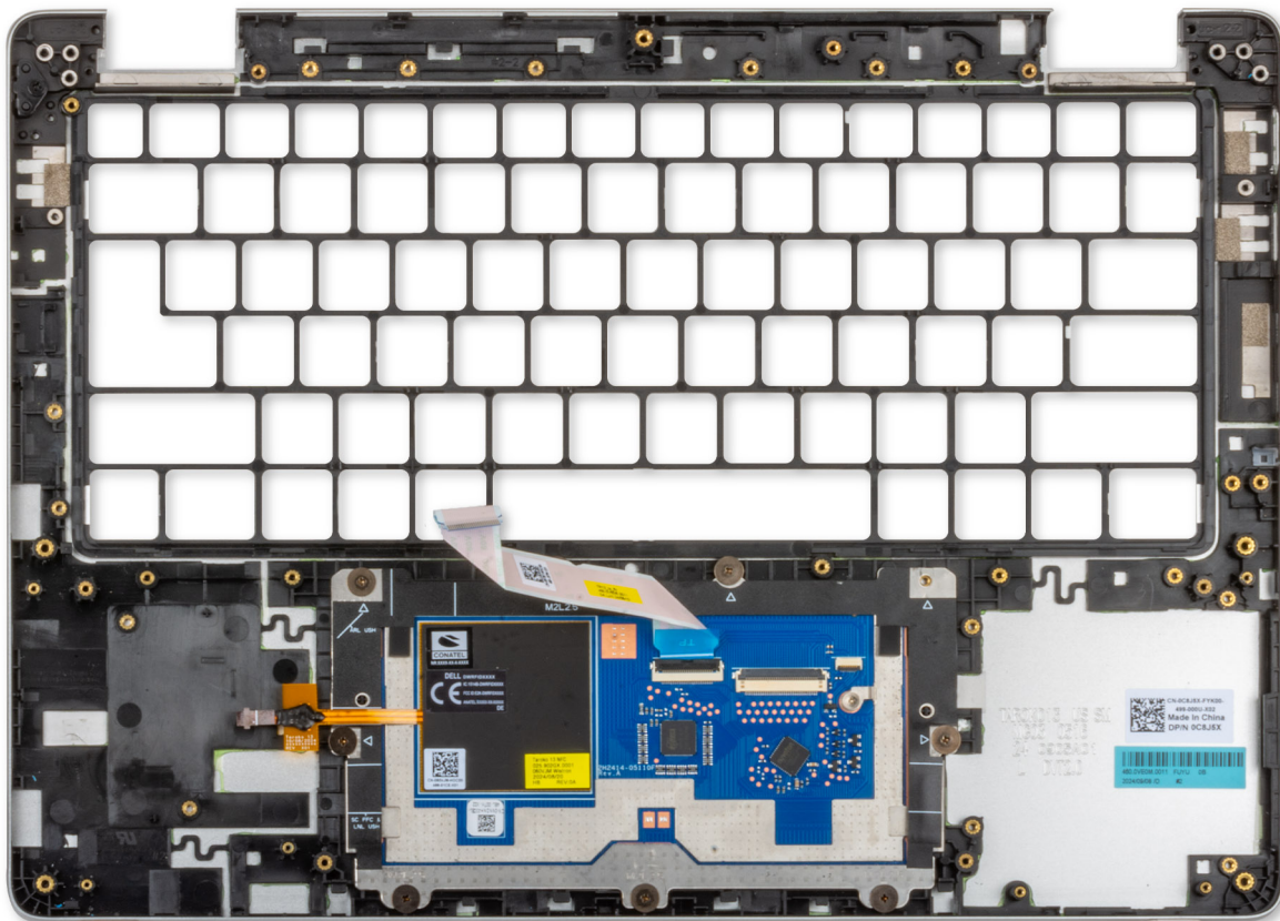
Figure 73. Installing the palm-rest assembly
