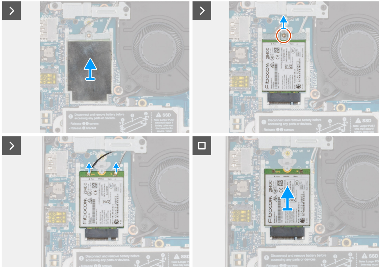
Figure 33. Removing the 4G WWAN card
