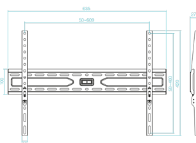
Dimensions (mm)
