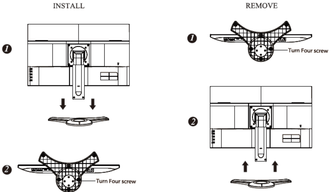
Figure.1. Installing and Removing the Base
