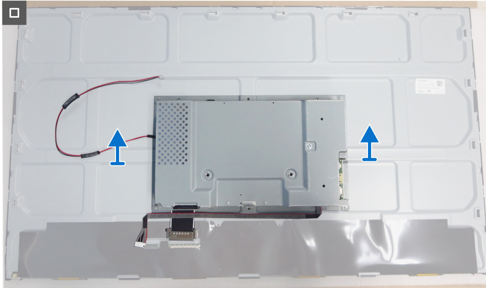
Figure 12. Removing the main chassis
