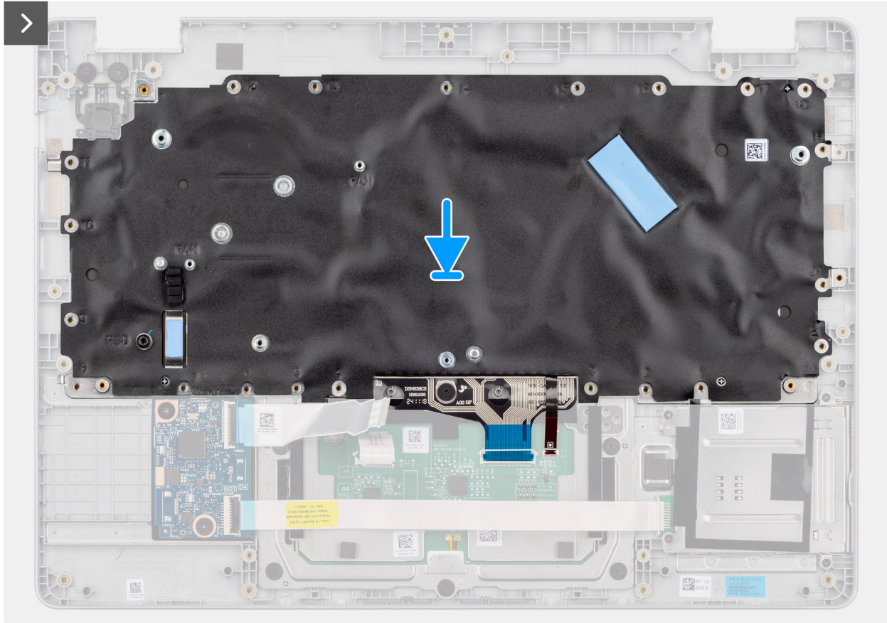
Figure 89. Installation du clavier
