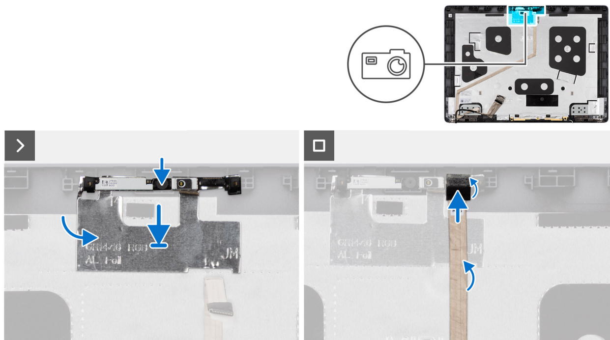
Figur 70. Installera kameran
