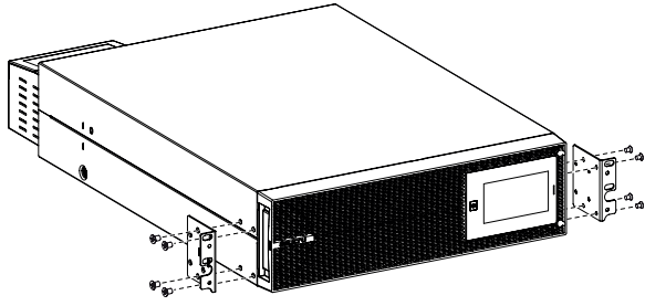
Fig. 20. Install the ears to the device.
