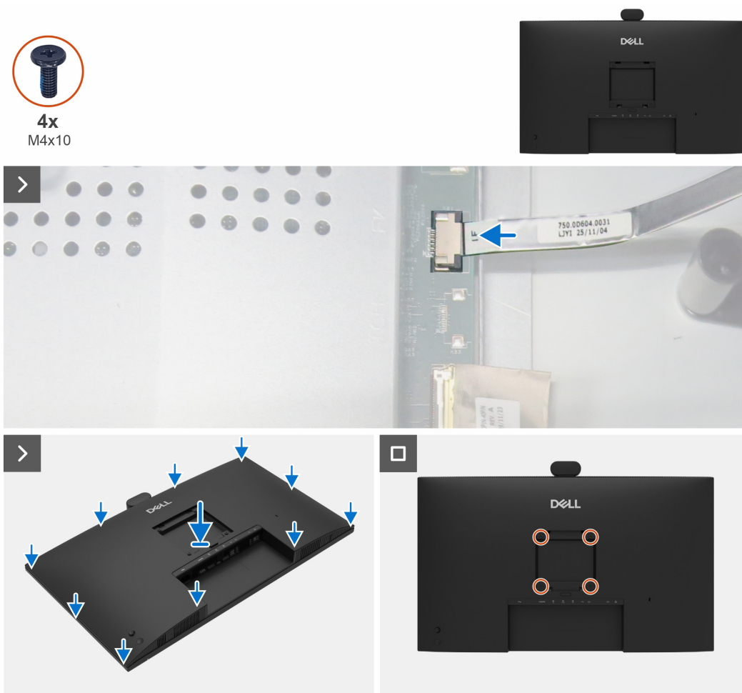
Figure 19. Installing the back cover
