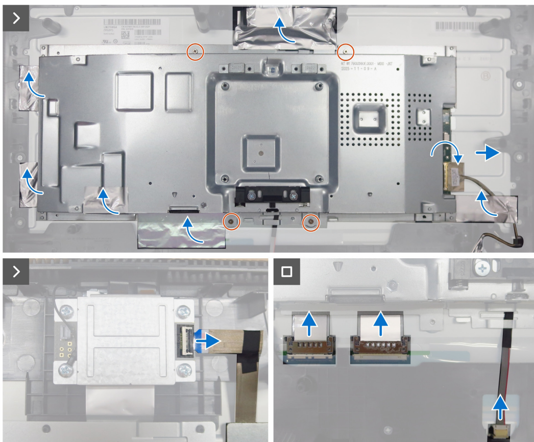
Figure 24. Removing the main chassis
