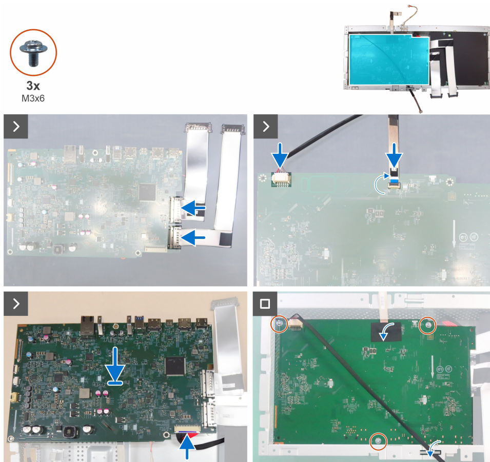
Figure 35. Installing the main board
