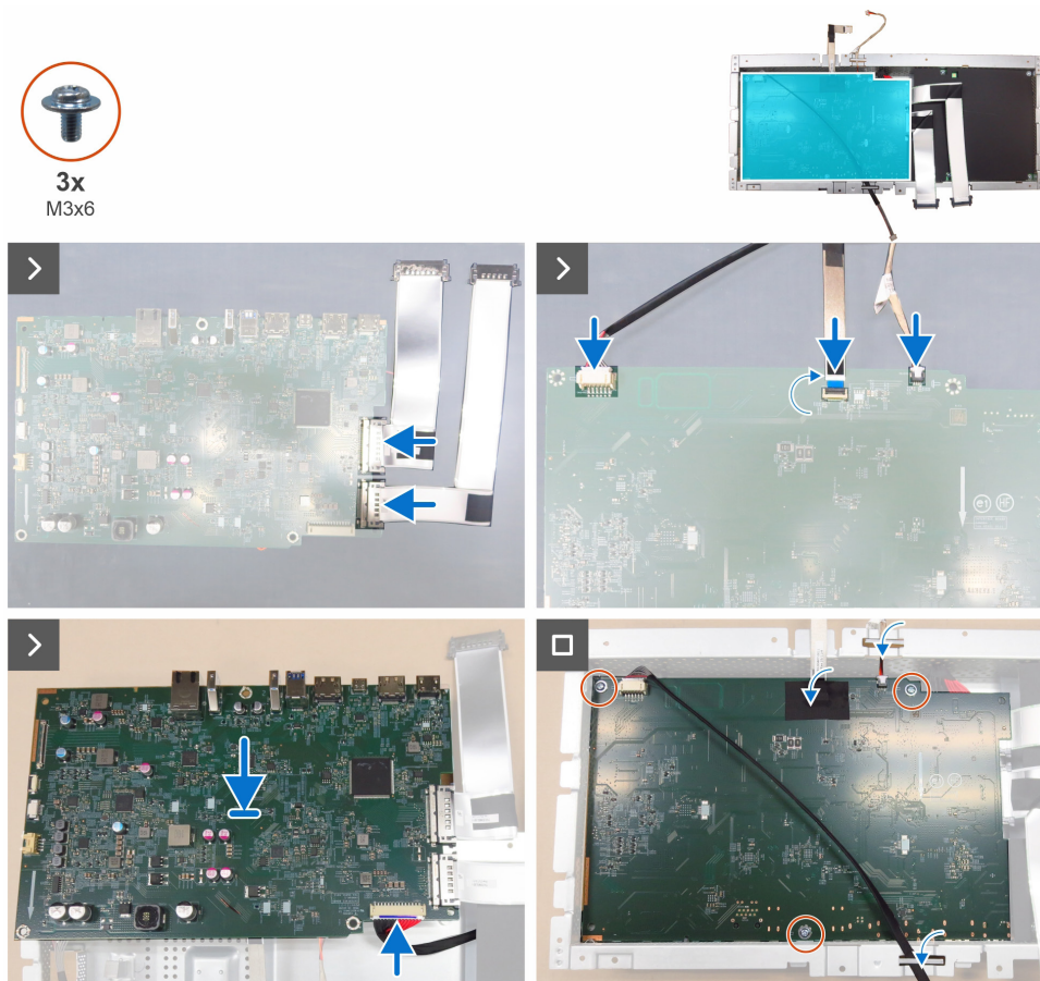
Figure 37. Installing the main board
