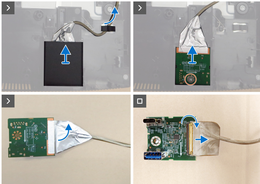
Figure 28. Removing the USB board
