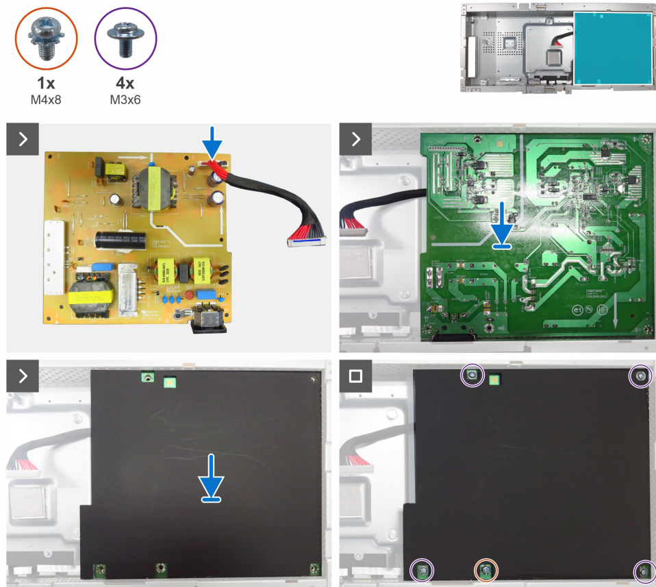
Figure 39. Installing the power board
