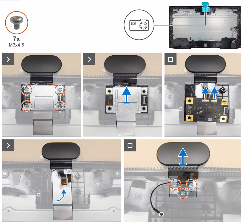
Figure 30. Removing the camera module
