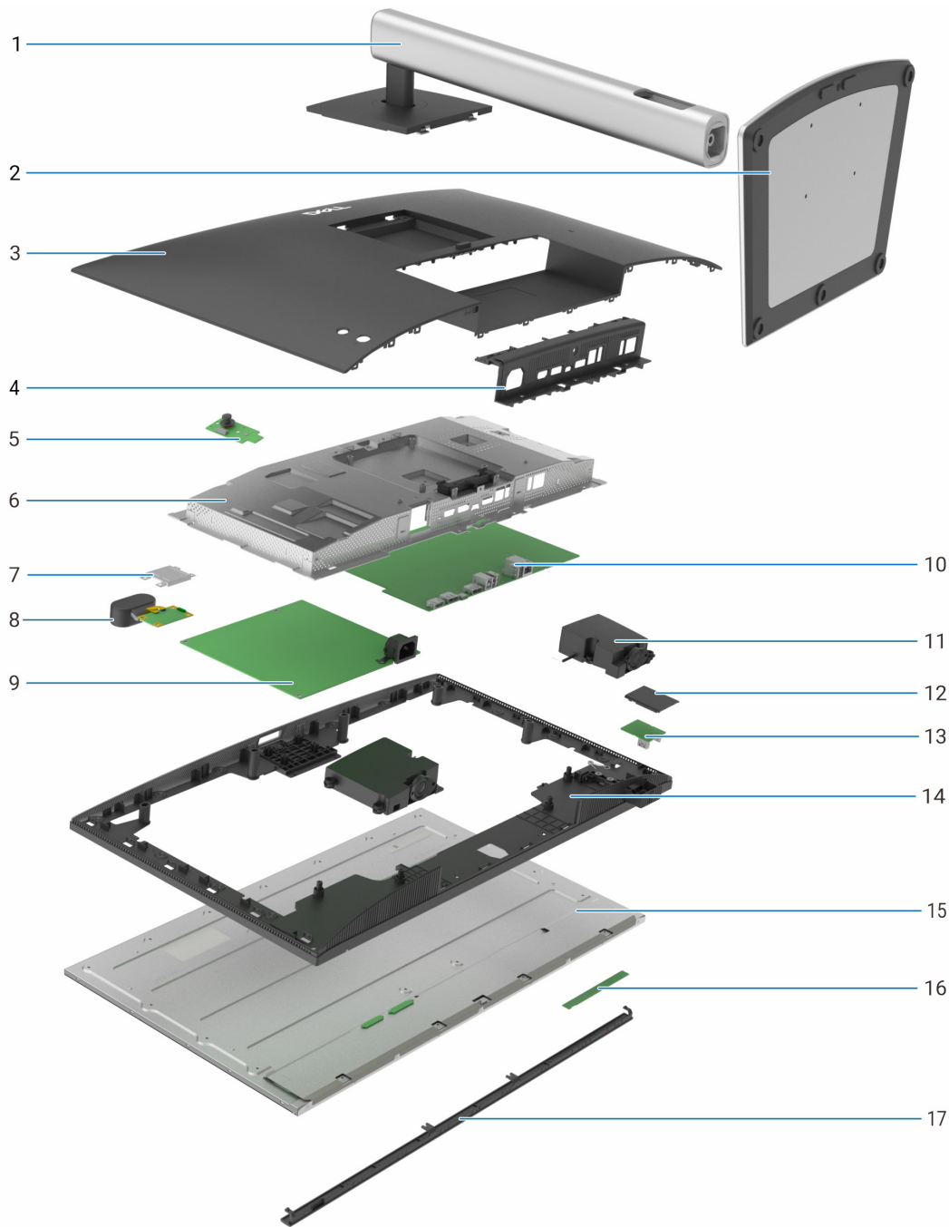
Figure 5. Major components of the P2426HEB/P2726DEB/P3426WEB monitor
