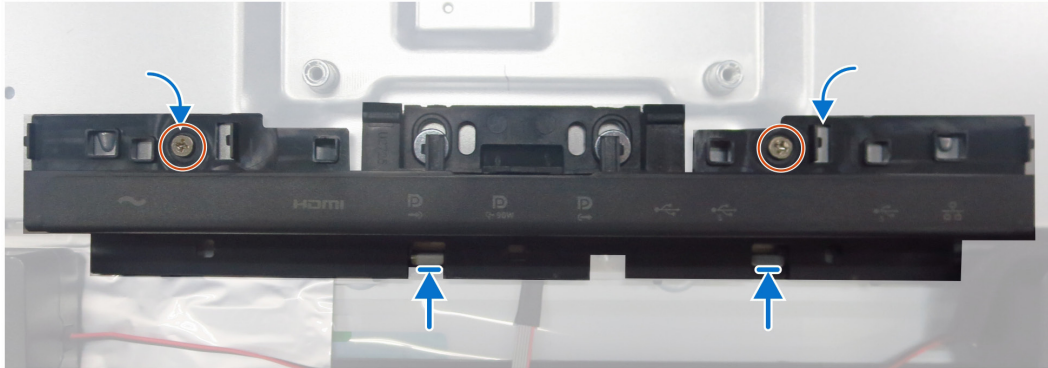
Figure 23. Installing the I/O cover
