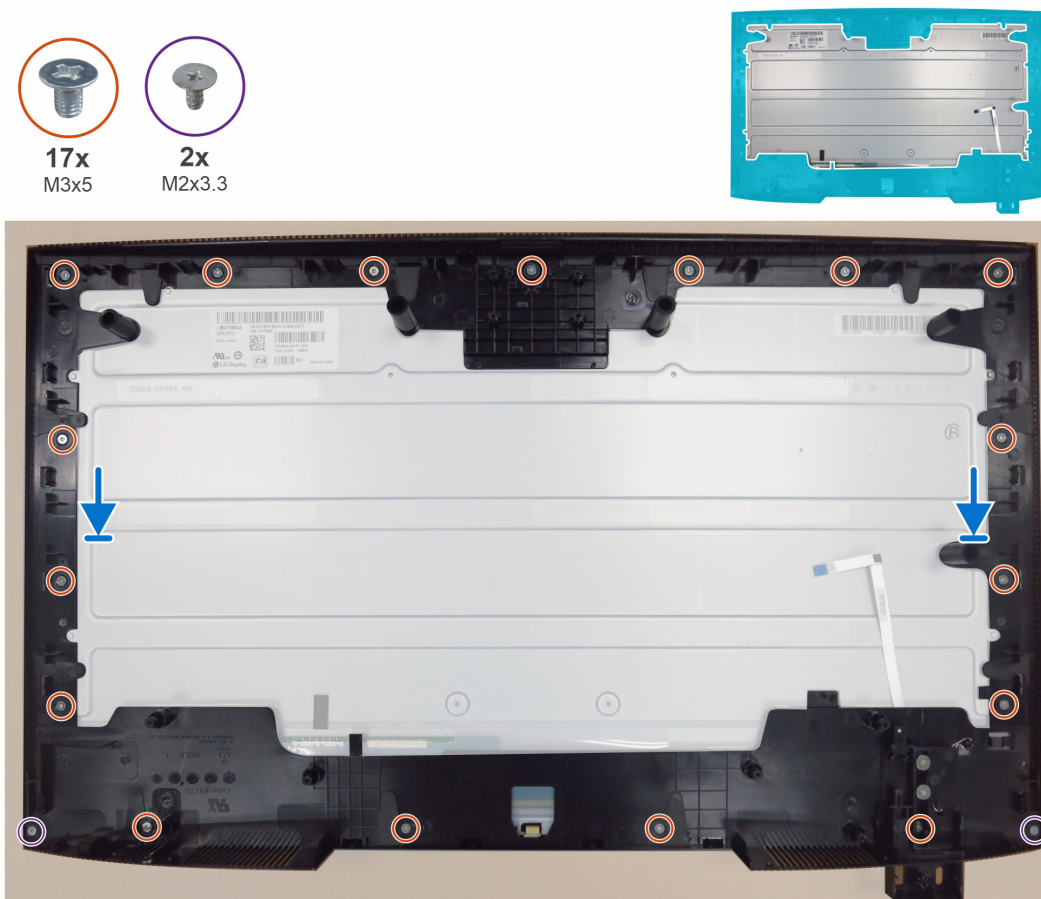
Figure 33. Installing the middle frame
