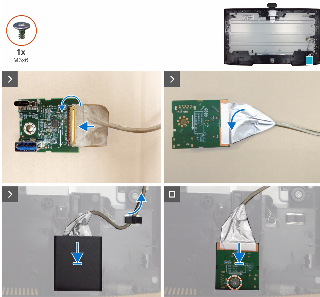
Figure 29. Installing the USB board
