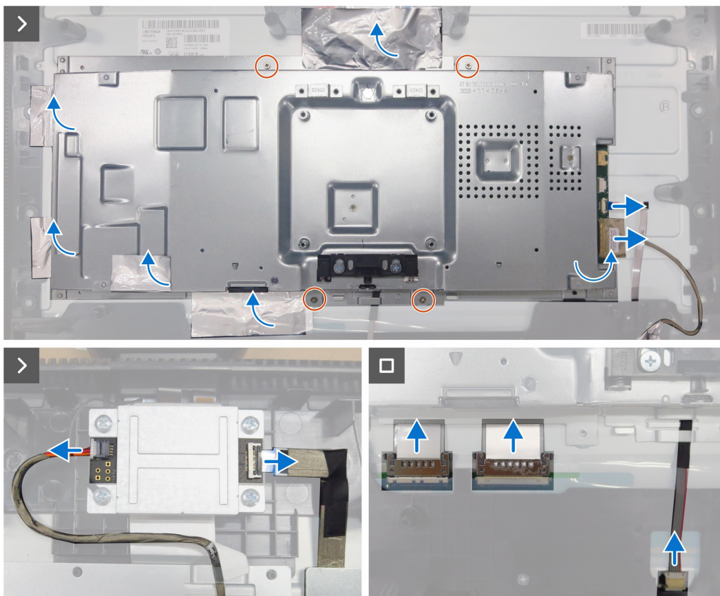
Figure 26. Removing the main chassis
