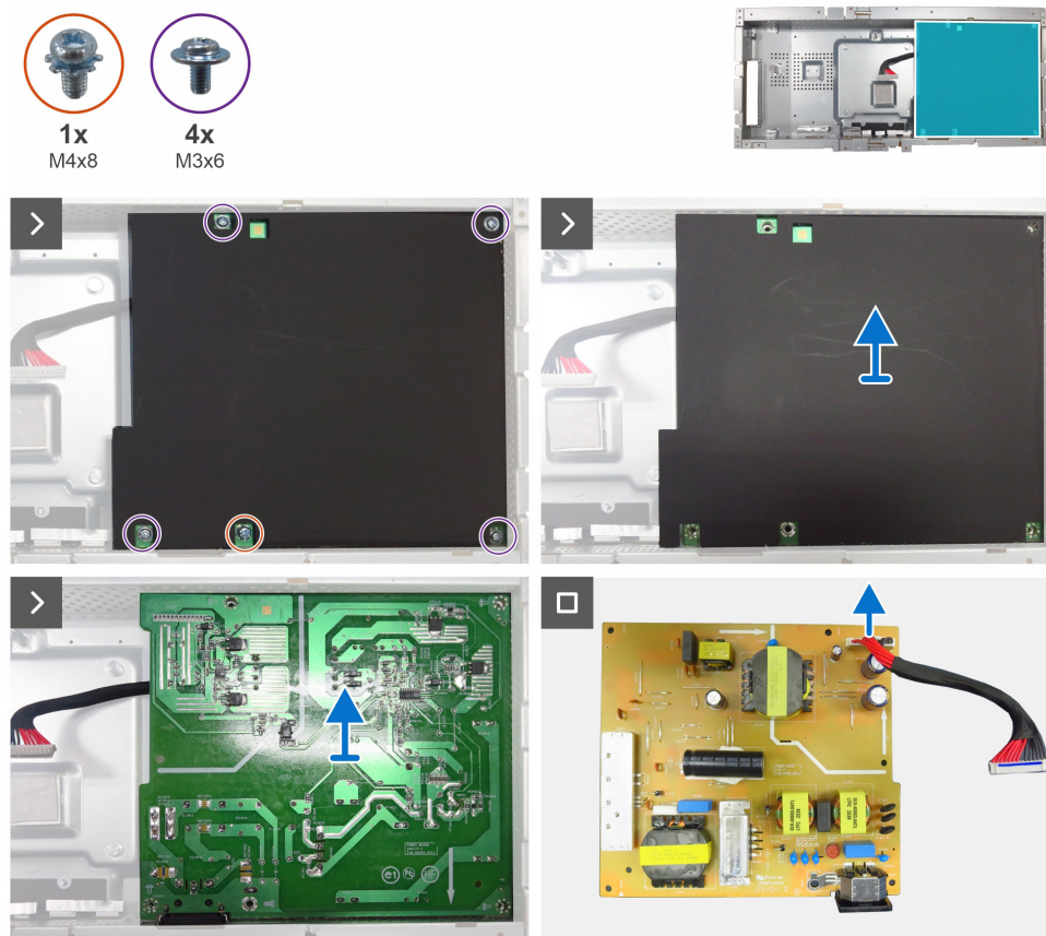
Figure 38. Removing the power board
