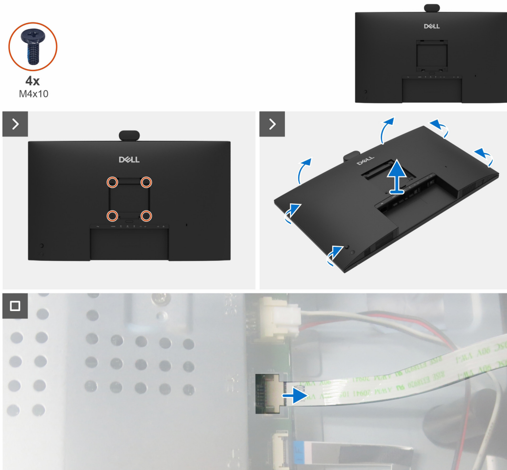
Figure 18. Removing the back cover
