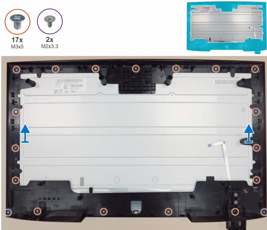
Figure 32. Removing the middle frame
