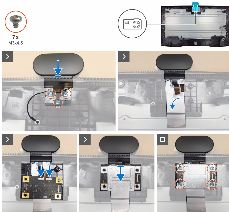
Figure 31. Installing the camera module
