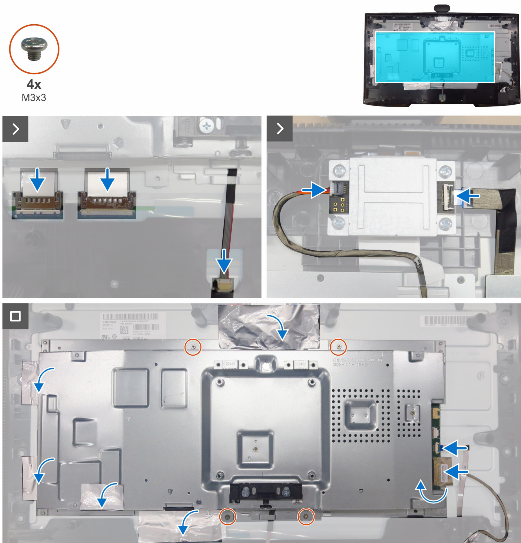
Figure 27. Installing the main chassis
