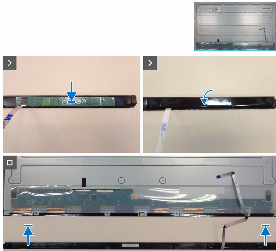
Figure 35. Installing the front trim and the touch board
