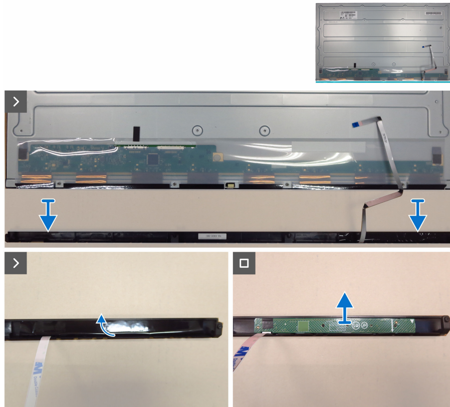
Figure 34. Removing the front trim and the touch board
