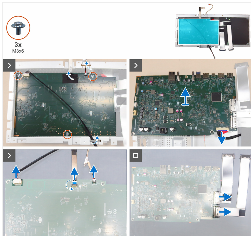
Figure 36. Removing the main board
