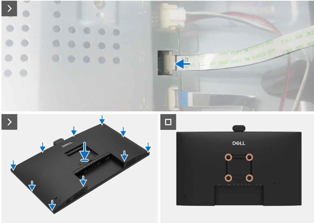
Figure 19. Installing the back cover
