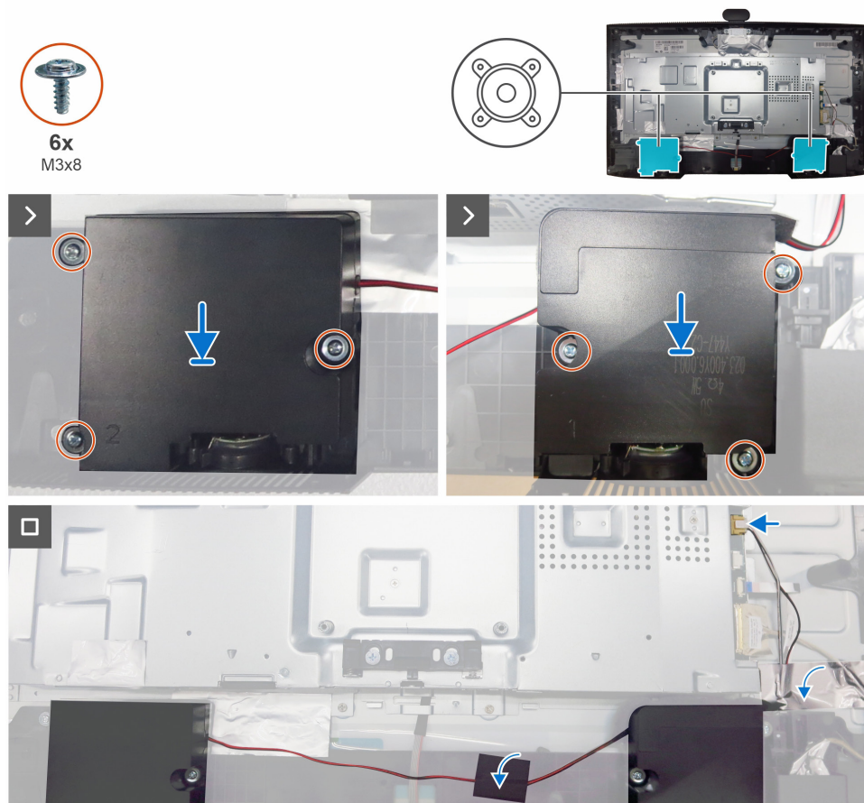
Figure 25. Installing the speakers
