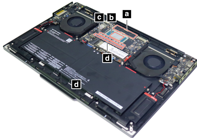
Figure 2. Areas on the system board where thermal interface materials are applied
