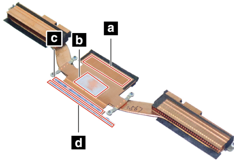
Figure 1. Type, quantity, and areas of thermal interface materials application on the heat sink
