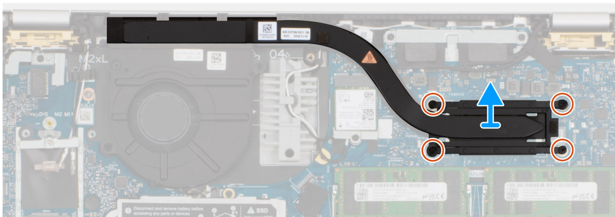
4x M2x2.25
