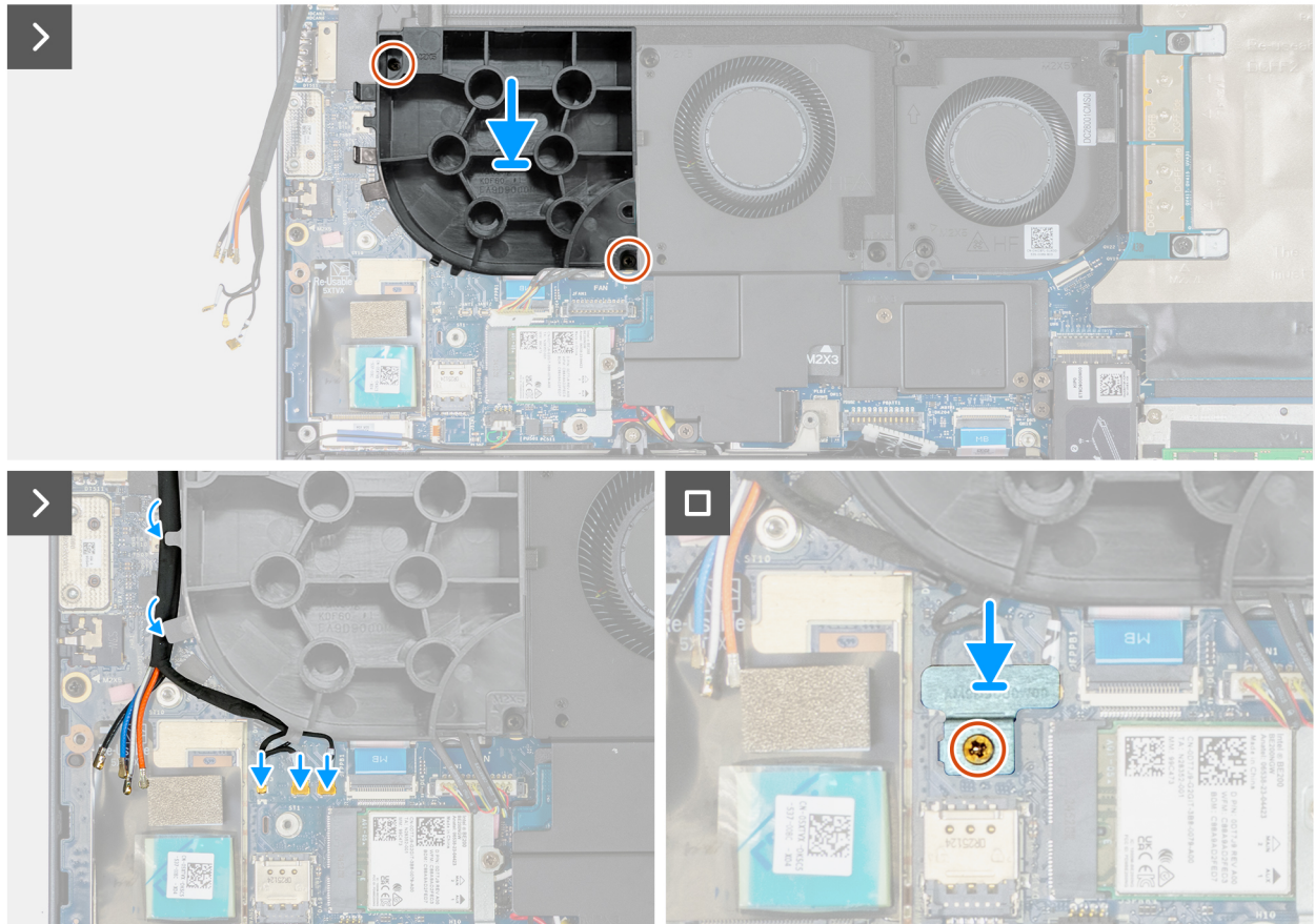
Figure 58. Installation du ventilateur factice
