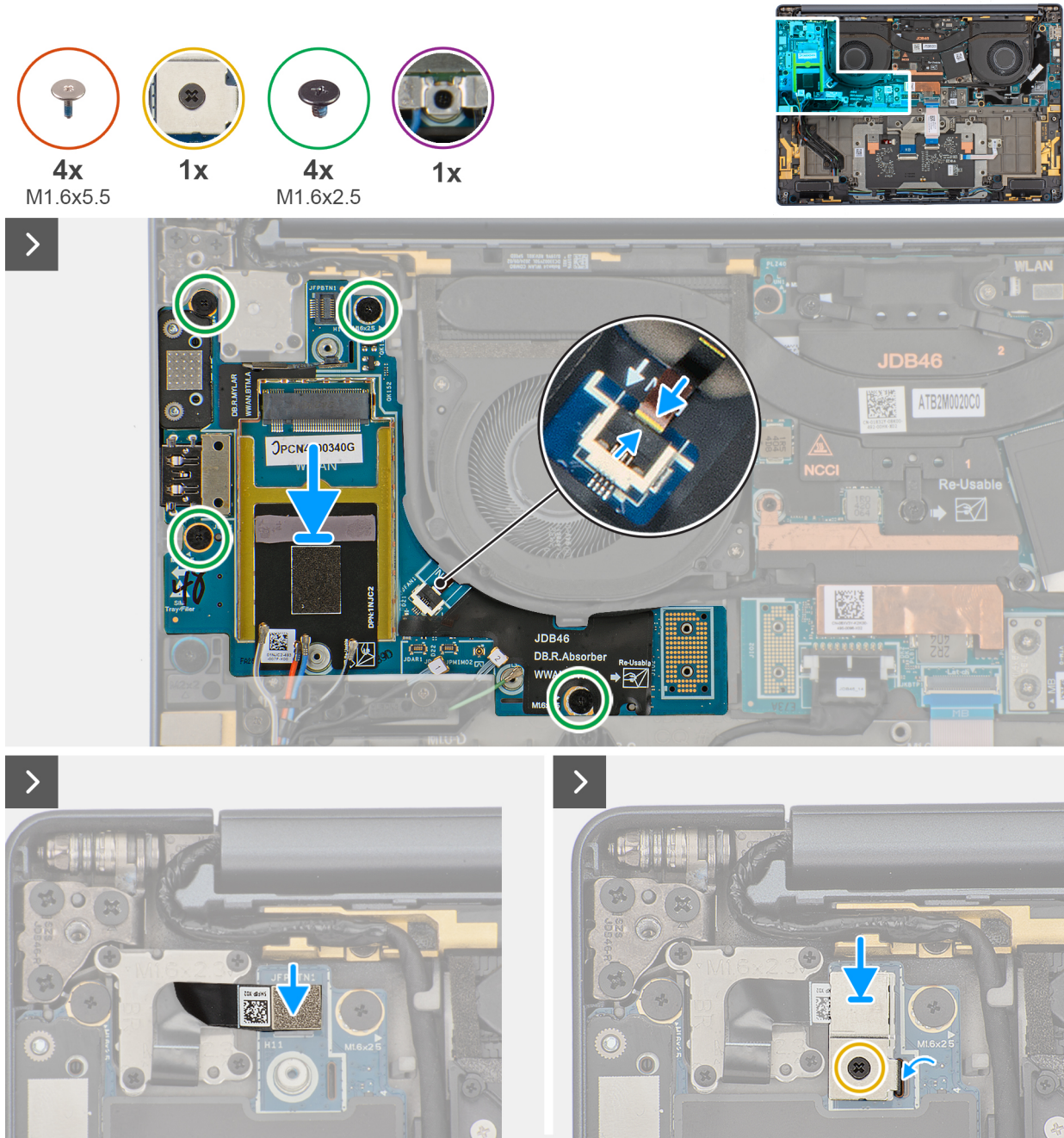
Figure 53. Installation des vis
