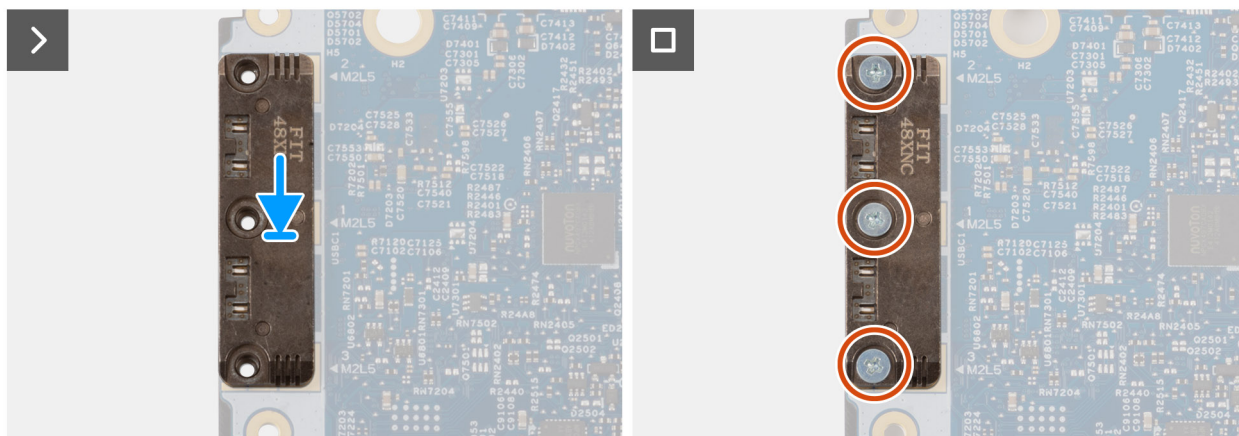
Figure 49. Installation du module USB-C
