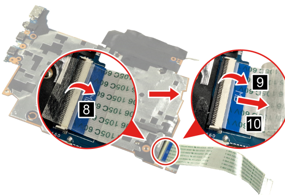
Figure 20. Disconnect the I/O board cable from the system board
